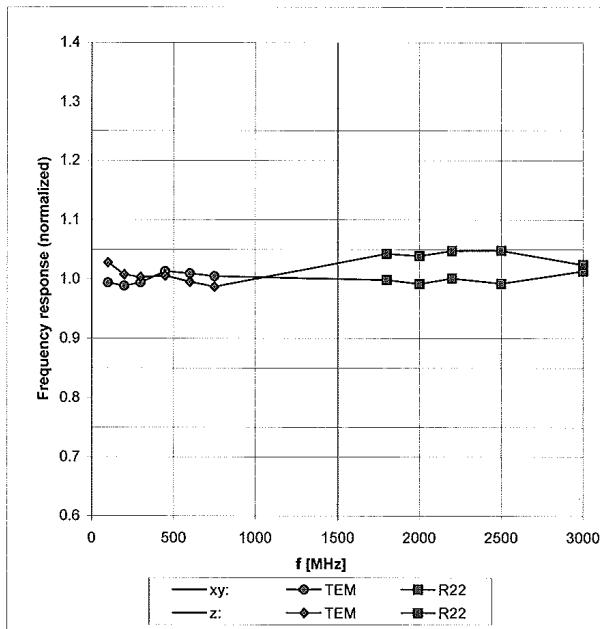
Uncertainty of Frequency Response of H-field: ± 6.3% (k=2)
