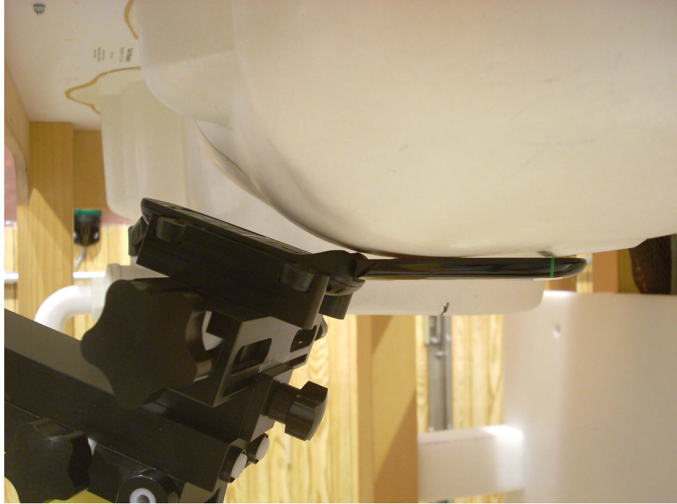
Figure 18-5 SAR Test Setup Photo 5
