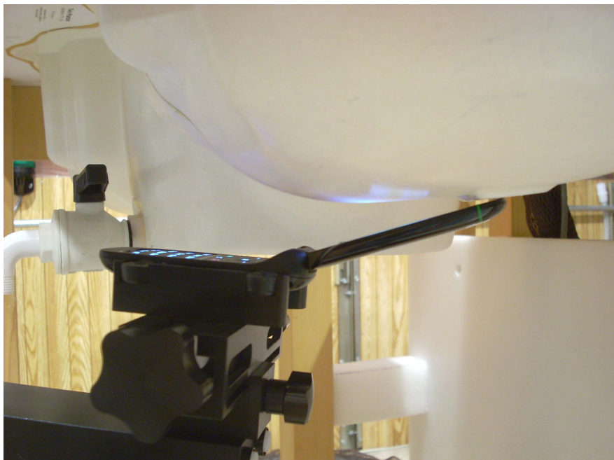
Figure 18-2 SAR Test Setup Photo 2
