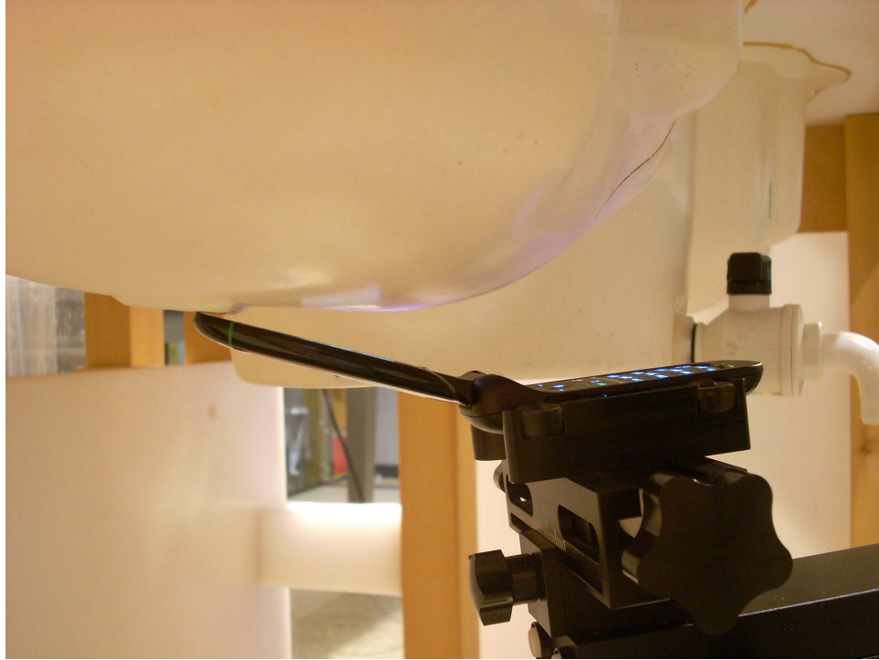
Figure 18-3 SAR Test Setup Photo 3
