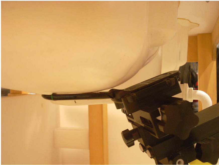
Figure 18-1 SAR Test Setup Photo 1
