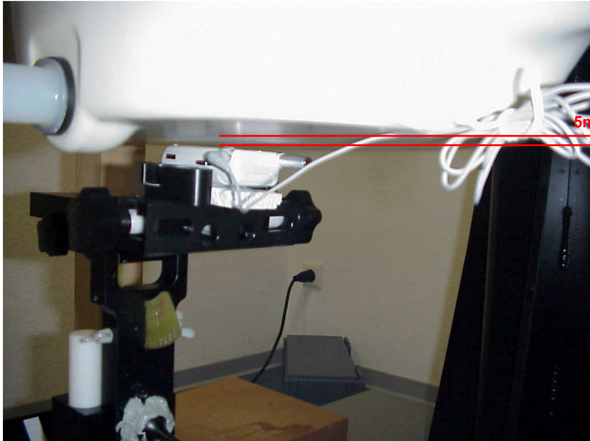
Photo 6 : test position at the flat phantom, rear side, test with headset
