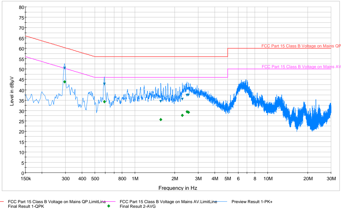
Plot 6-86. Line Conducted Plot with 802.11a UNII Band 1 (N)
