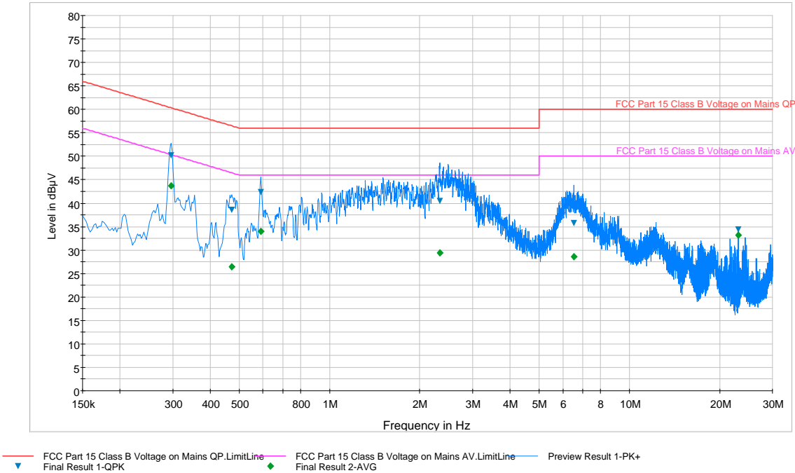
Plot 6-89. Line Conducted Plot with 802.11a UNII Band 3 (L1)
