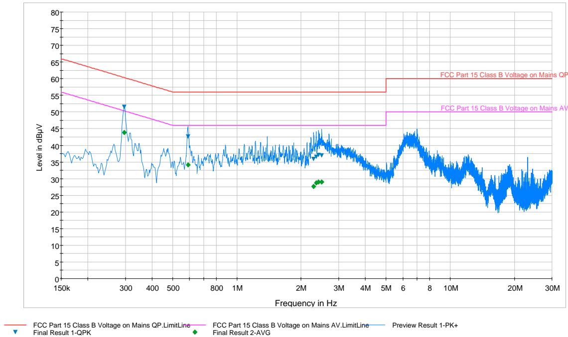
Plot 6-88. Line Conducted Plot with 802.11a UNII Band 2 (N)
