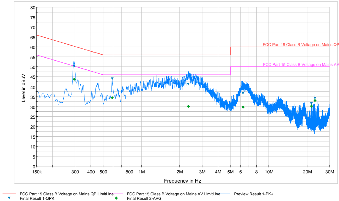
Plot 6-85. Line Conducted Plot with 802.11a UNII Band 1 (L1)
