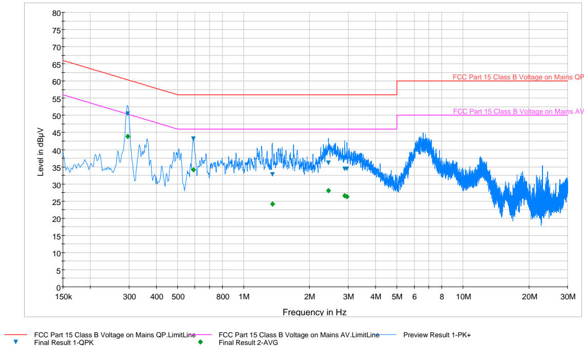
Plot 6-90. Line Conducted Plot with 802.11a UNII Band 3 (N)
