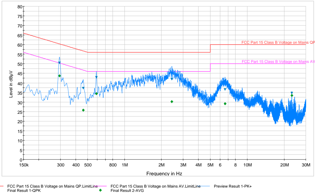
Plot 6-87. Line Conducted Plot with 802.11a UNII Band 2 (L1)
