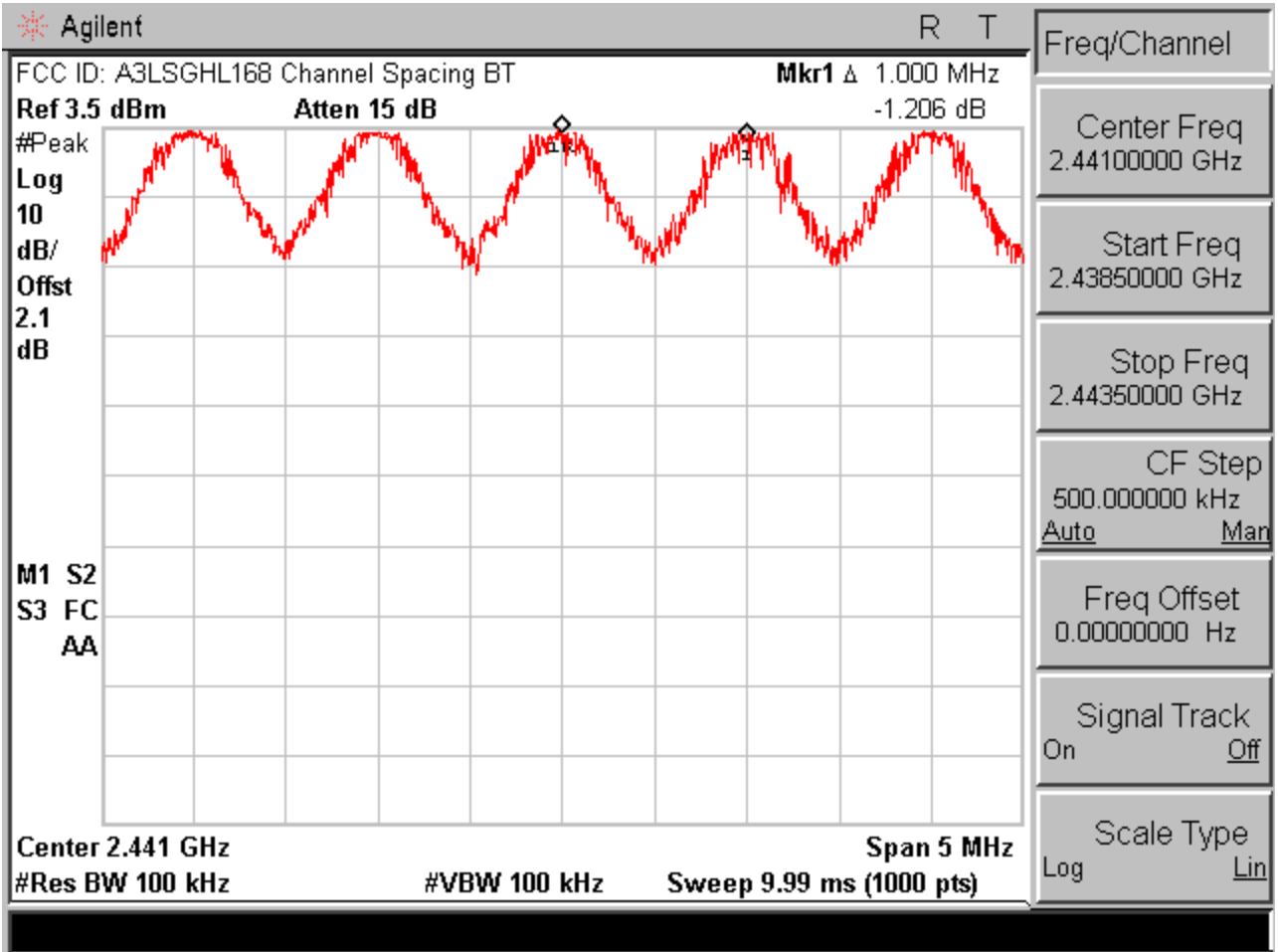
Plot 6-8. Channel Spacing Plot (Bluetooth)
