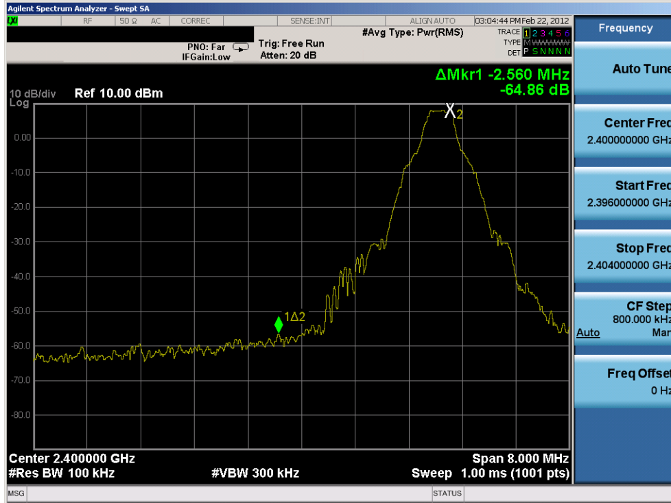
Plot 6-1. Band Edge Plot (Bluetooth with Hopping Disabled, 1Mbps – Ch. 0)
