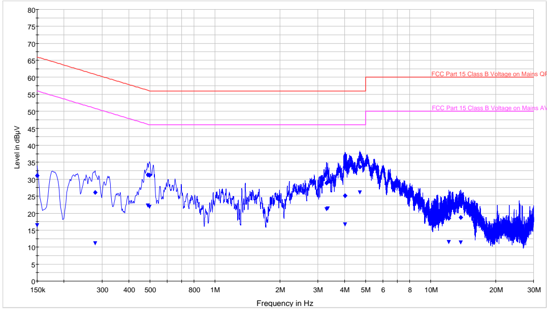
Plot 6-5. Line Conducted Plot with Bluetooth – Line 1
