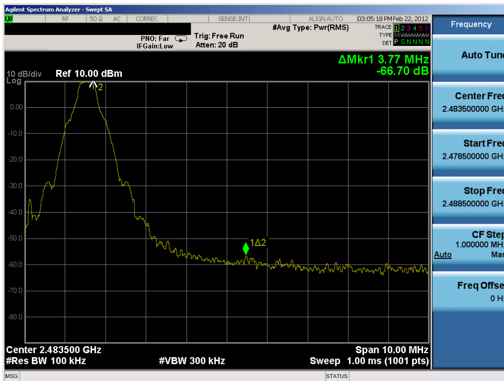
Plot 6-2. Band Edge Plot (Bluetooth with Hopping Disabled, 1Mbps – Ch. 78)
