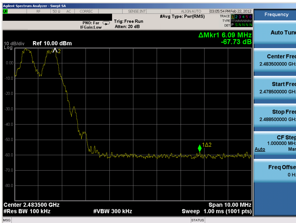
Plot 6-4. Band Edge Plot (Bluetooth with Hopping Enabled, 1Mbps – Ch. 78)
