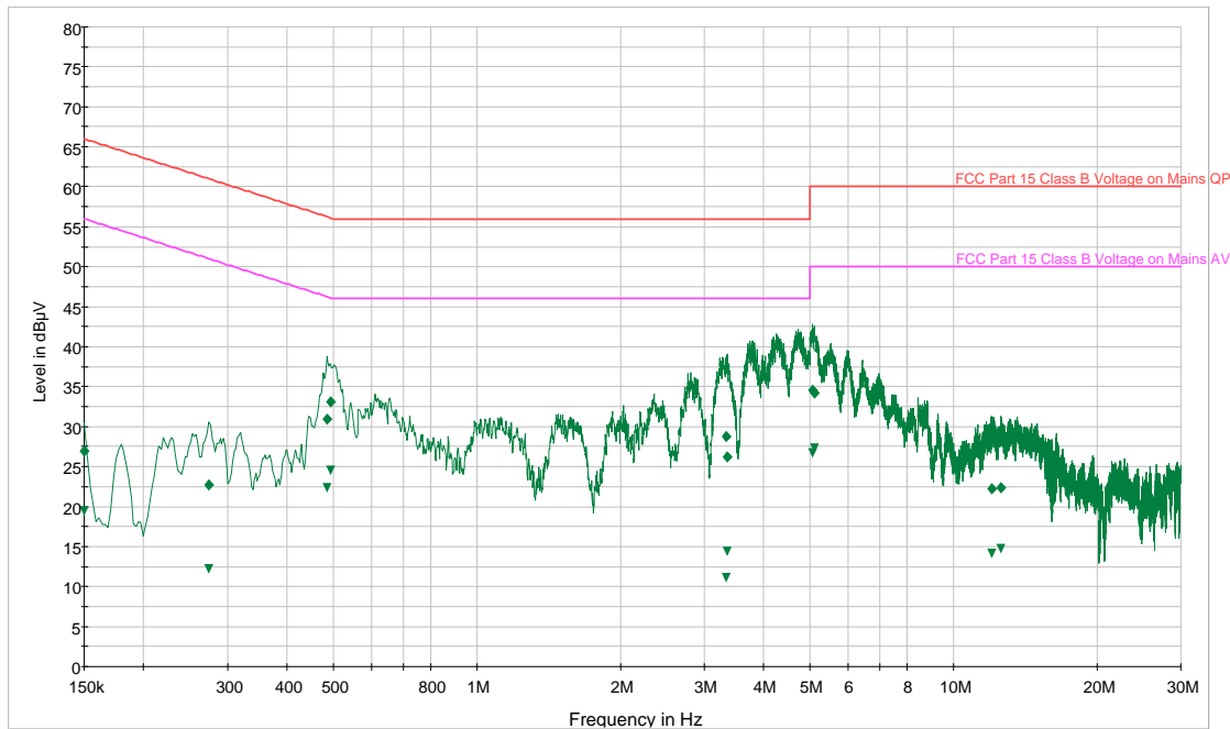
Plot 6-5. Line Conducted Plot with Bluetooth – Line 1
