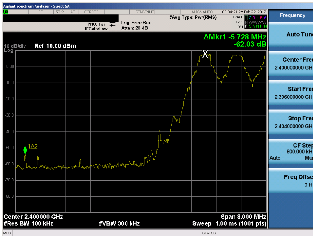
Plot 6-3. Band Edge Plot (Bluetooth with Hopping Enabled, 1Mbps – Ch. 0)
