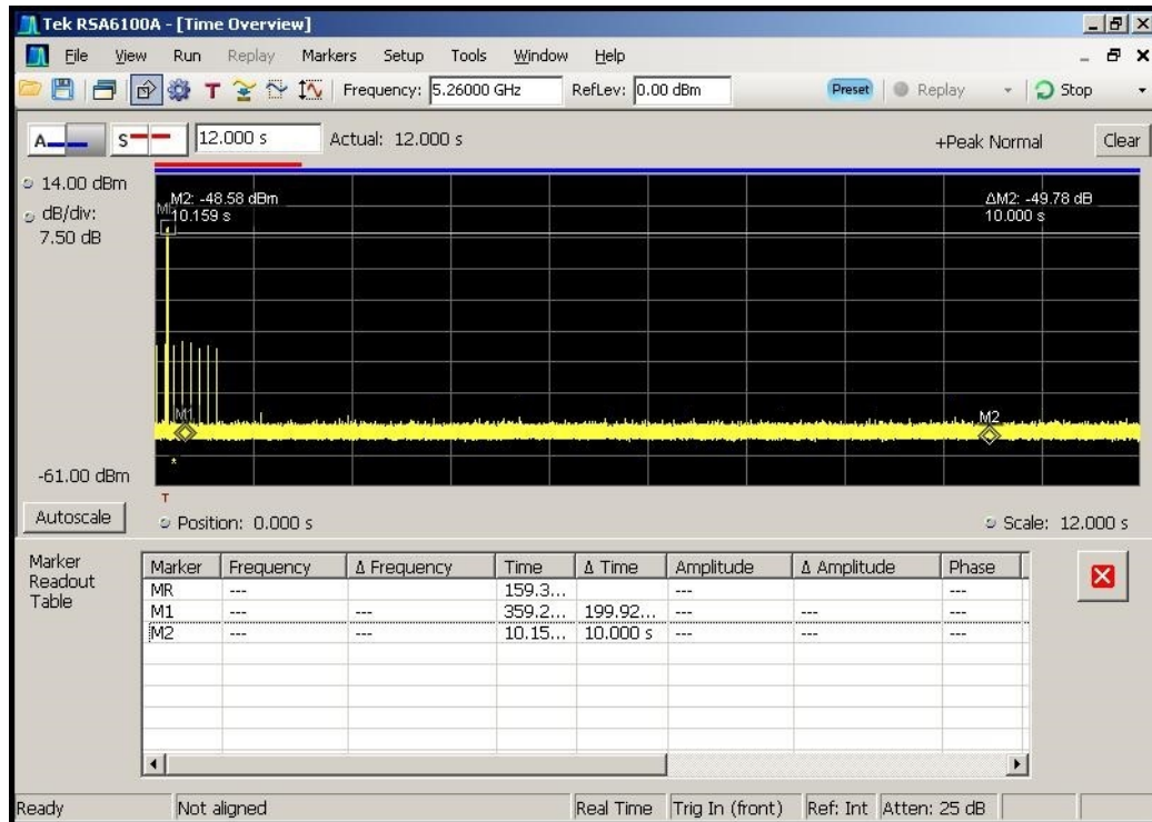
Figure 5-5. Channel Move Time (< 10sec)
