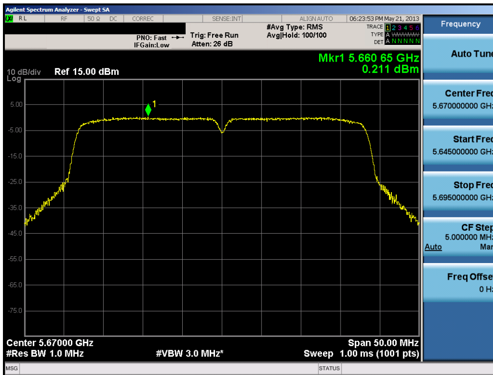
Plot 6-57. Peak Power Spectral Density Plot (40MHz BW 802.11n (UNII Band 3) – Ch. 134)
