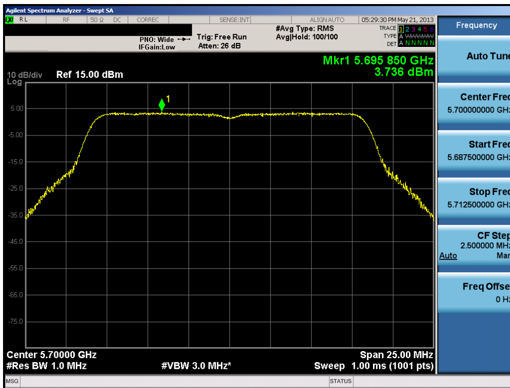
Plot 6-51. Peak Power Spectral Density Plot (802.11a (UNII Band 3) – Ch. 140)
