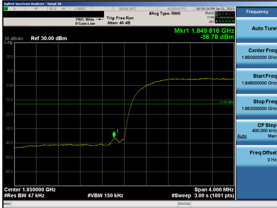
Plot 7-45. Band Edge Plot (PCS WCDMA Mode – Ch. 9262)
