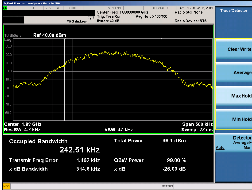
Plot 7-23. Occupied Bandwidth Plot (PCS GSM Mode – Ch. 661)
