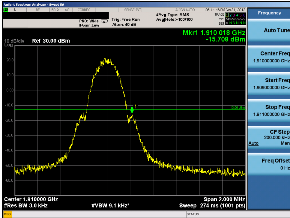
Plot 7-28. Band Edge Plot (PCS GSM Mode – Ch. 810)
