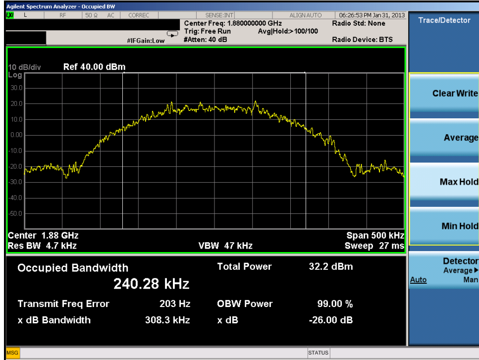
Plot 7-29. Occupied Bandwidth Plot (EDGE1900 Mode – Ch. 661)
