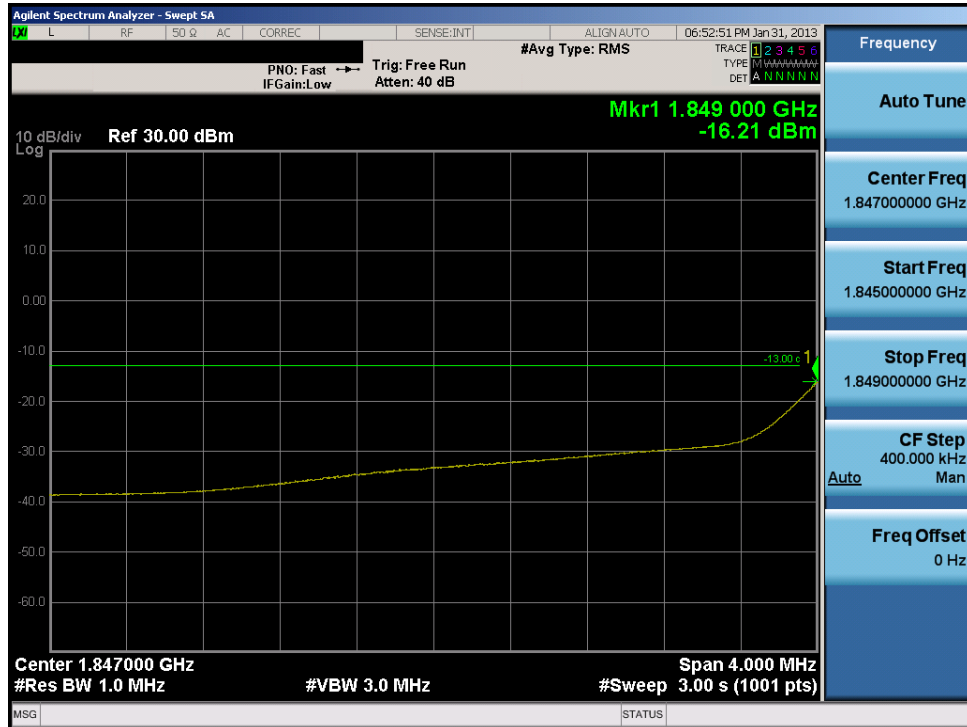
Plot 7-46. 4MHz Span Plot (PCS WCDMA Mode – Ch. 9262)
