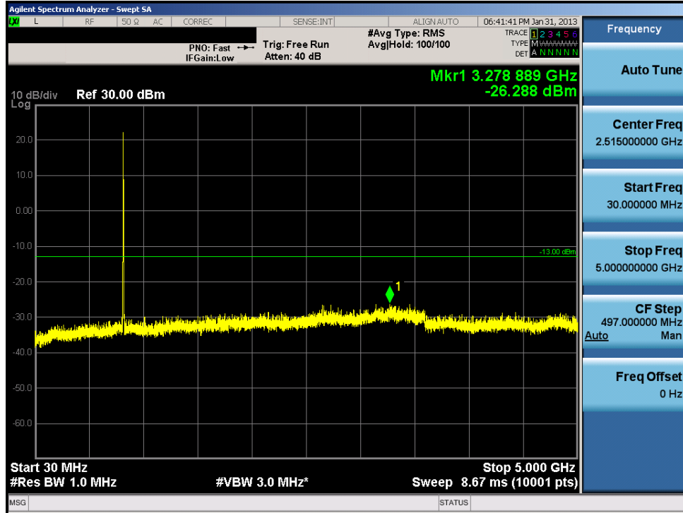
Plot 7-35. Conducted Spurious Plot (Cellular WCDMA Mode – Ch. 4183)
