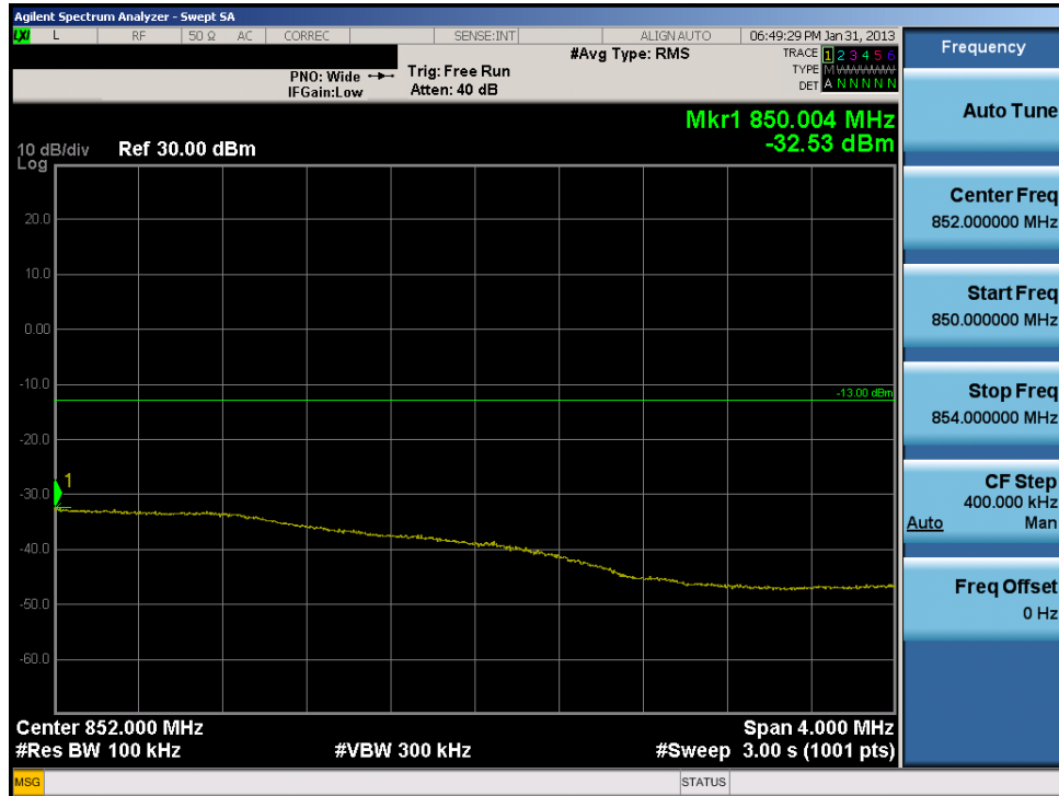
Plot 7-42. 4MHz Span Plot (Cellular WCDMA Mode – Ch. 4233)
