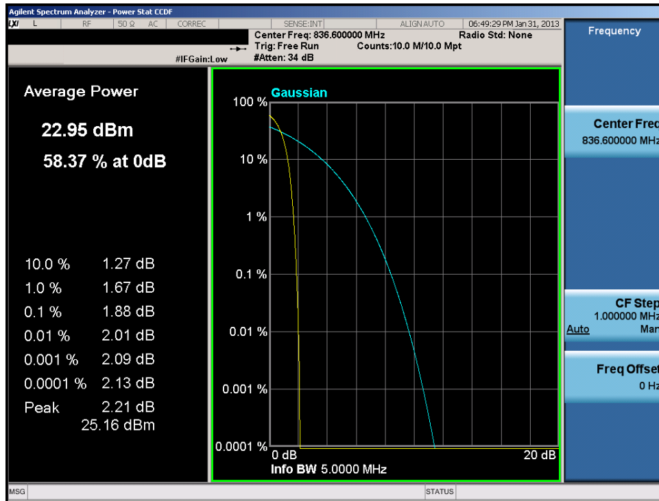
Plot 7-38. Peak-Average Ratio Plot (Cellular WCDMA Mode – Ch. 4183)
