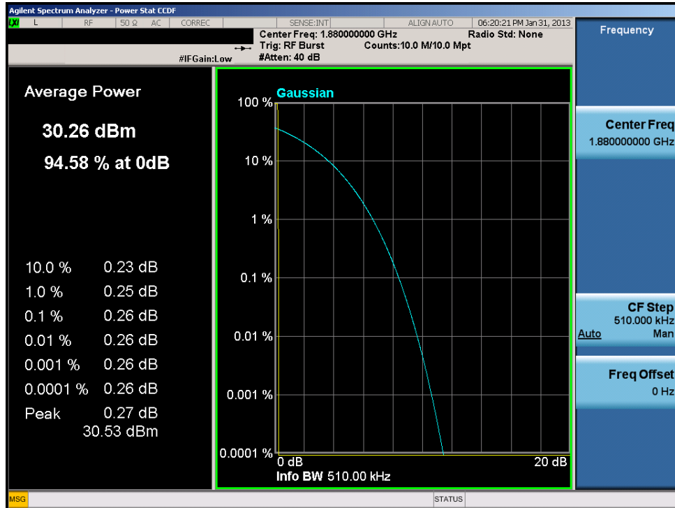
Plot 7-24. Peak-Average Ratio Plot (PCS GSM Mode – Ch. 661)
