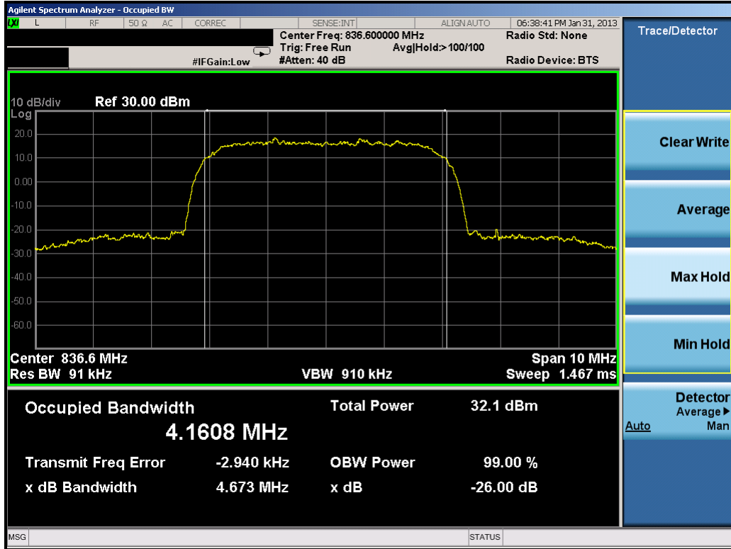
Plot 7-37. Occupied Bandwidth Plot (Cellular WCDMA Mode – Ch. 4183)
