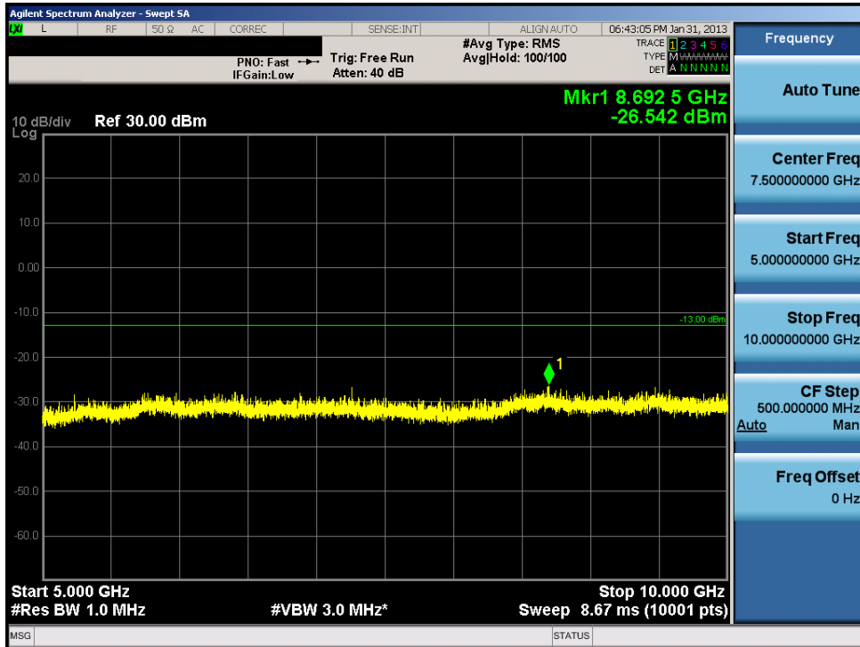
Plot 7-40. Conducted Spurious Plot (Cellular WCDMA Mode – Ch. 4233)
