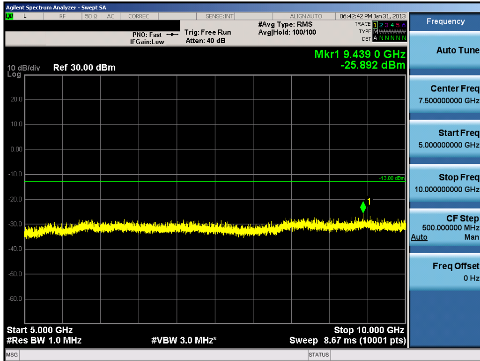
Plot 7-32. Conducted Spurious Plot (Cellular WCDMA Mode – Ch. 4132)
