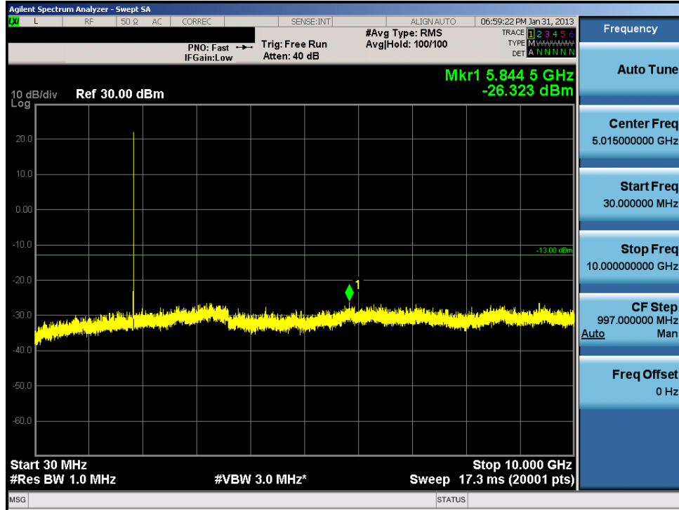
Plot 7-43. Conducted Spurious Plot (PCS WCDMA Mode – Ch. 9262)
