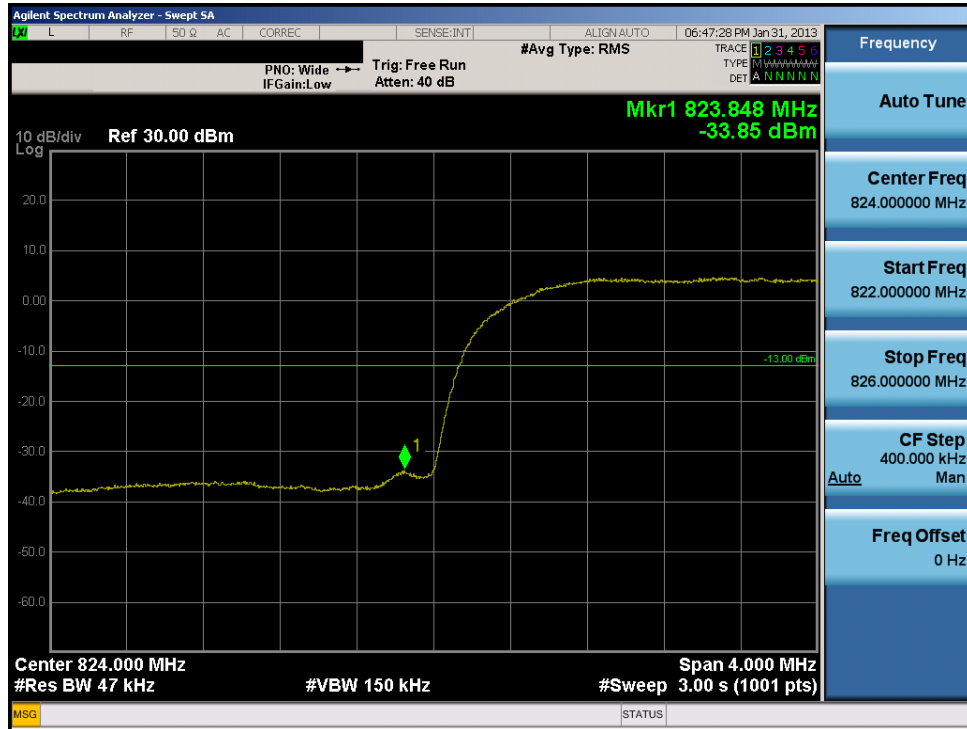
Plot 7-33. Band Edge Plot (Cellular WCDMA Mode – Ch. 4132)
