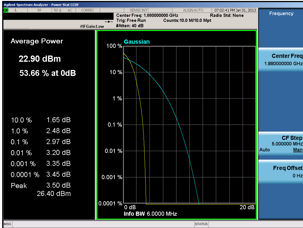
Plot 7-50. Peak-Average Ratio Plot (PCS WCDMA Mode – Ch. 9400)
