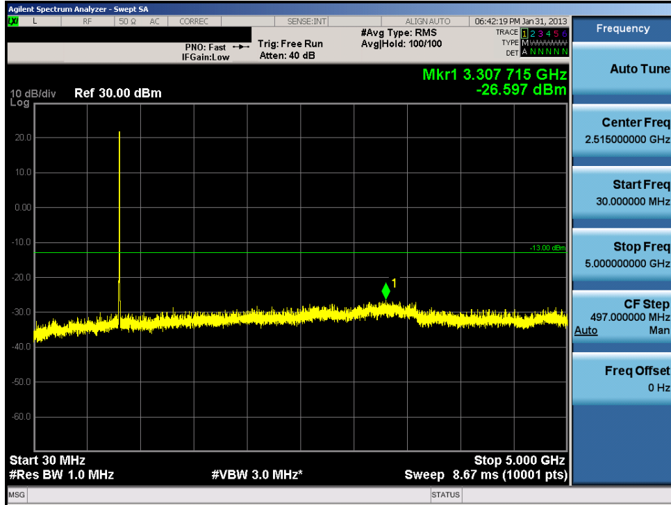
Plot 7-31. Conducted Spurious Plot (Cellular WCDMA Mode – Ch. 4132)
