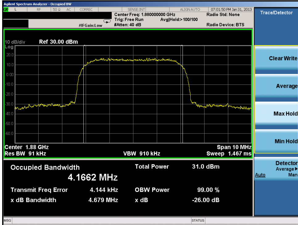
Plot 7-49. Occupied Bandwidth Plot (PCS WCDMA Mode – Ch. 9400)
