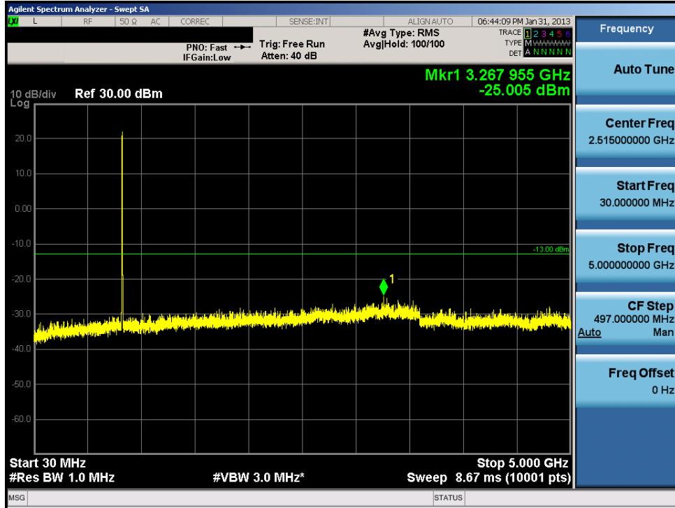
Plot 7-39. Conducted Spurious Plot (Cellular WCDMA Mode – Ch. 4233)
