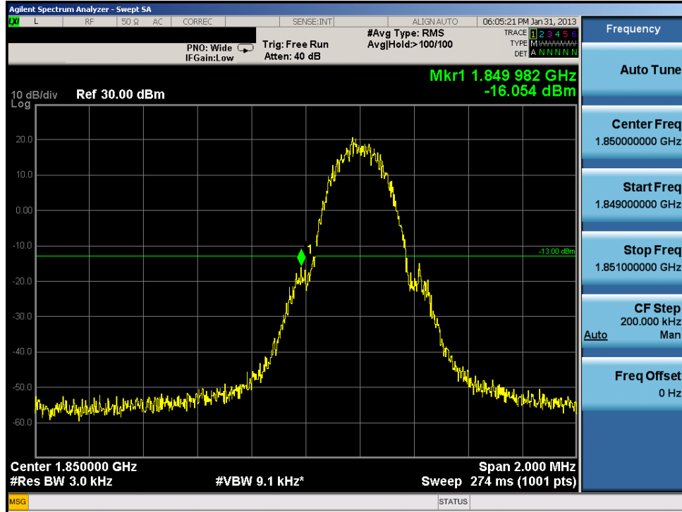
Plot 7-19. Band Edge Plot (PCS GSM Mode – Ch. 512)
