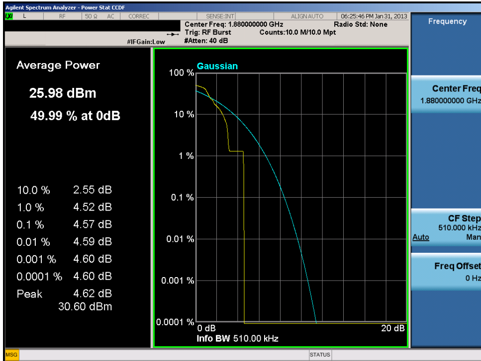
Plot 7-30. Peak-Average Ratio Plot (EDGE1900 Mode – Ch. 661)
