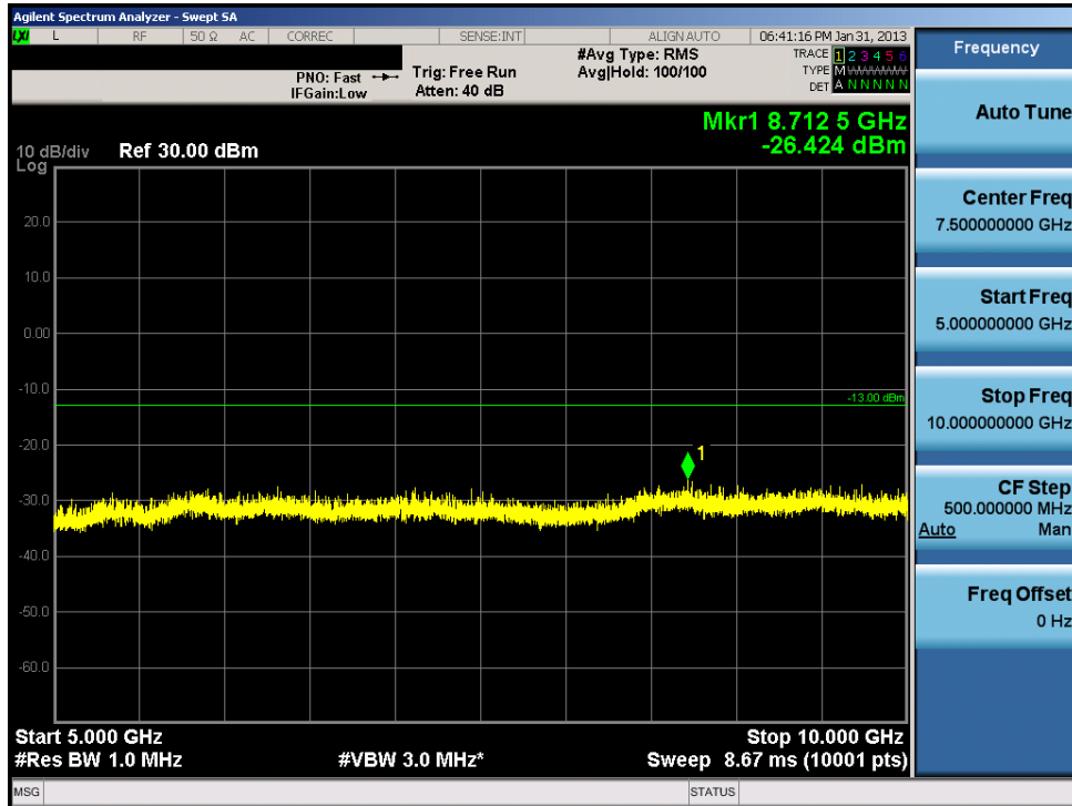
Plot 7-36. Conducted Spurious Plot (Cellular WCDMA Mode – Ch. 4183)
