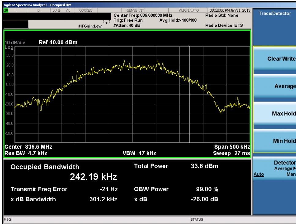
Plot 7-14. Occupied Bandwidth Plot (EDGE850 Mode – Ch. 190)
