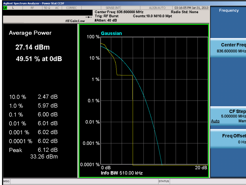
Plot 7-15. Peak-Average Ratio Plot (EDGE850 Mode – Ch. 190)
