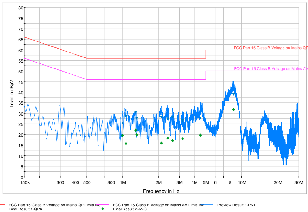
Plot 6-15. Line Conducted Plot with Bluetooth LE (L1)
