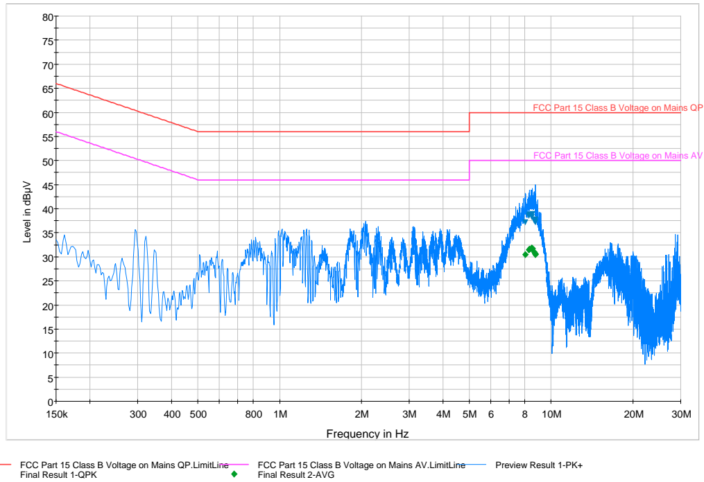
Plot 6-16. Line Conducted Plot with Bluetooth LE (N)
