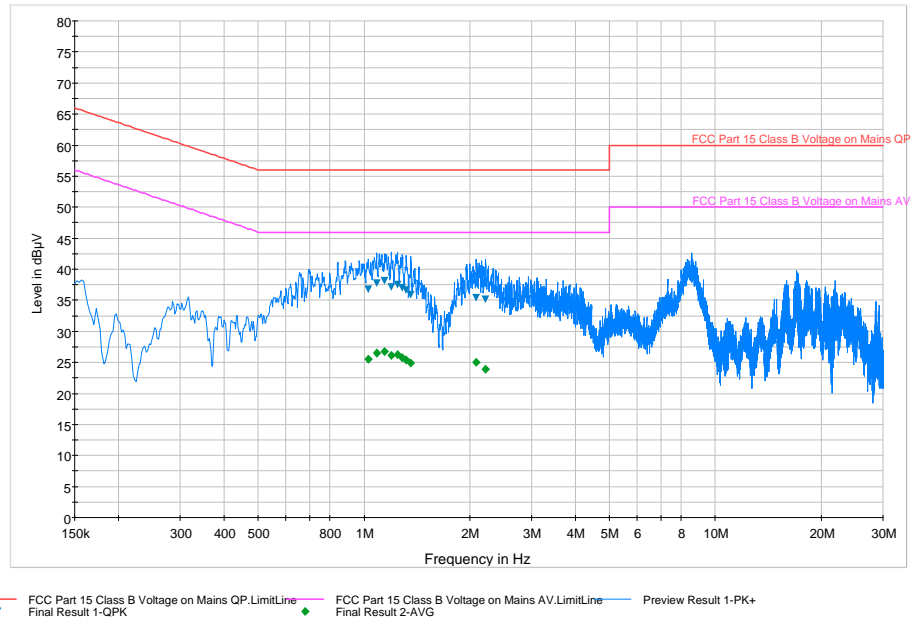
Plot 6-62. Line Conducted Plot with 802.11a (N)
