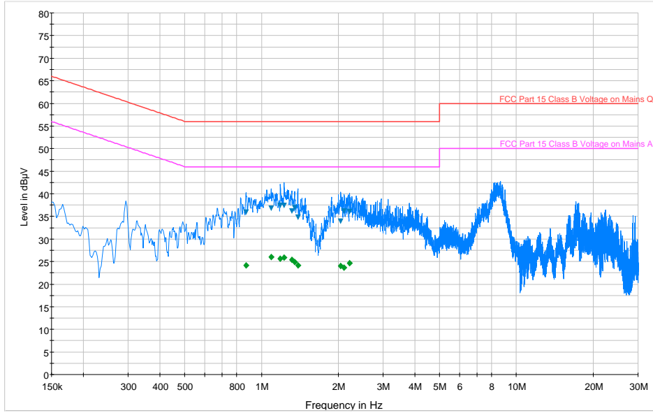
— FCC Part 15 Class B Voltage on Mains QP.LimitLine — FCC Part 15 Class B Voltage on Mains AV.LimitLine — Preview Result 1-PK+ ▼ Final Result 1-QPK ◆ Final Result 2-AVG
