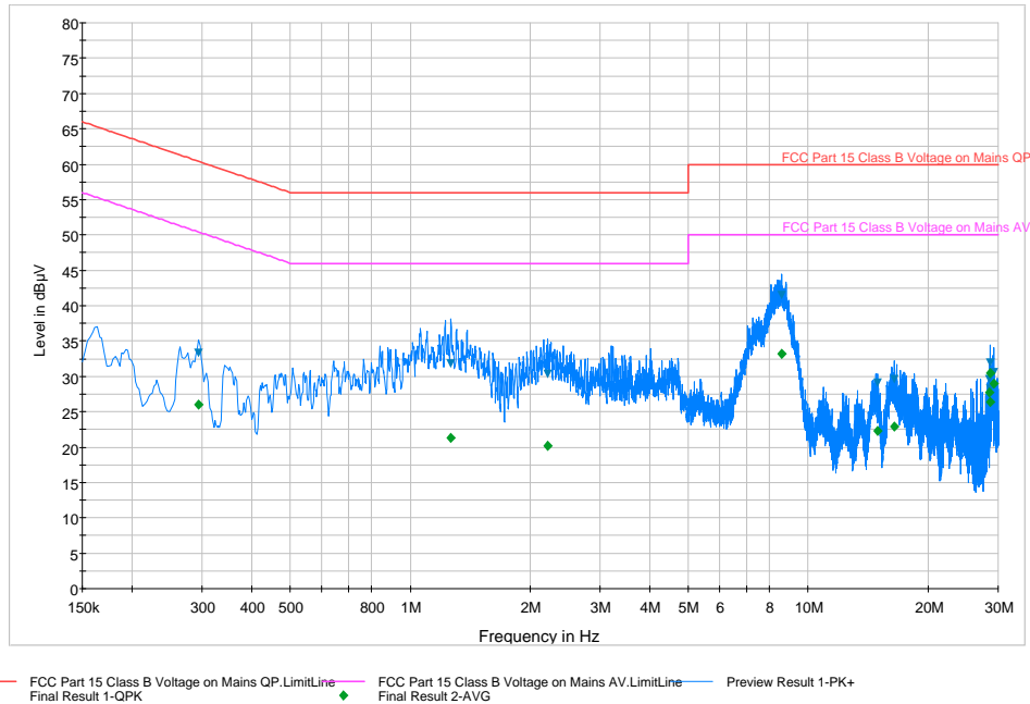
Plot 6-61. Line Conducted Plot with 802.11a (L1)
