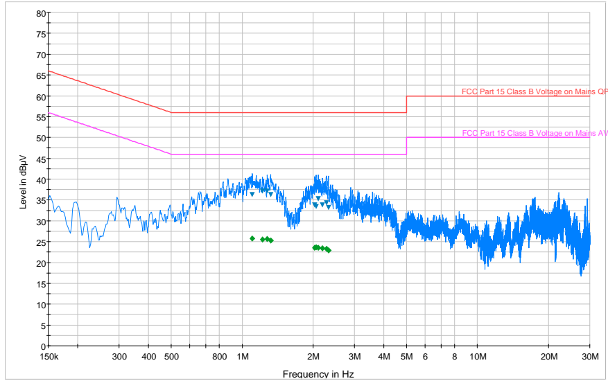
Plot 6-79. Line Conducted Plot with 802.11a UNII Band 2 (N)
