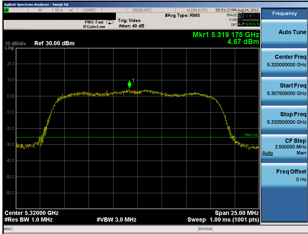
Plot 6-36. Peak Power Spectral Density Plot (802.11a (UNII Band 2) – Ch. 64)
