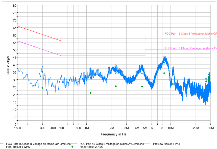
Plot 6-76. Line Conducted Plot with 802.11a UNII Band 1 (L1)
