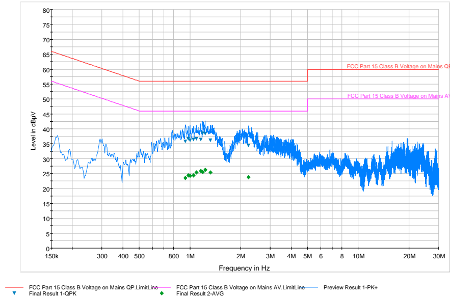
Plot 6-81. Line Conducted Plot with 802.11a UNII Band 3 (N)
