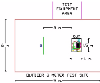
Figure 3.2-2. Dimensions of Outdoor Test Site
