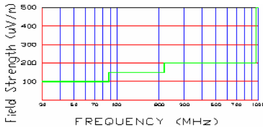
Figure C-1. 3 Meter Limits
