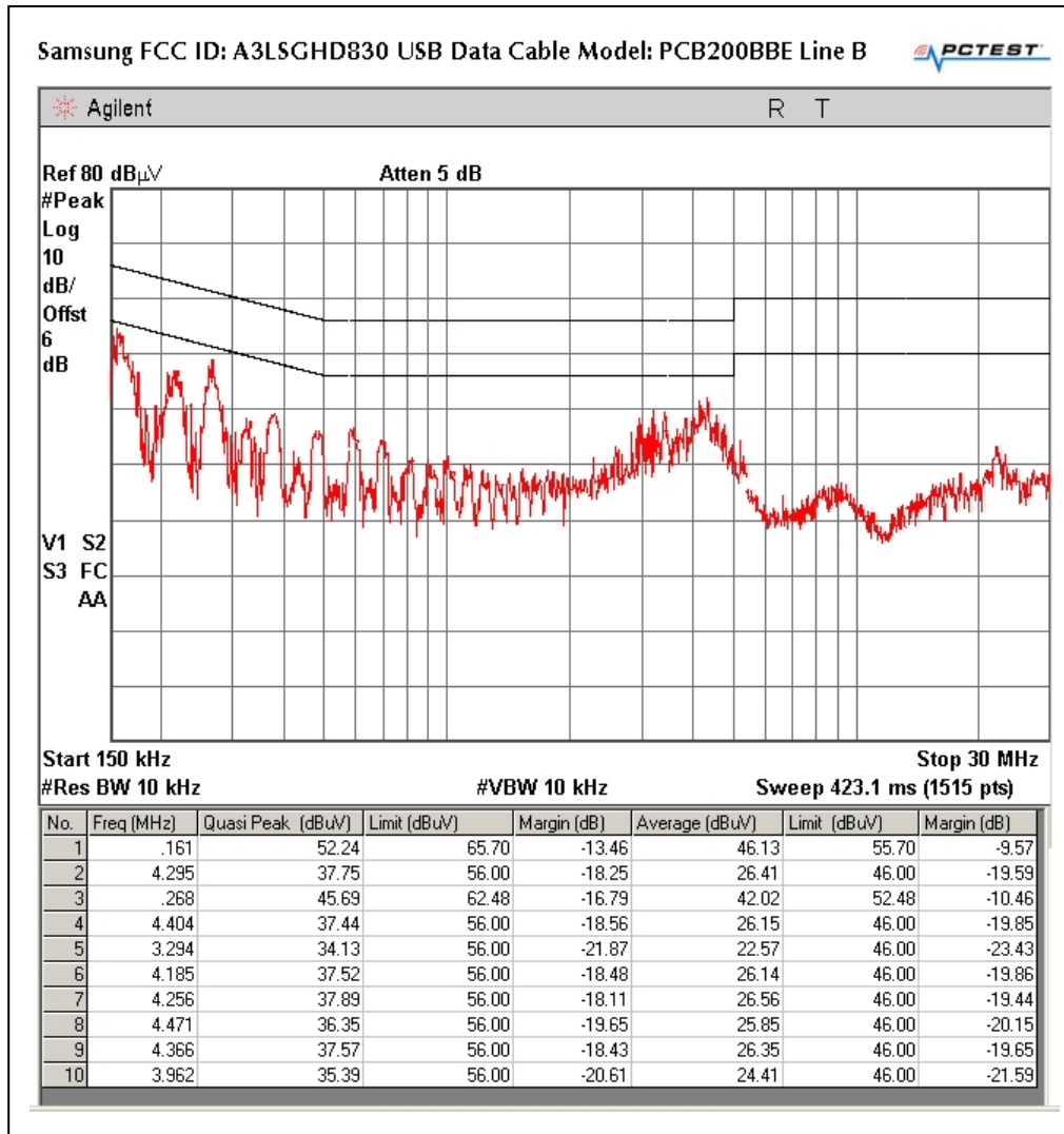
Plot C-2. Line-Conducted Test Plot
