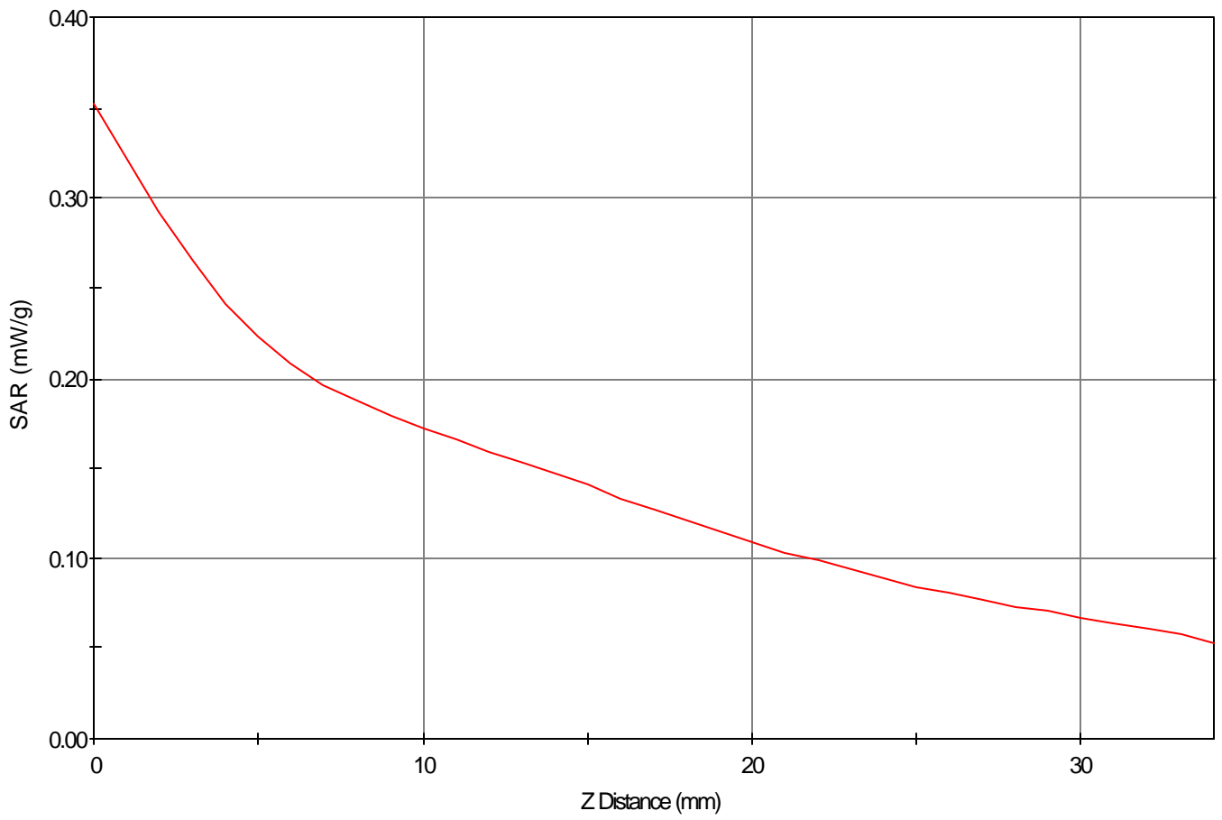
SAR - Z Axis at Hotspot x:39.0 y:-2.0
