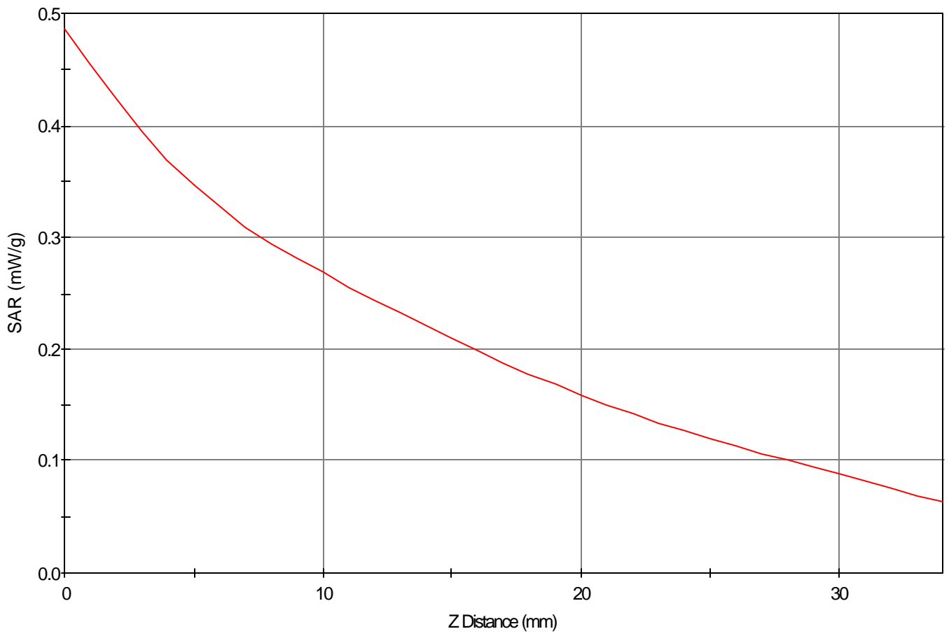
SAR - Z Axis at Hotspot x:59.0 y:4.0
