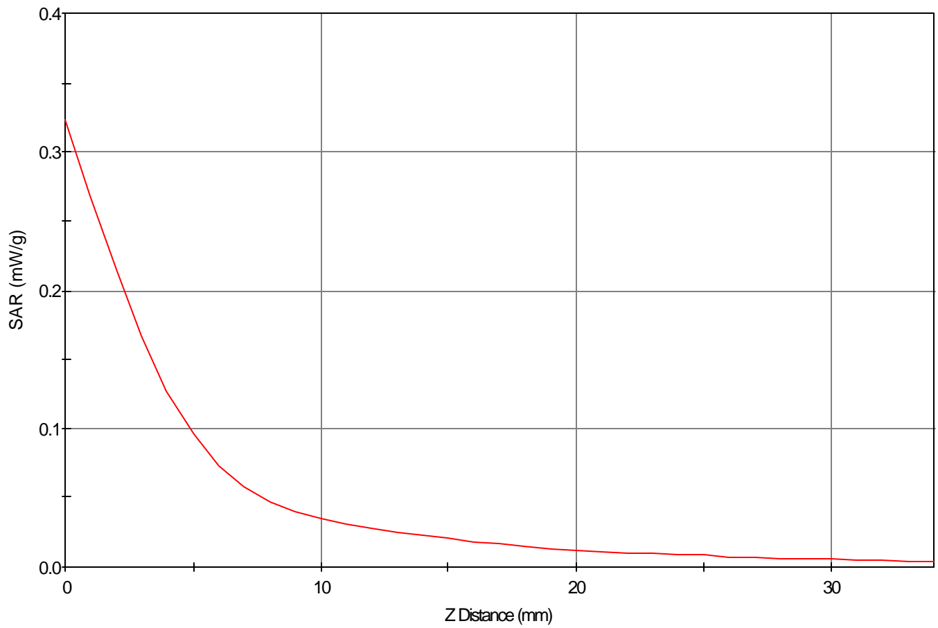
SAR - Z Axis at Hotspot x:67.0 y:25.0
