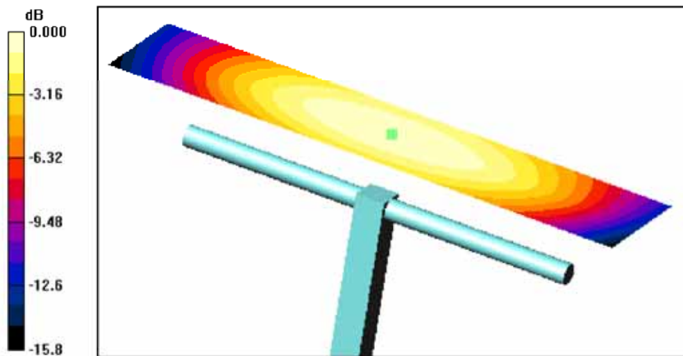
0 dB = 0.460A/m
