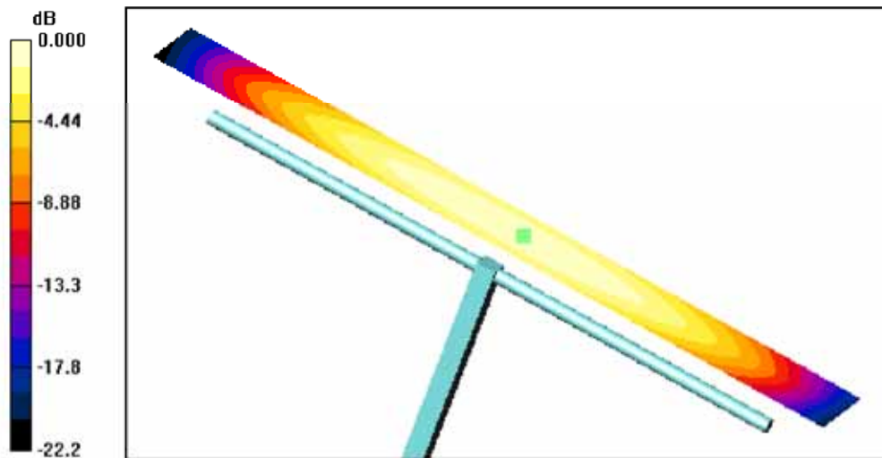
0 dB = 0.513A/m
