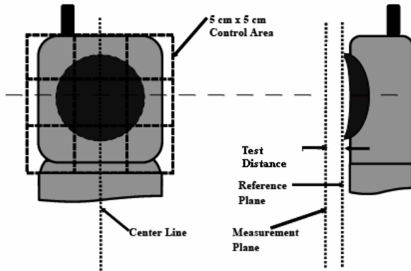
Figure 6-1 E/H-Field Emissions Test Setup Diagram
