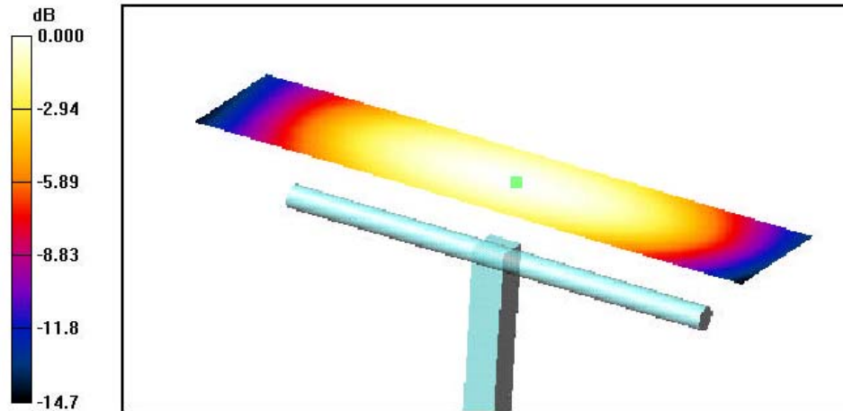
0 dB = 0.440A/m
