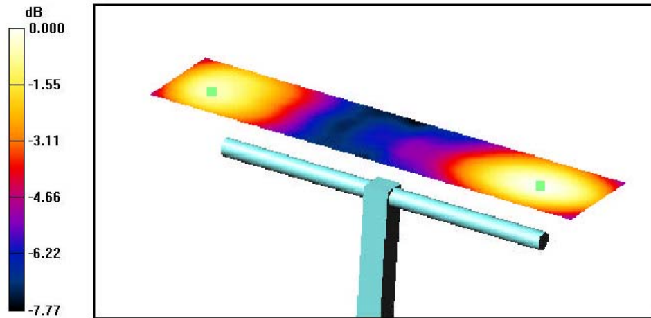
0 dB = 145.6V/m
