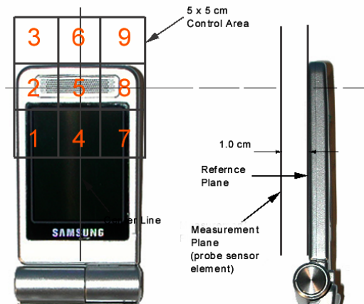
Figure 13 E/H-Field Emissions Test Setup Diagram
