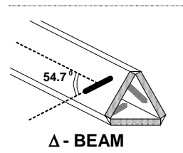
Figure 3.3 Triangular Probe Configuration
