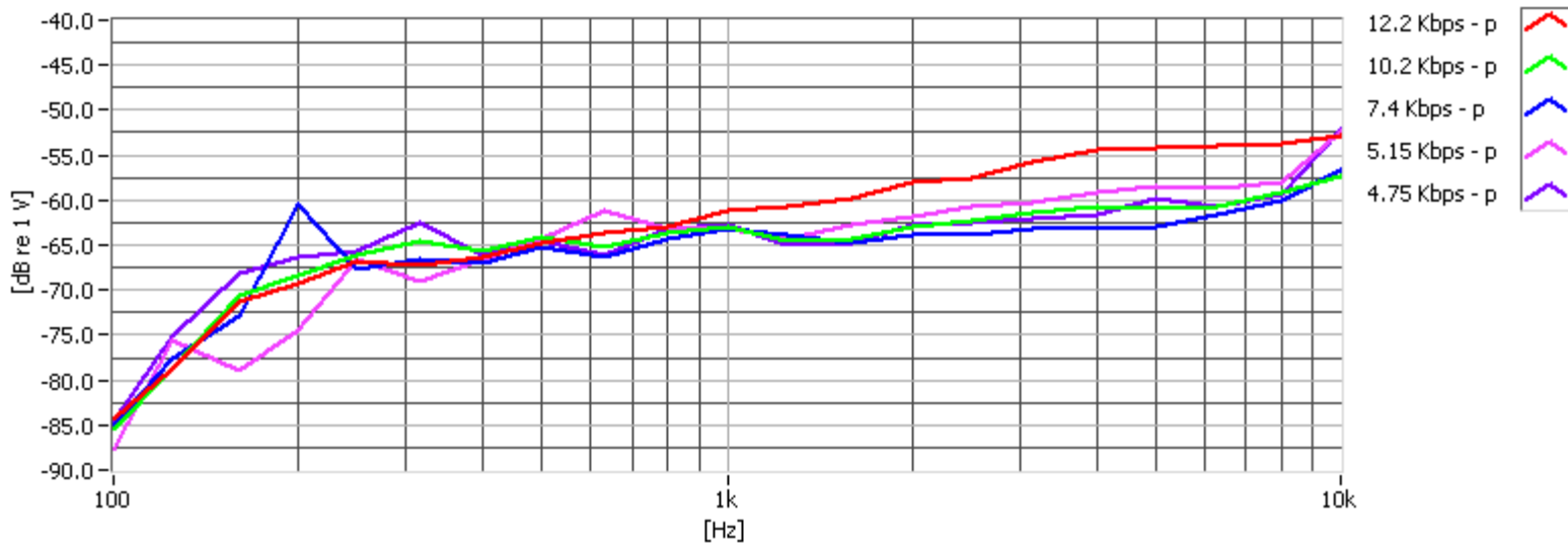
Figure 5-7 Vocoder Analysis for ABM Noise (WCDMA)
