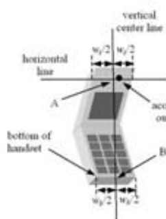
Figure 5.4 Handset vertical and horizontal reference lines
