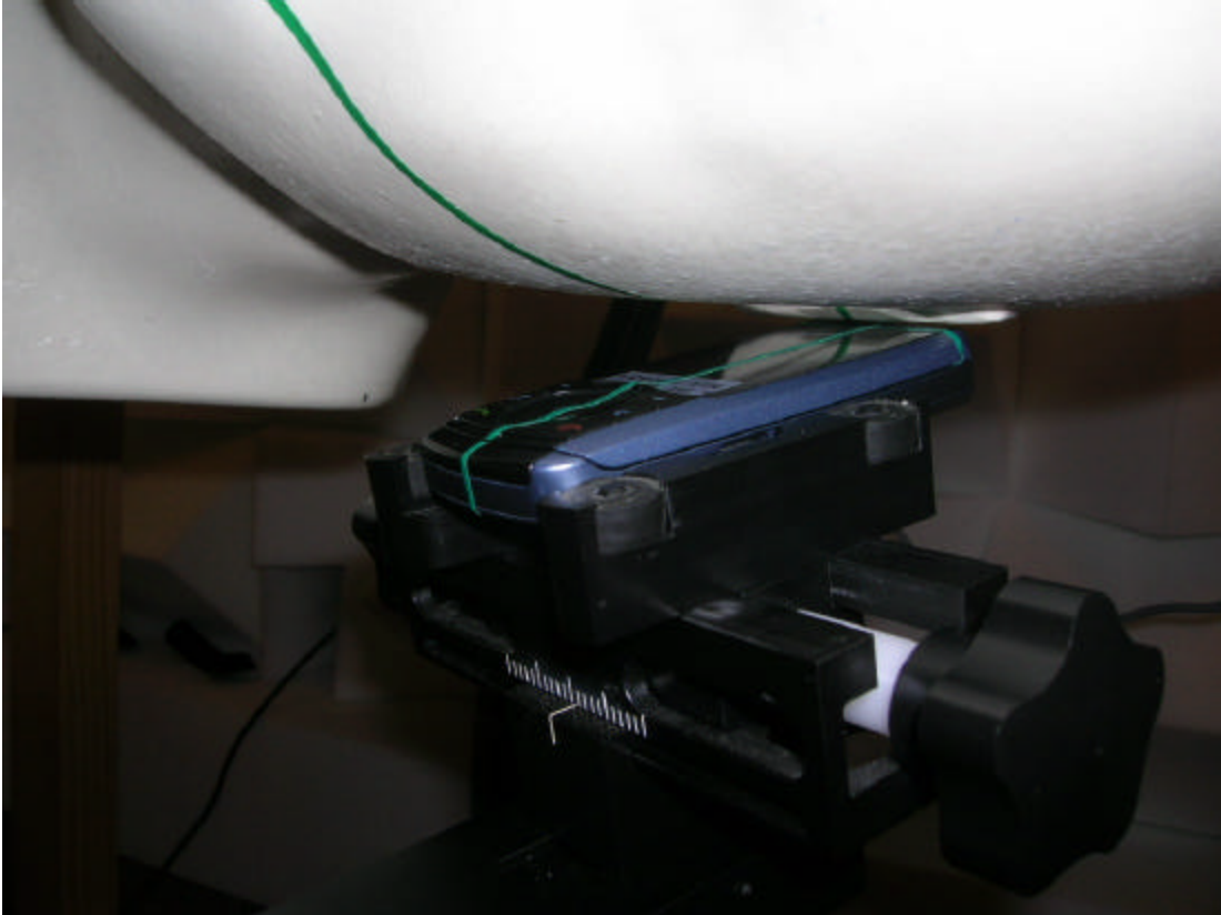
9. Left Head SAR, Slide In, 15° Tilt
