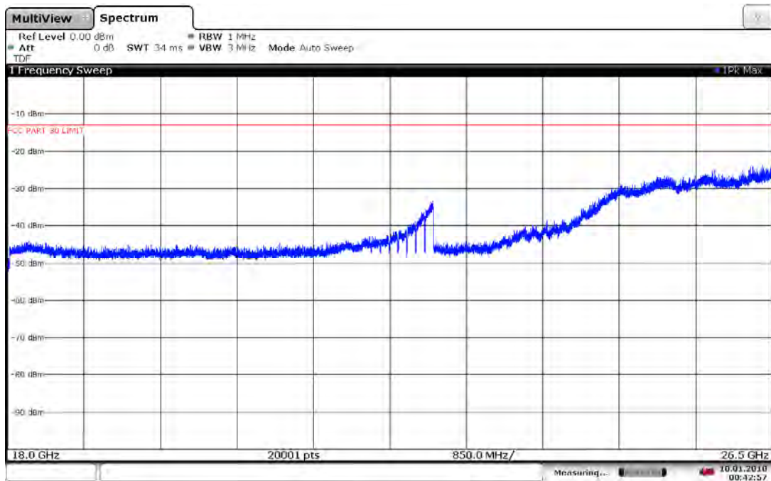
Plot 7-76. Antenna B Radiated Spurious Plot 18-26.5 GHz (8CC QPSK Mid Channel)
