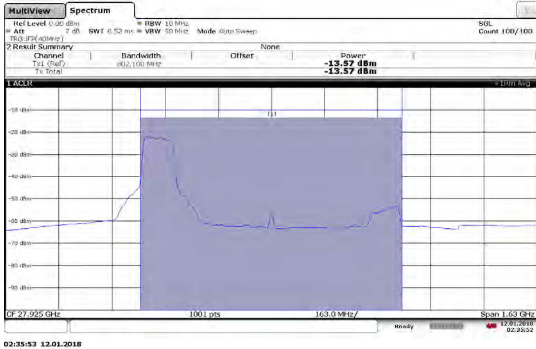
Plot 7-17. Antenna A EIRP Plot (1CC 16QAM Mid Channel)
