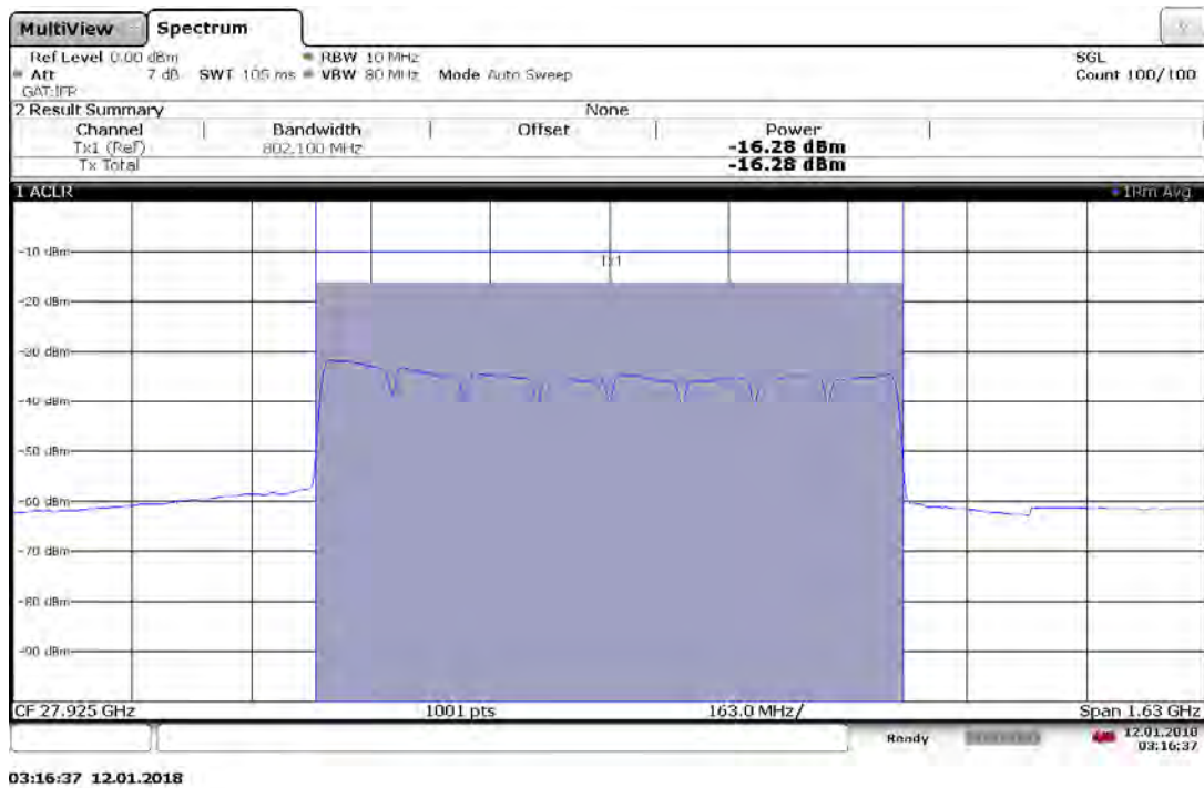
Plot 7-23. Antenna A EIRP Plot (8CC 16QAM Mid Channel)
