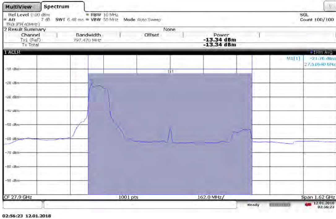
Plot 7-19. Antenna A EIRP Plot (1CC 64QAM Low Channel)
