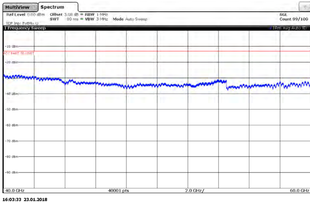
Plot 7-56. Antenna A Radiated Spurious Plot 40-60 GHz (8CC QPSK Mid Channel)
