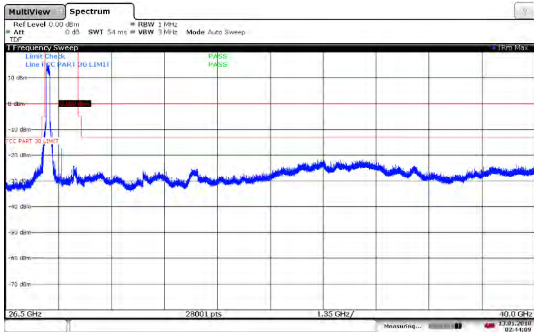
Plot 7-78. Antenna B Radiated Spurious Plot 26.5-40 GHz (1CC QPSK Mid Channel)
