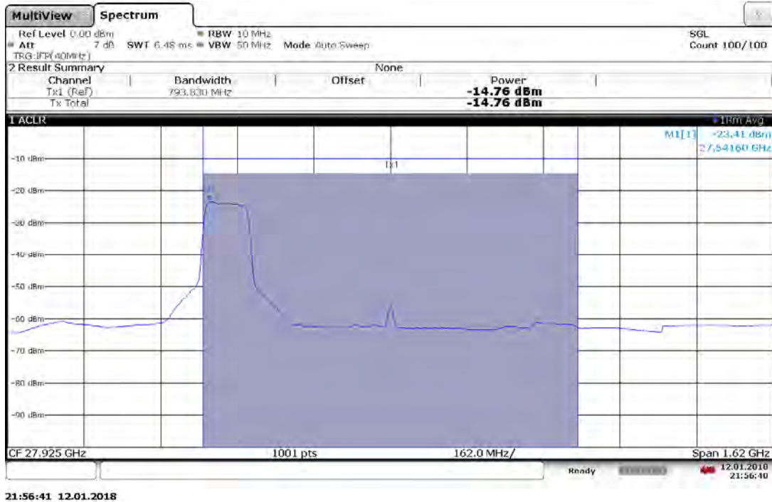
Plot 7-26. Antenna B EIRP Plot (1CC QPSK Mid Channel)
