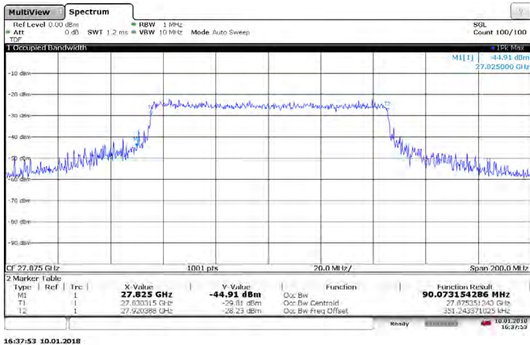
Plot 7-7. Occupied Bandwidth Plot (1CC QPSK Mid Channel)
