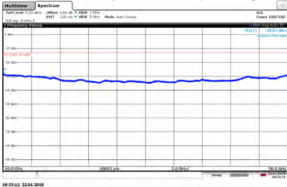
Plot 7-60. Antenna A Radiated Spurious Plot 60-90 GHz (8CC QPSK Mid Channel)
