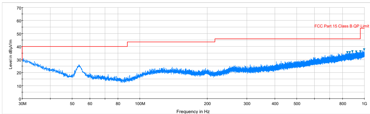
Plot 7-67. Antenna B Radiated Spurious Plot 30 MHz - 1 GHz (1CC QPSK High Channel)
