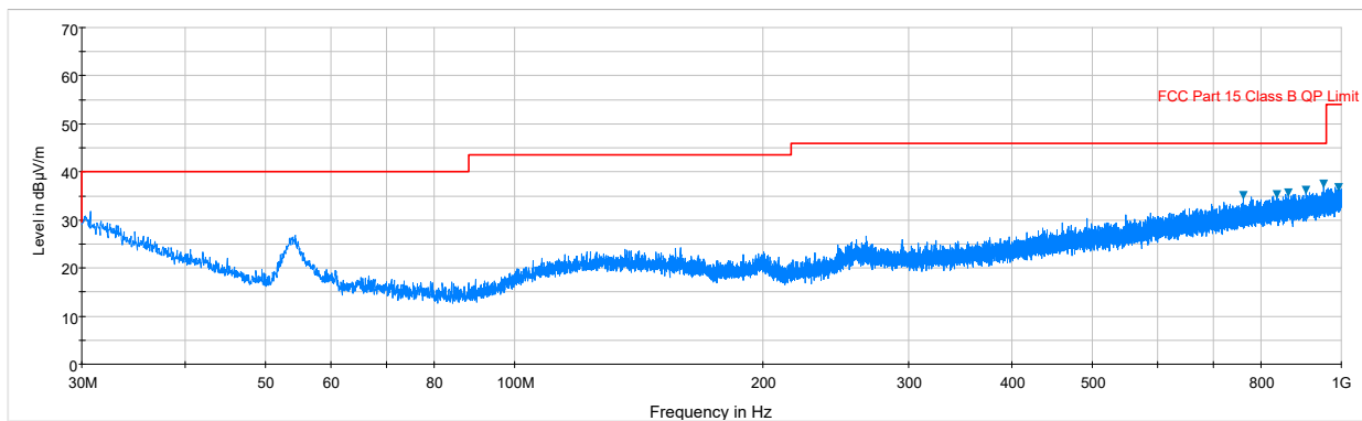
Plot 7-39. Antenna A Radiated Spurious Plot 30 MHz - 1 GHz (1CC QPSK High Channel)
