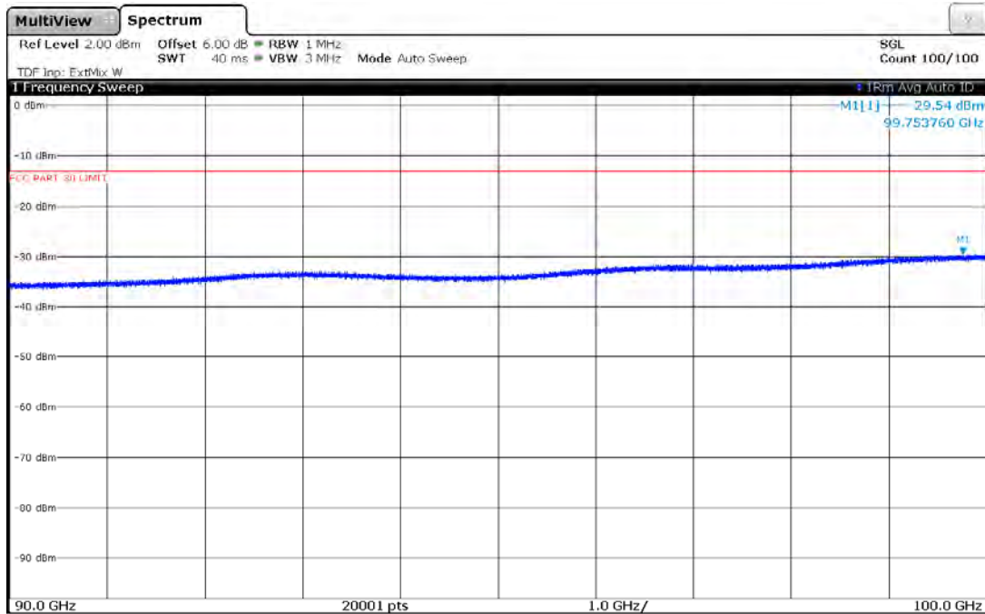
Plot 7-89. Antenna B Radiated Spurious Plot 90-100 GHz (1CC QPSK Low Channel)
