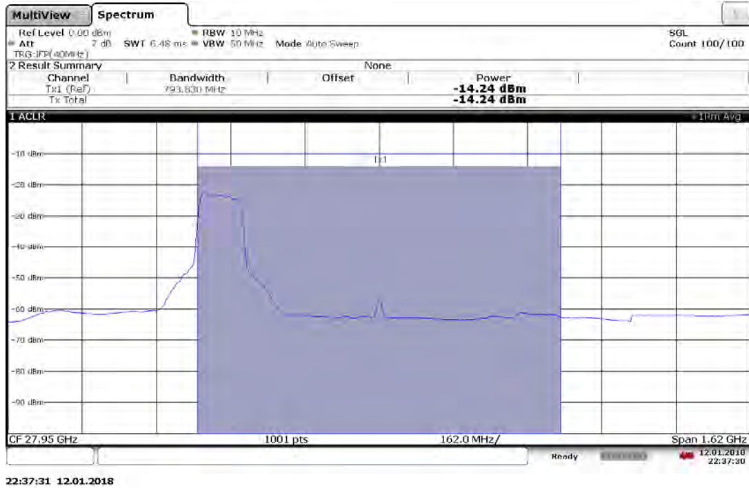
Plot 7-27. Antenna B EIRP Plot (1CC QPSK High Channel)
