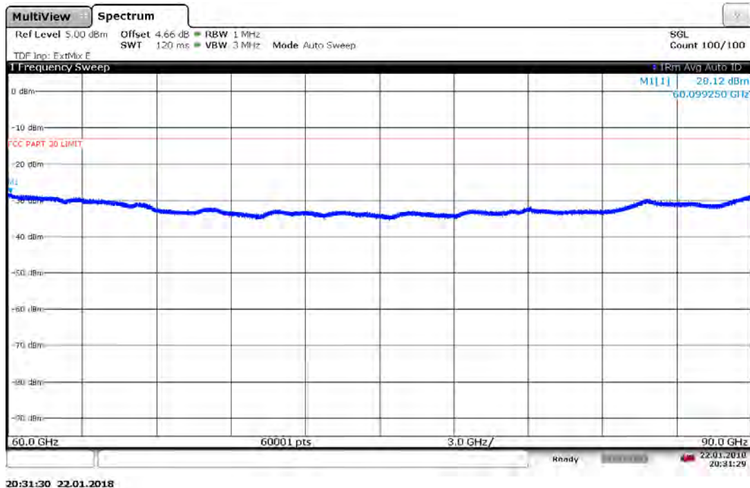
Plot 7-86. Antenna B Radiated Spurious Plot 60-90 GHz (1CC QPSK Mid Channel)
