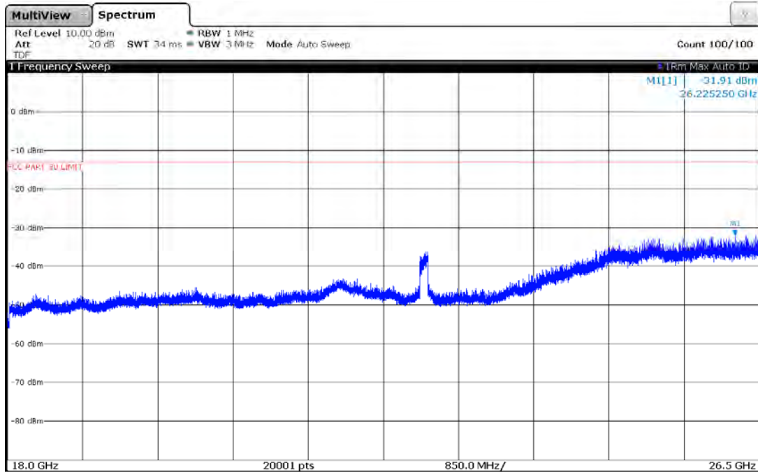
Plot 7-75. Antenna B Radiated Spurious Plot 18-26.5 GHz (1CC QPSK High Channel)
