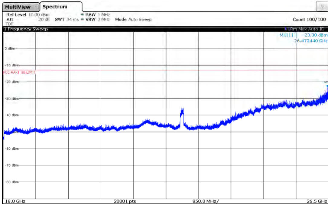
Plot 7-73. Antenna B Radiated Spurious Plot 18-26.5 GHz (1CC QPSK Low Channel)
