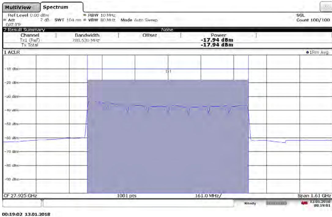
Plot 7-36. Antenna B EIRP Plot (8CC 64QAM Mid Channel)
