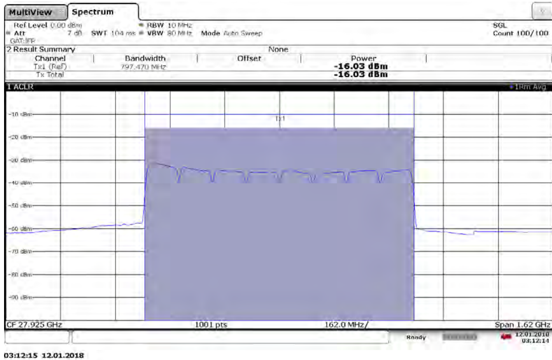
Plot 7-24. Antenna A EIRP Plot (8CC 64QAM Mid Channel)
