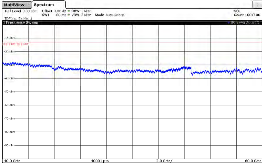
Plot 7-81. Antenna B Radiated Spurious Plot 40-60 GHz (1CC QPSK Low Channel)
