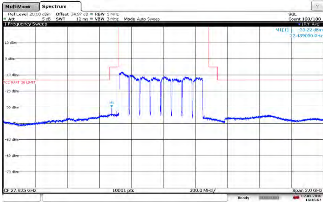
Plot 7-97. Band Edge Plot (8CC 16QAM Low Channel)
