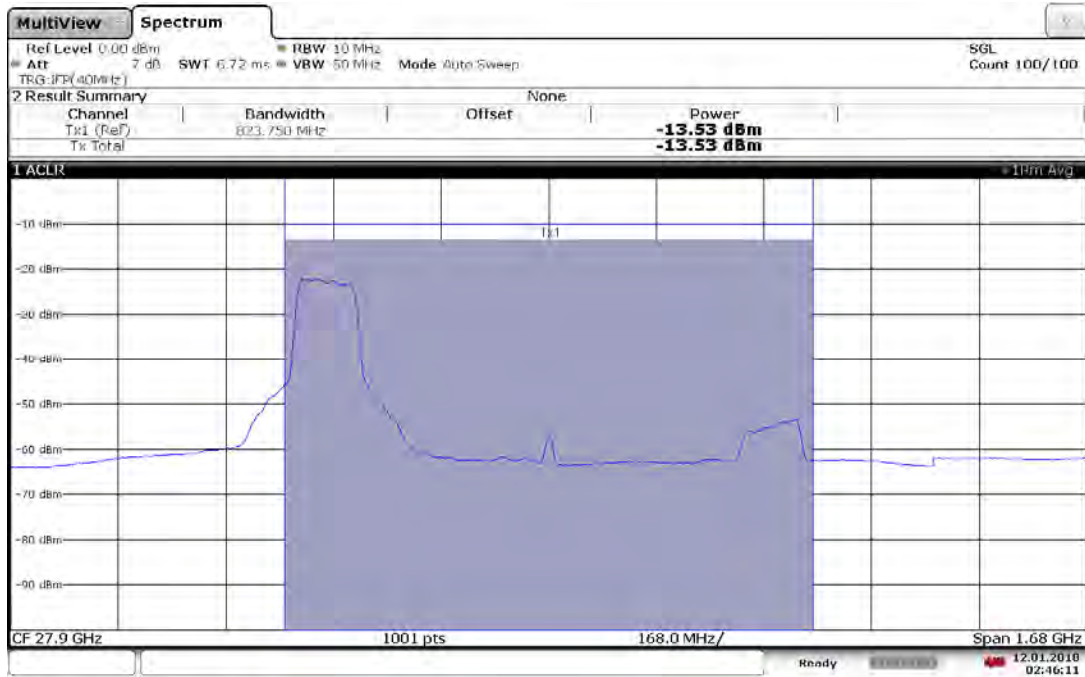
Plot 7-16. Antenna A EIRP Plot (1CC 16QAM Low Channel)
