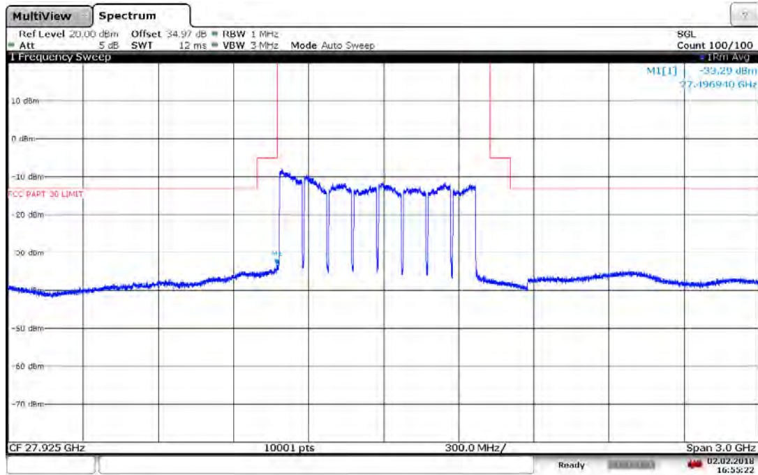
Plot 7-108. Band Edge Plot (8CC QPSK Low Channel)
