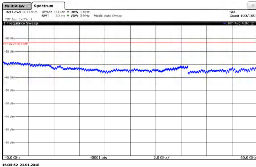
Plot 7-84. Antenna B Radiated Spurious Plot 40-60 GHz (8CC QPSK Mid Channel)
