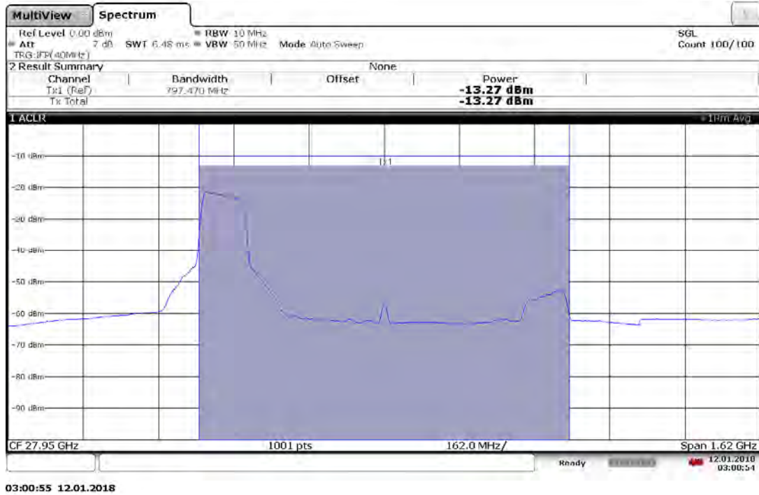
Plot 7-21. Antenna A EIRP Plot (1CC 64QAM High Channel)
