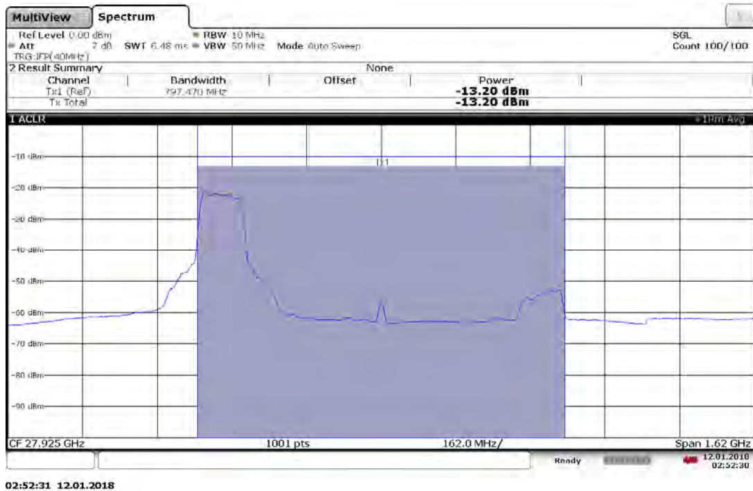
Plot 7-20. Antenna A EIRP Plot (1CC 64QAM Mid Channel)
