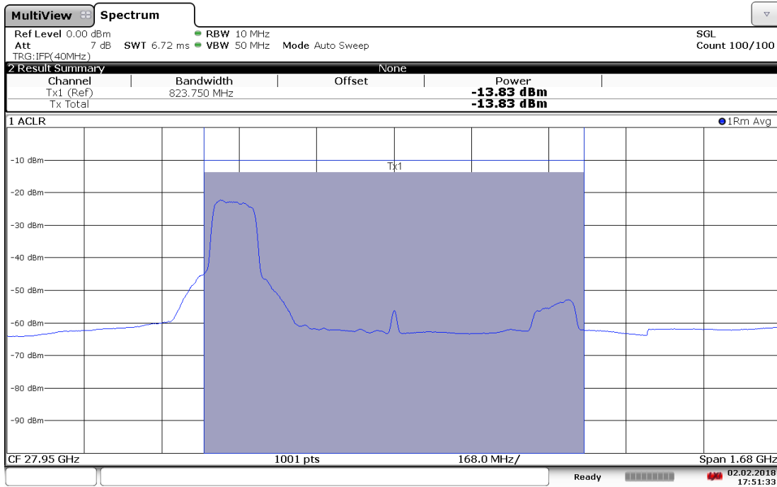
Plot 7-15. Antenna A EIRP Plot (1CC QPSK High Channel)
