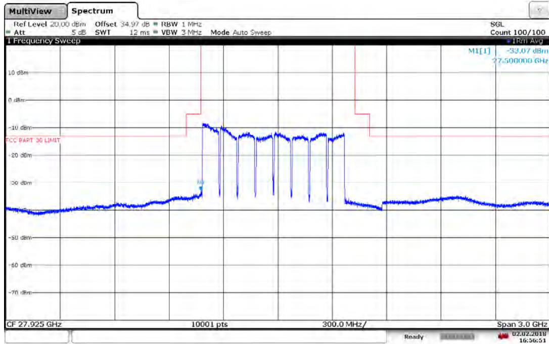
Plot 7-109. Band Edge Plot (8CC 16QAM Low Channel)
