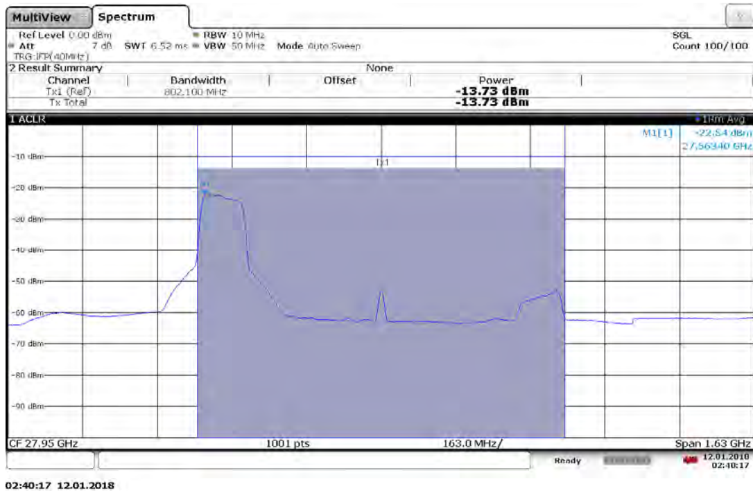
Plot 7-18. Antenna A EIRP Plot (1CC 16QAM High Channel)
