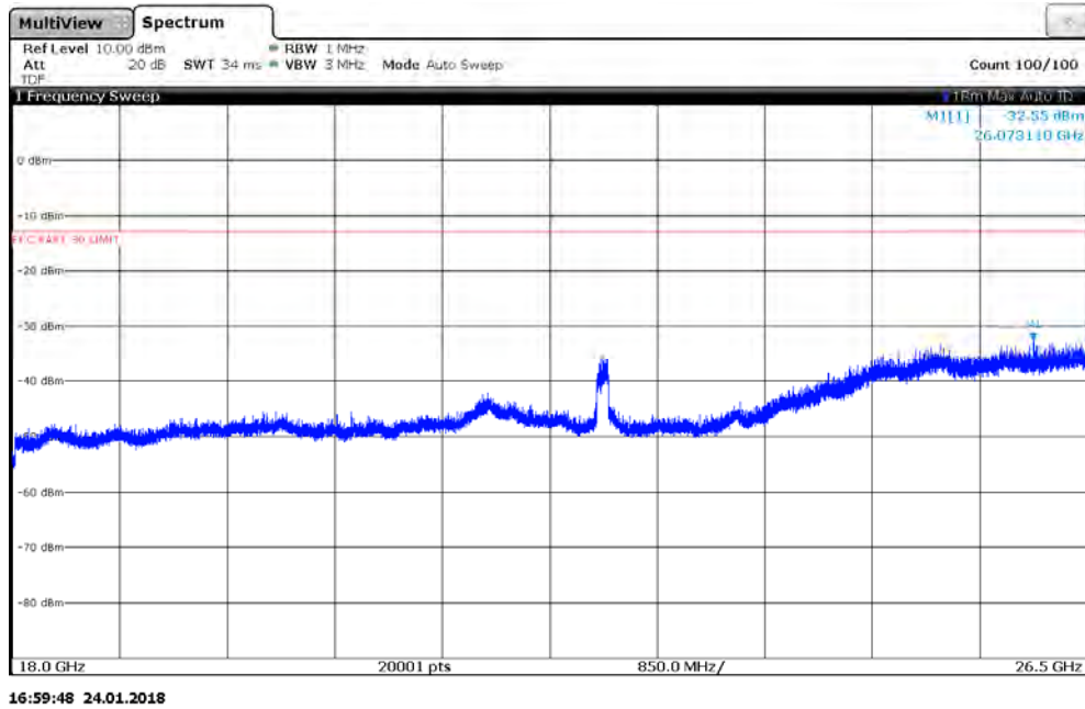
Plot 7-45. Antenna A Radiated Spurious Plot 18-26.5 GHz (1CC QPSK Low Channel)
