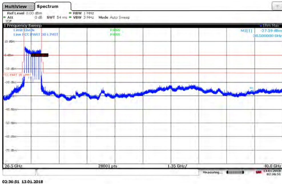
Plot 7-52. Antenna A Radiated Spurious Plot 26.5-40 GHz (8CC QPSK Mid Channel)
