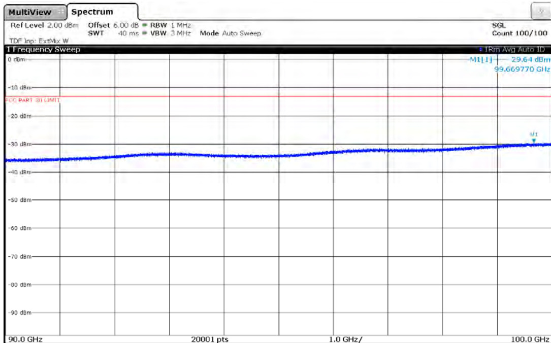
Plot 7-90. Antenna B Radiated Spurious Plot 90-100 GHz (1CC QPSK Mid Channel)
