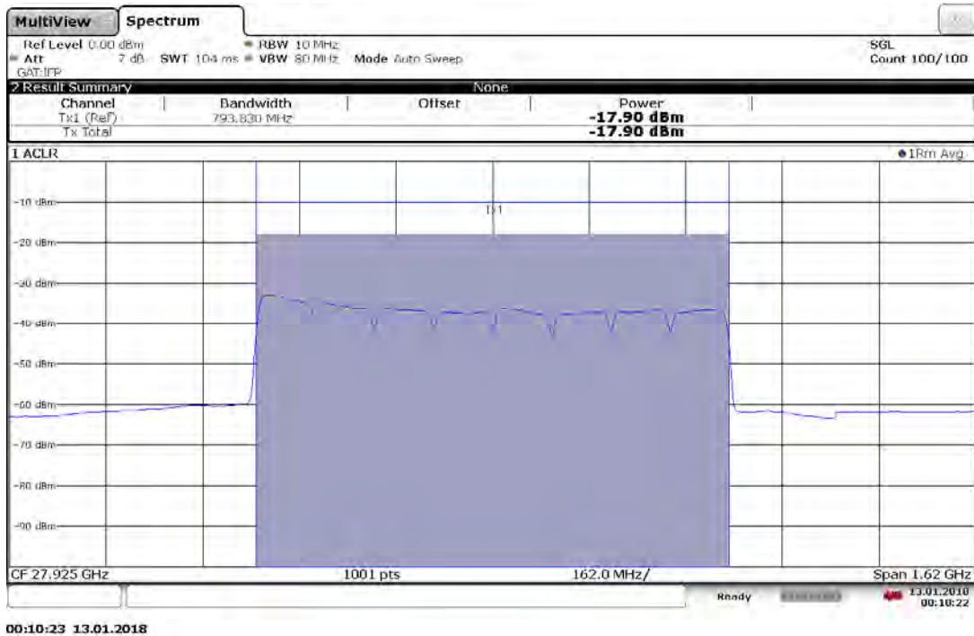
Plot 7-34. Antenna B EIRP Plot (8CC QPSK Mid Channel)
