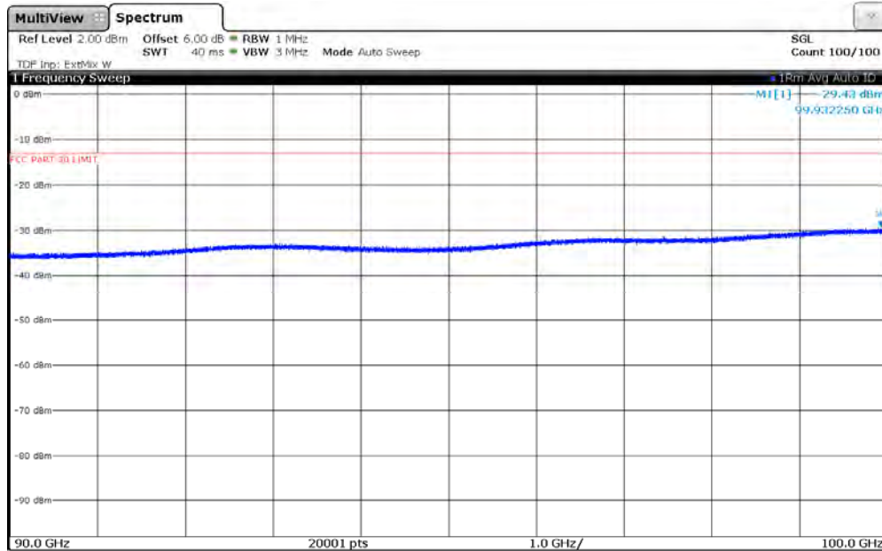
Plot 7-92. Antenna B Radiated Spurious Plot 90-100 GHz (8CC QPSK Mid Channel)
