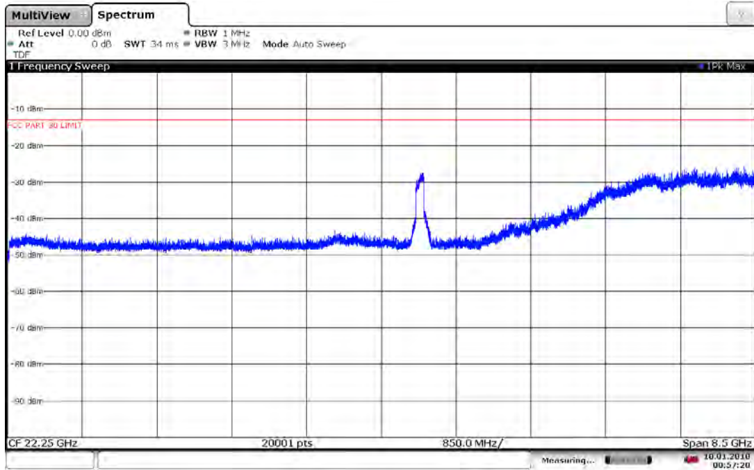
Plot 7-74. Antenna B Radiated Spurious Plot 18-26.5 GHz (1CC QPSK Mid Channel)
