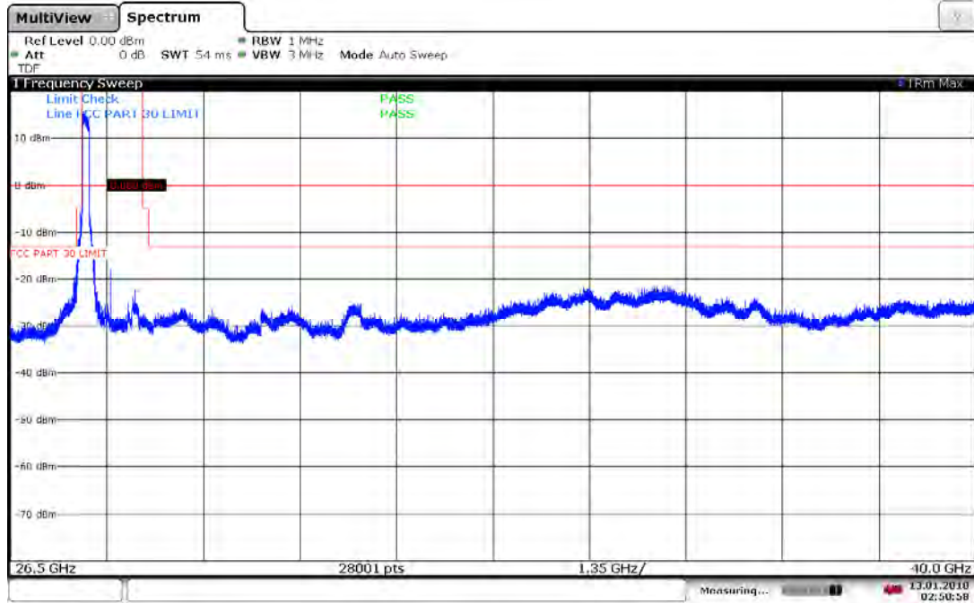
Plot 7-77. Antenna B Radiated Spurious Plot 26.5-40 GHz (1CC QPSK Low Channel)
