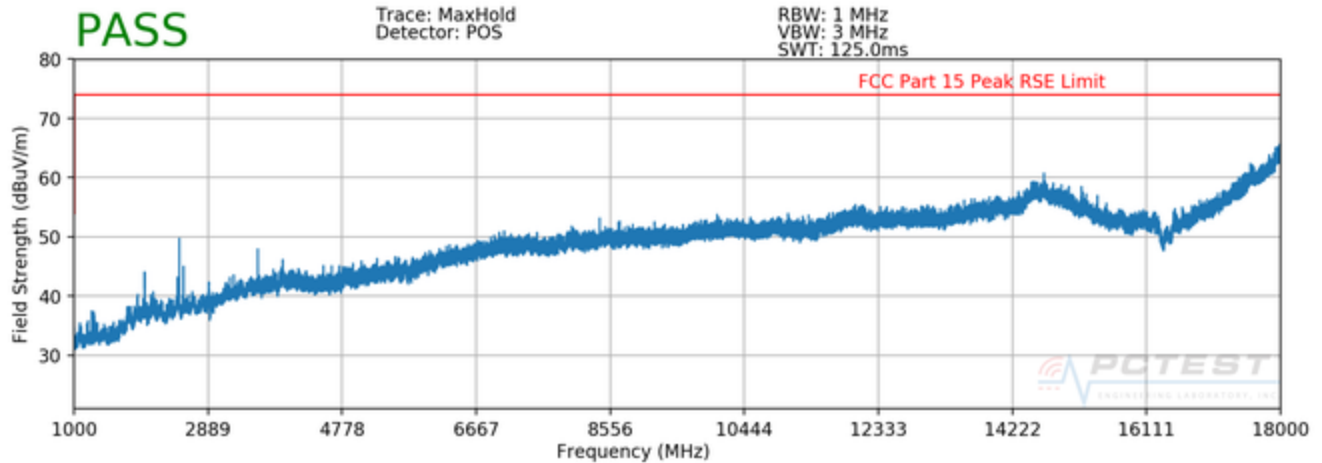
Plot 7-3. Radiated Spurious Emissions 1 - 18GHz (Ant. Pol. H)
