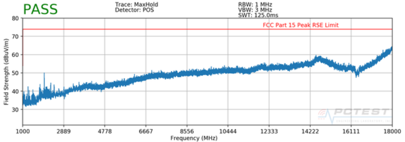
Plot 7-4. Radiated Spurious Emissions 1 - 18GHz (Ant. Pol. V)
