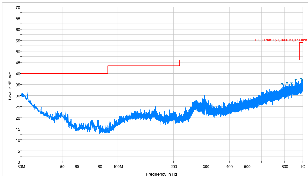
Plot 7-2. Radiated Spurious Emissions Below 1GHz (Ant. Pol. V)
