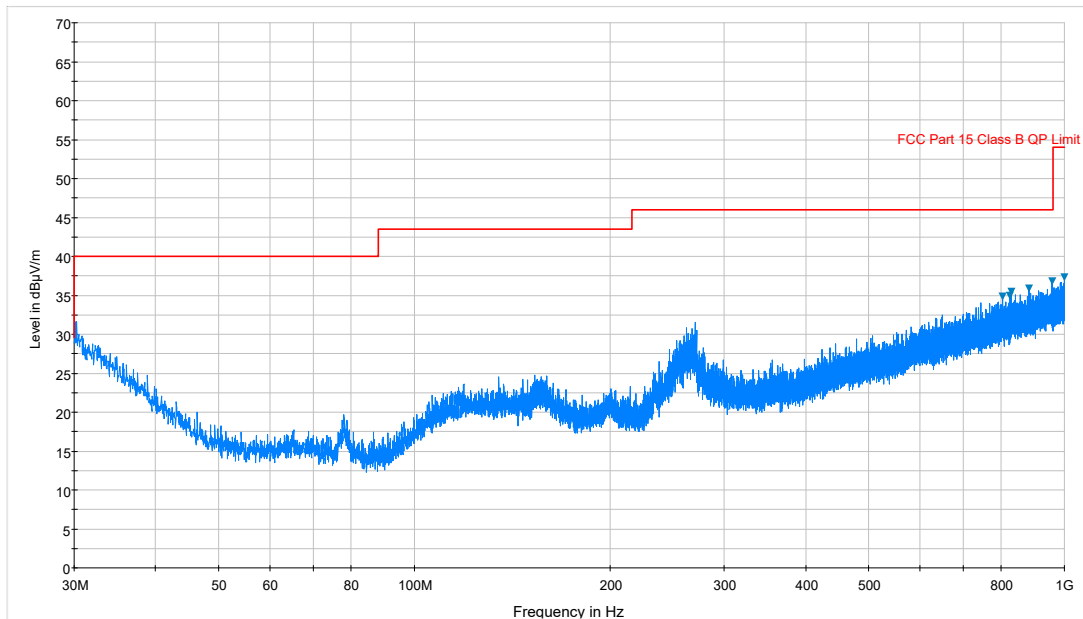
Plot 7-1. Radiated Spurious Emissions Below 1GHz (Ant. Pol. H)
