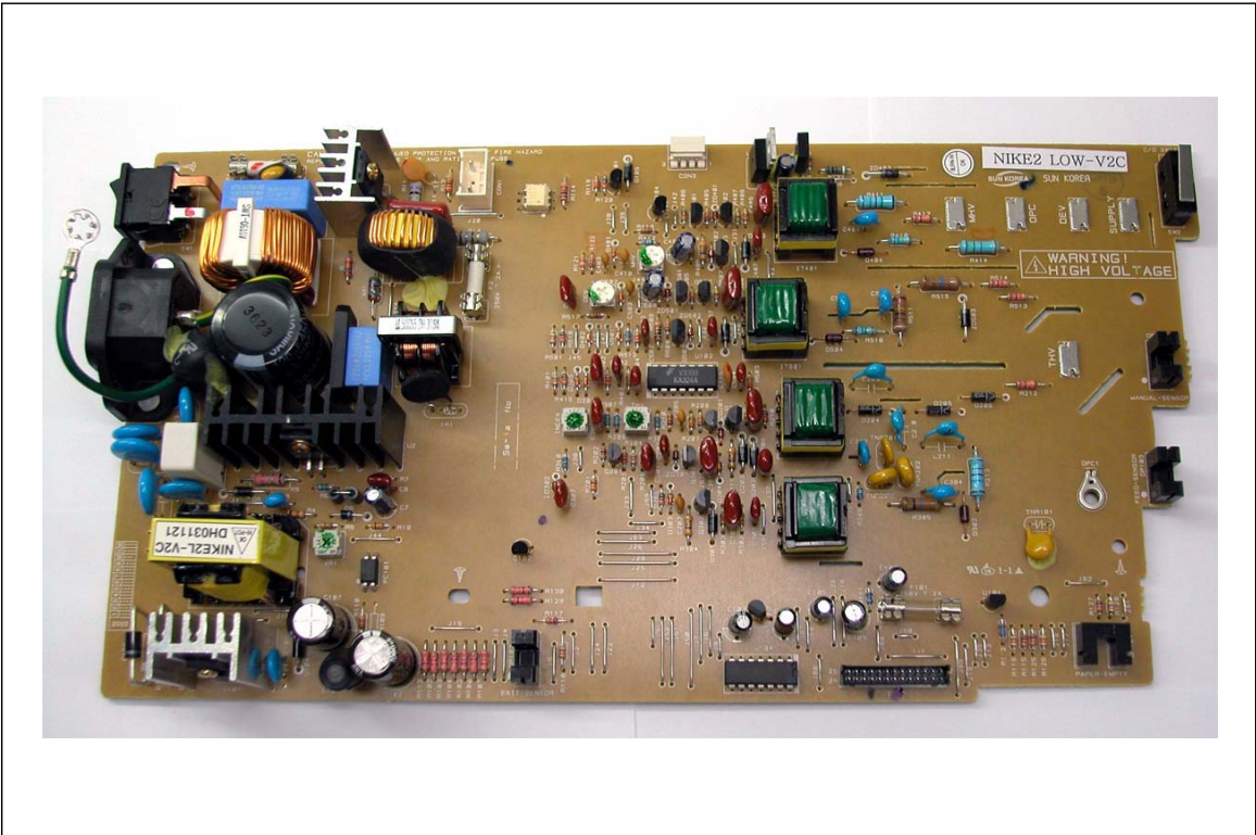
6) Top View of V2(SMPS + HVPS)
