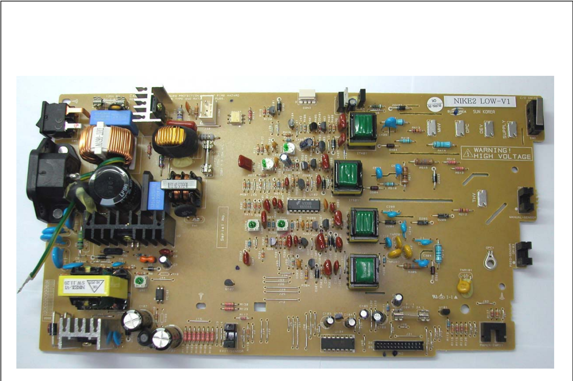
5) Top View of V1(SMPS + HVPS)
