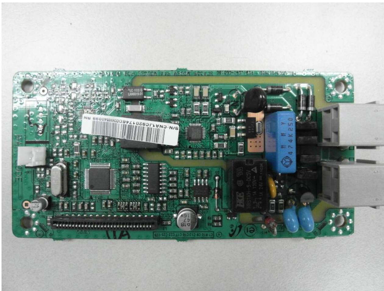
PBA Photo_FAX PBA Front
