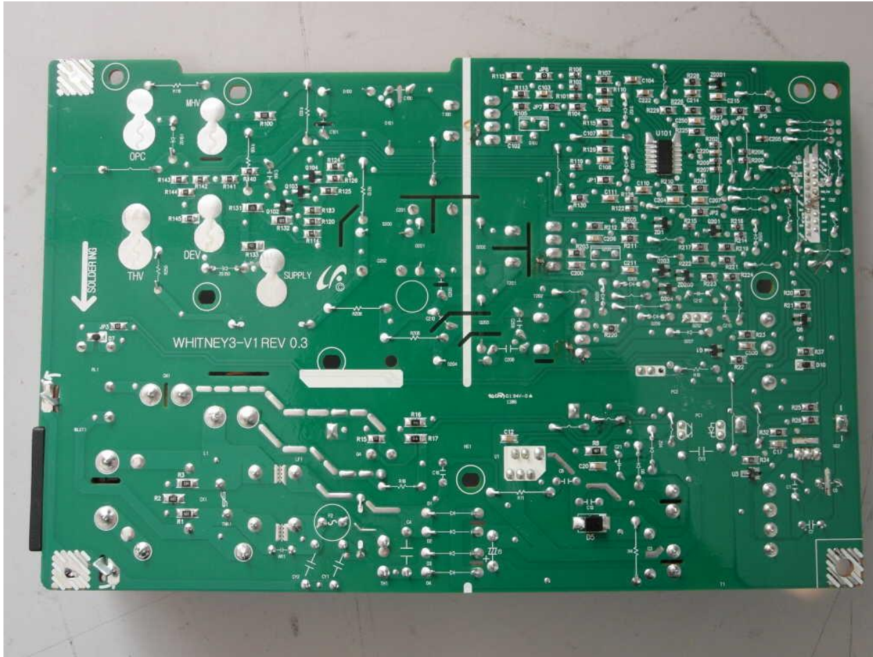
PBA Photo_SMPS+HVPS PBA Back (New Cowitel)
