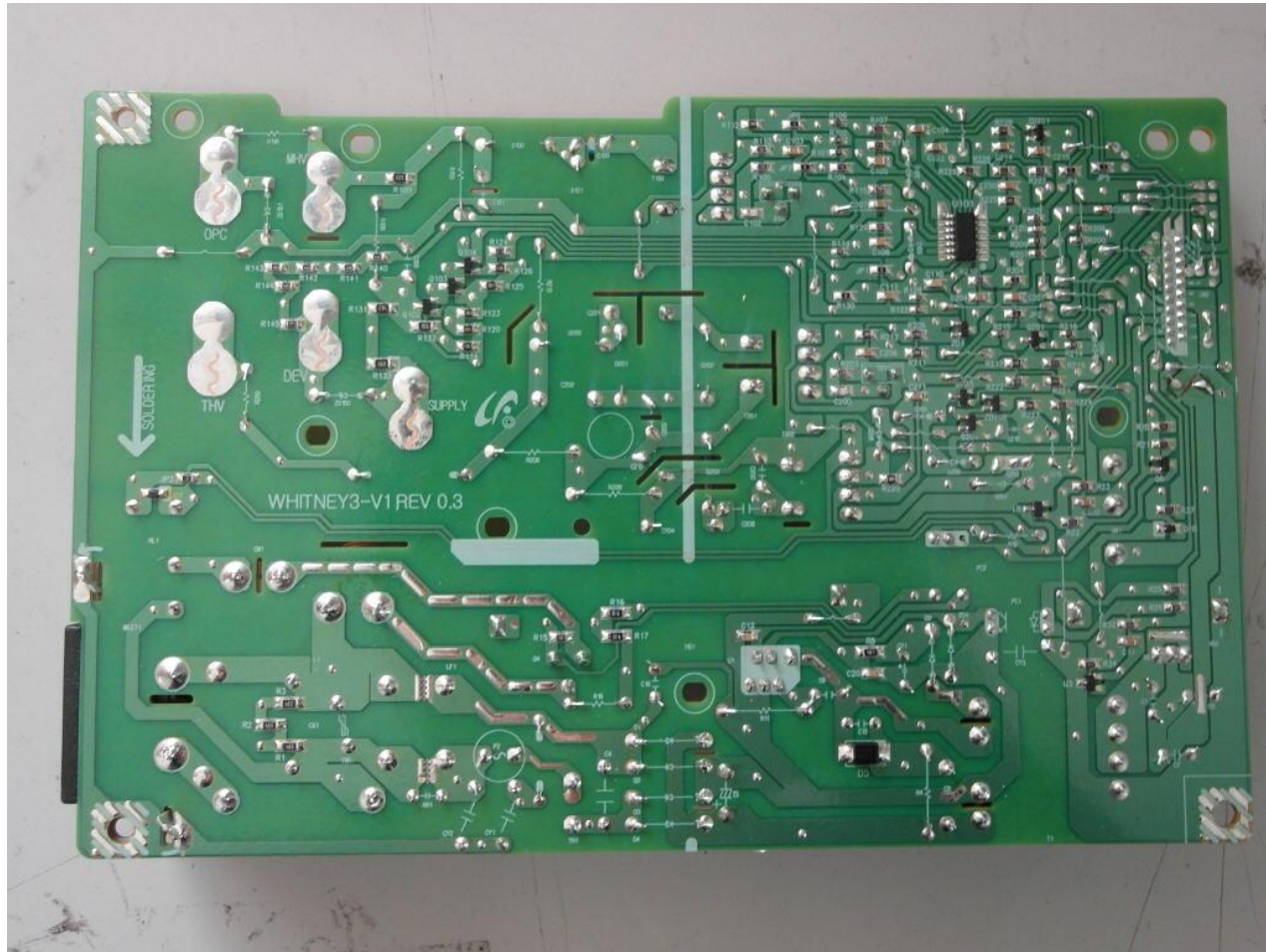
PBA Photo_SMPS+HVPS PBA Back (SUNG HO)
