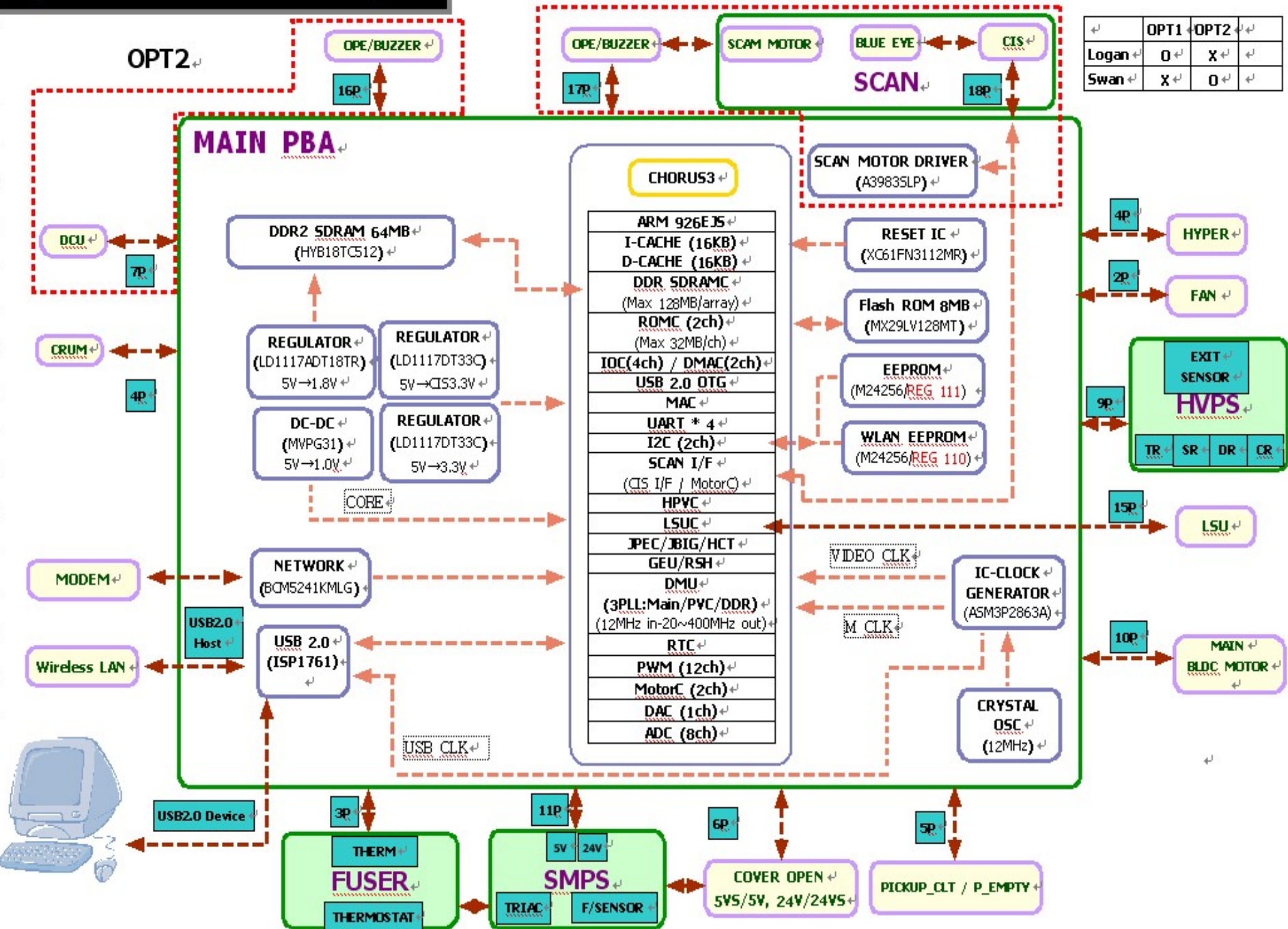
Logan/Swan_WLAN Block Diagram
