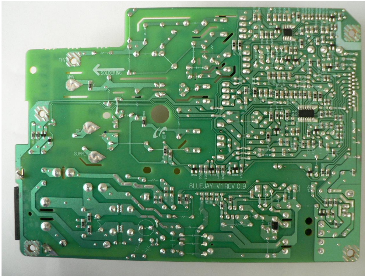
SUNGHO, Bluejay V1 SCX-3405W SMPS & HVPS PBA_Rear
