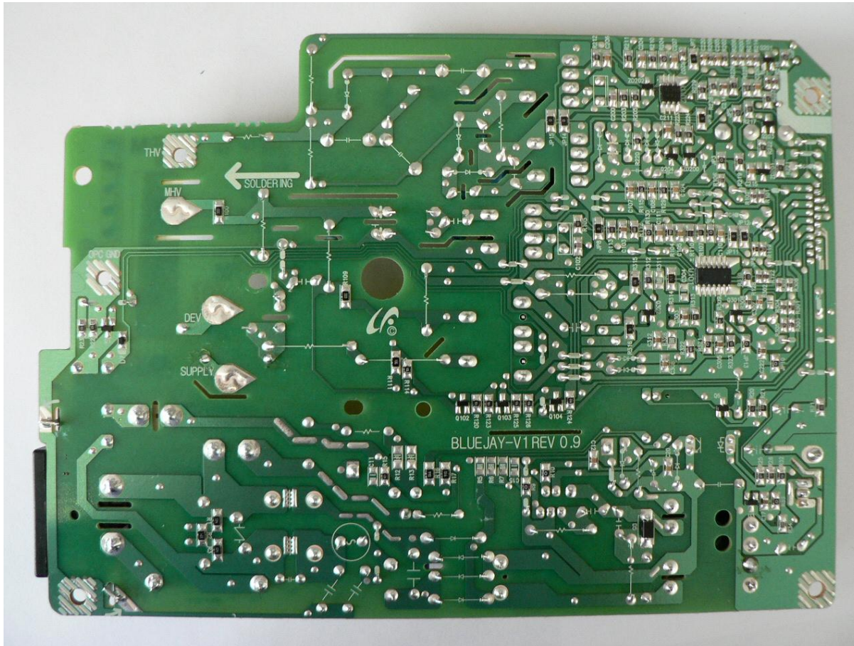
SHANDONG, Bluejay V1 SCX-3405W SMPS & HVPS PBA_Rear
