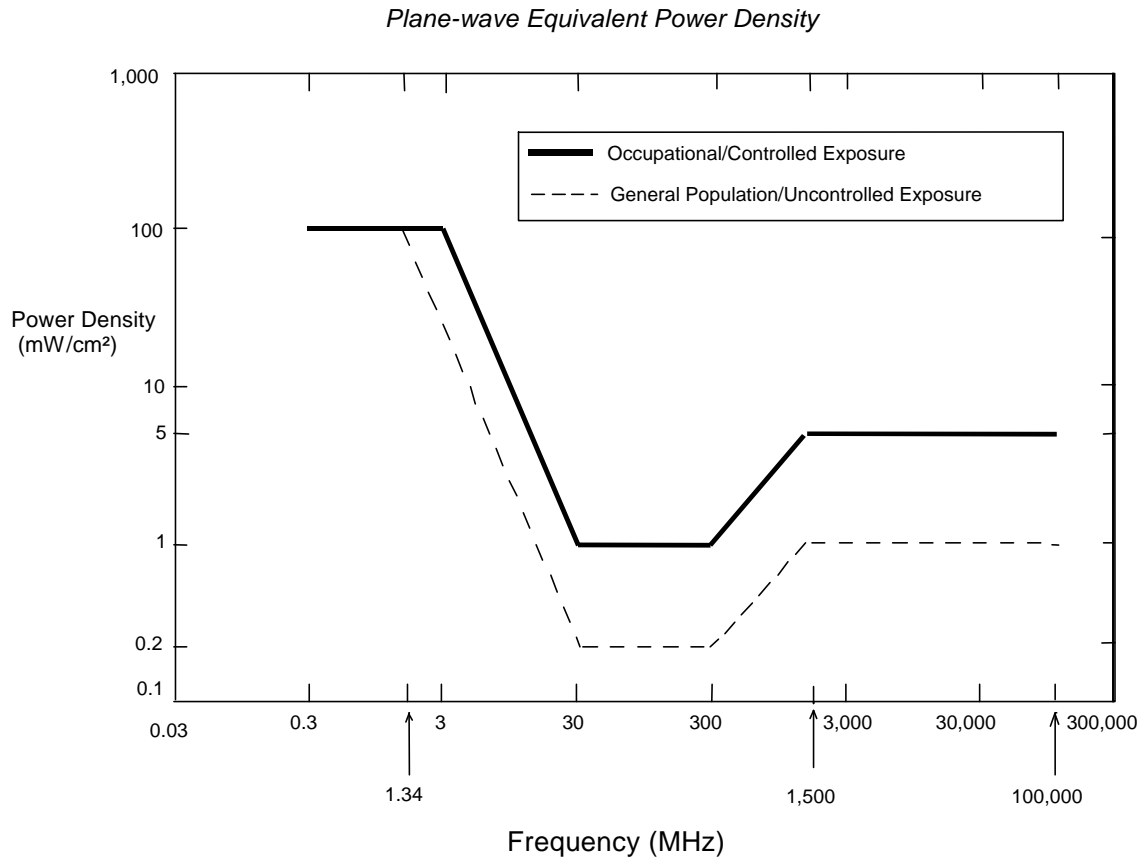
Figure 1. FCC Limits for Maximum Permissible Exposure (MPE)
