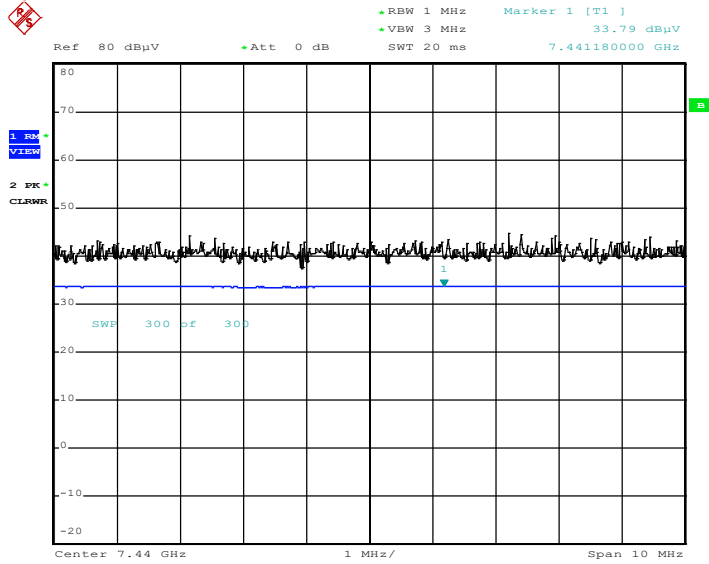
Radiated Spurious Emissions plot – Average Reading (Ch.39 3rd Harmonic_Y-H)
