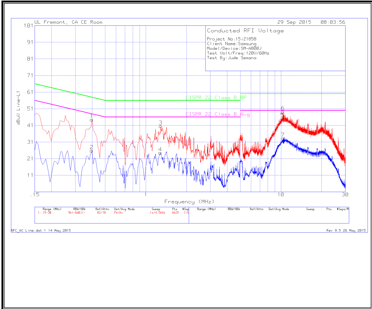
Range 1: Line-L1 .15 - 30MHz
