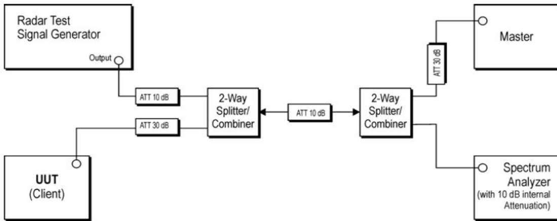
Figure 3-1. Conducted Test Setup for DFS
