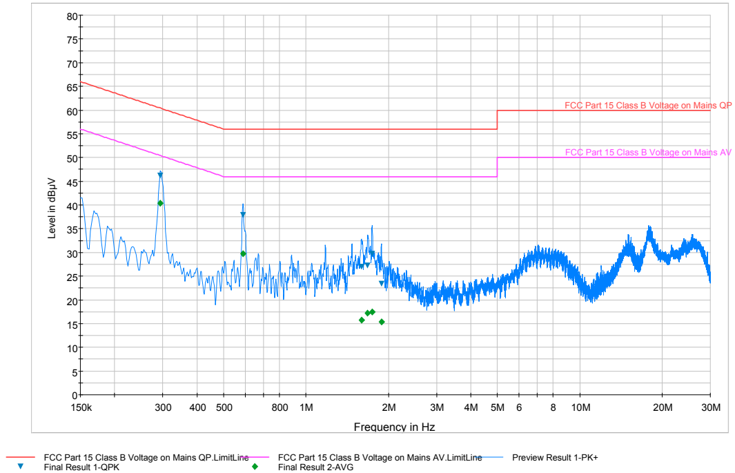
Plot 6-70. Line Conducted Plot with 802.11a (N)
