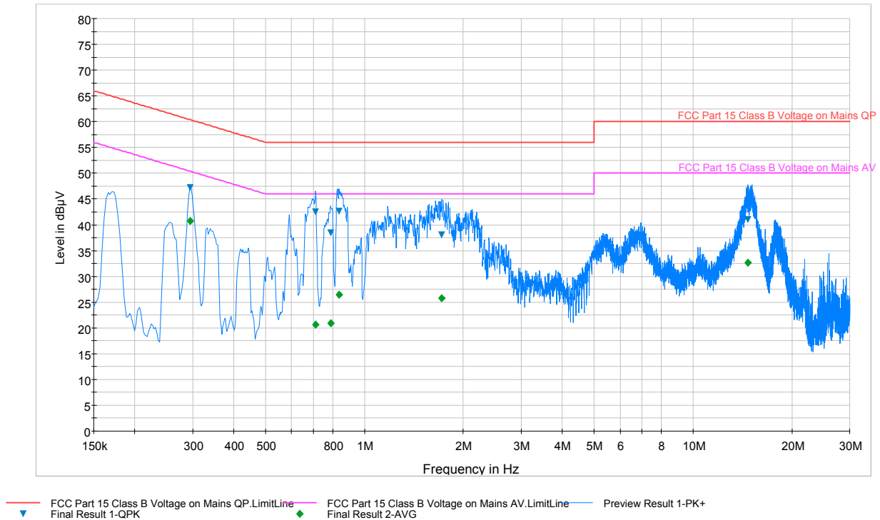
Plot 6-69. Line Conducted Plot with 802.11a (L1)
