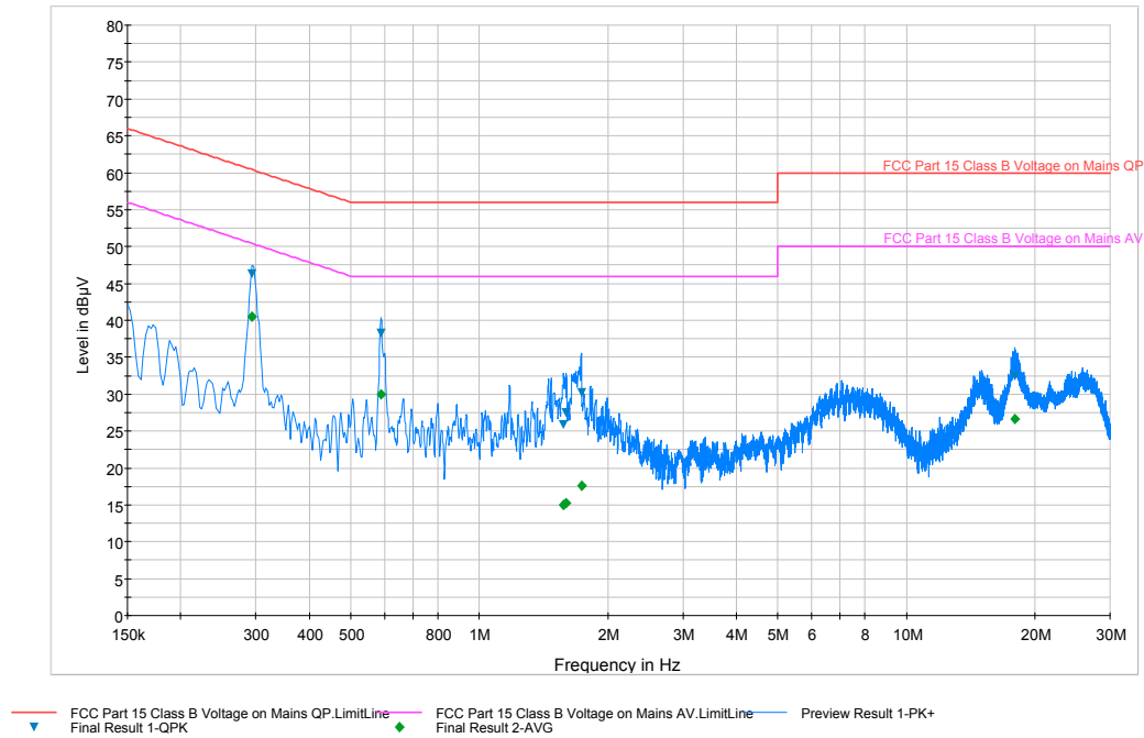
Plot 6-68. Line Conducted Plot with 802.11b (N)
