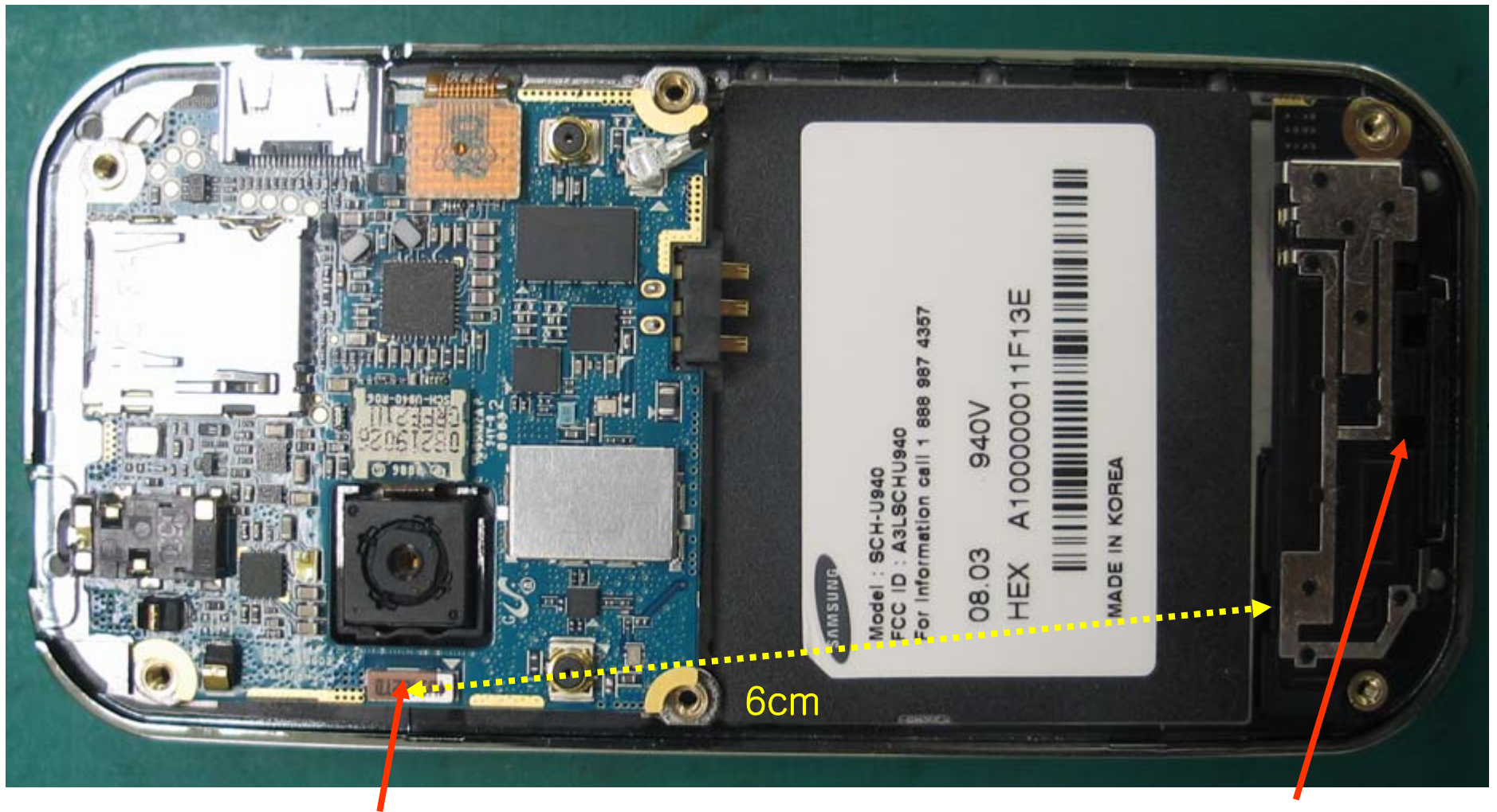
BT antenna
