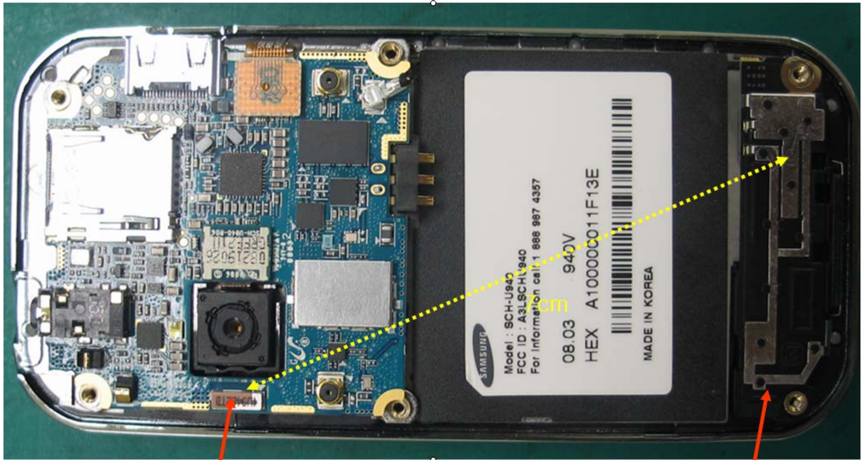
BT antenna
