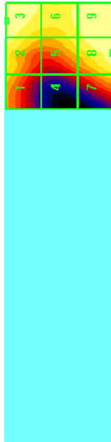
Figure 10-1 Sample E-field Scan Overlay (See Test Setup Photographs for actual WD overlay)
