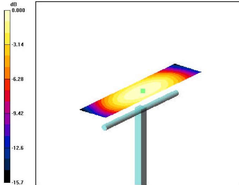
0 dB = 0.444A/m
