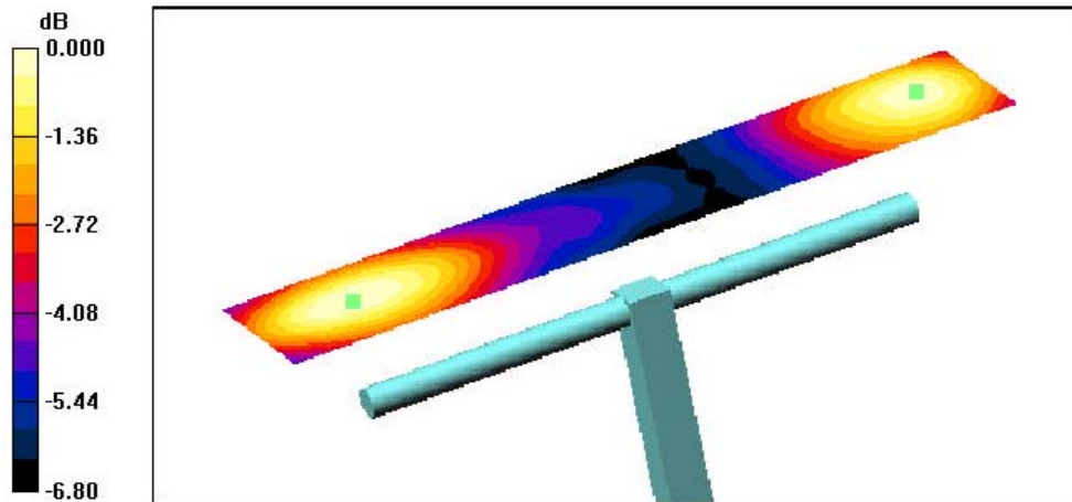
0 dB = 138.8V/m
