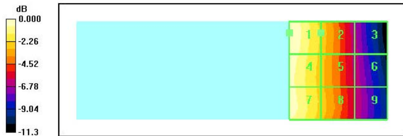
0 dB = 0.160A/m
