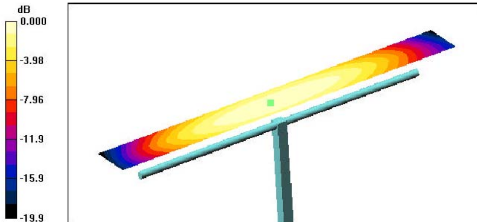
0 dB = 0.445A/m
