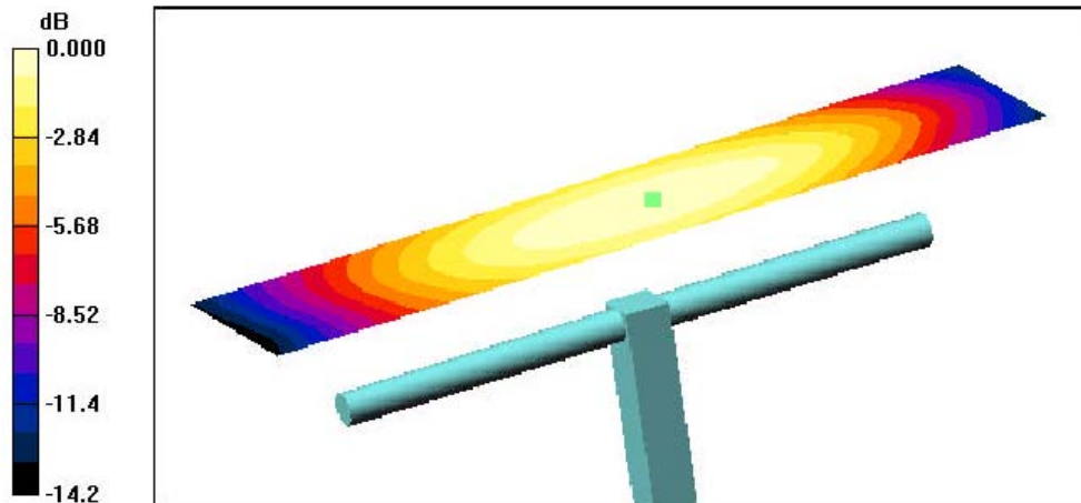
0 dB = 0.435A/m
