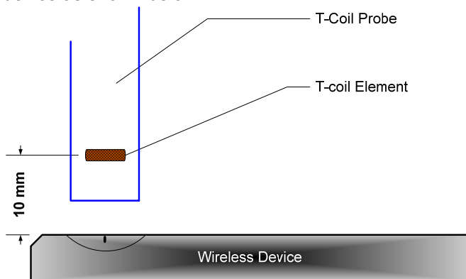
Figure 5-11 Measurement Distance
