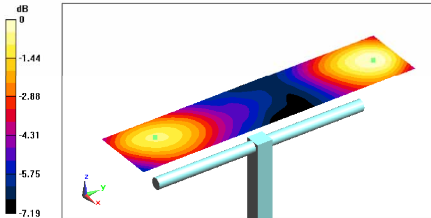
0 dB = 132.6V/m
