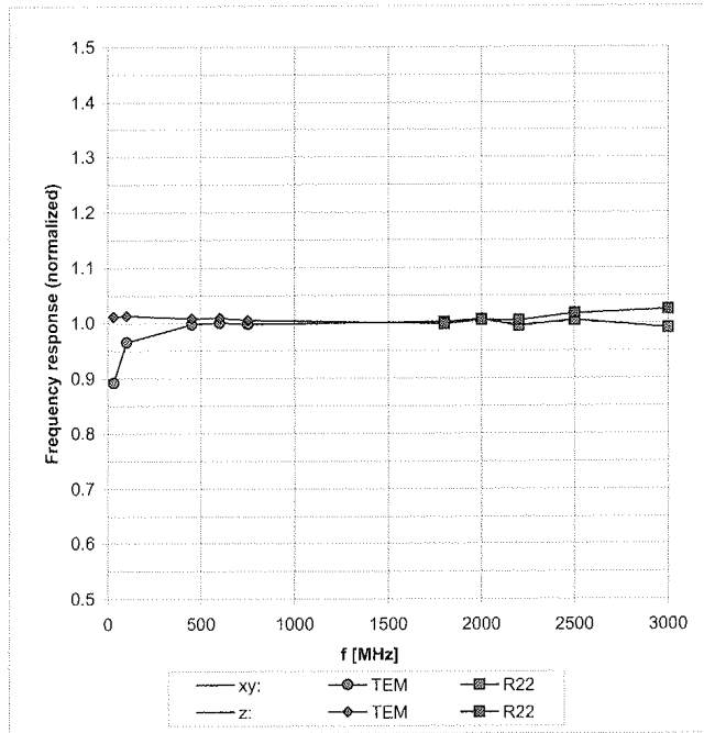
Uncertainty of Frequency Response of E-field: ± 6.3% (k=2)
