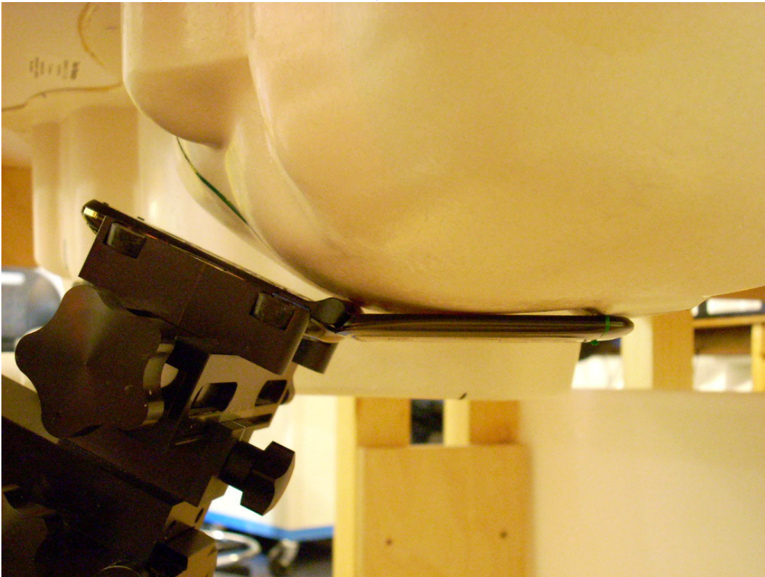
11. Mouth SAR, Touch Measurement, 2.6 cm
