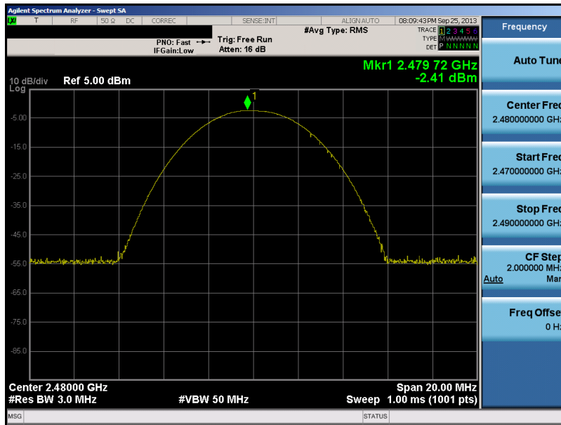
Plot 6-6 Peak Power Plot (2480MHz – High Channel)
