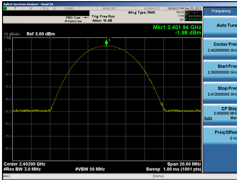
Plot 6-4. Peak Power Plot (2402MHz – Low Channel)
