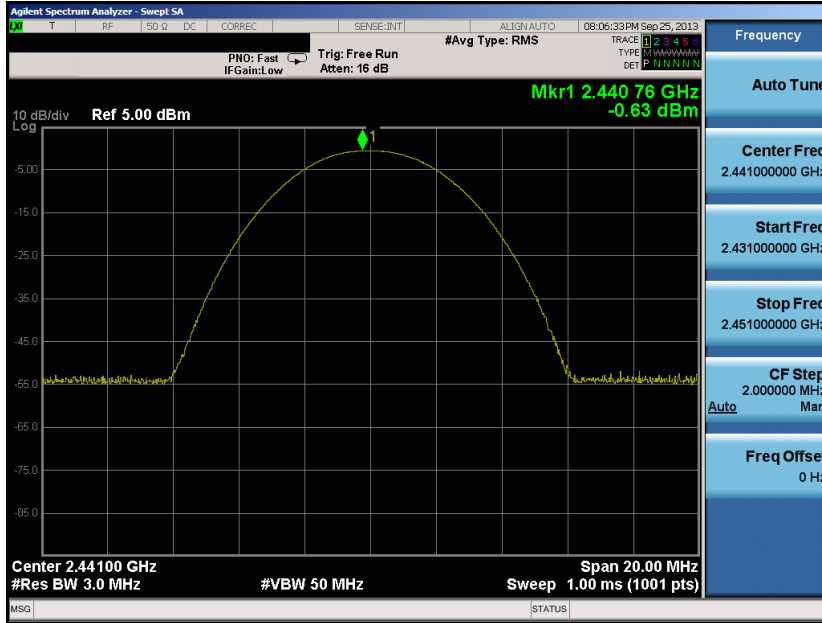
Plot 6-5 Peak Power Plot (2441MHz – Mid Channel)
