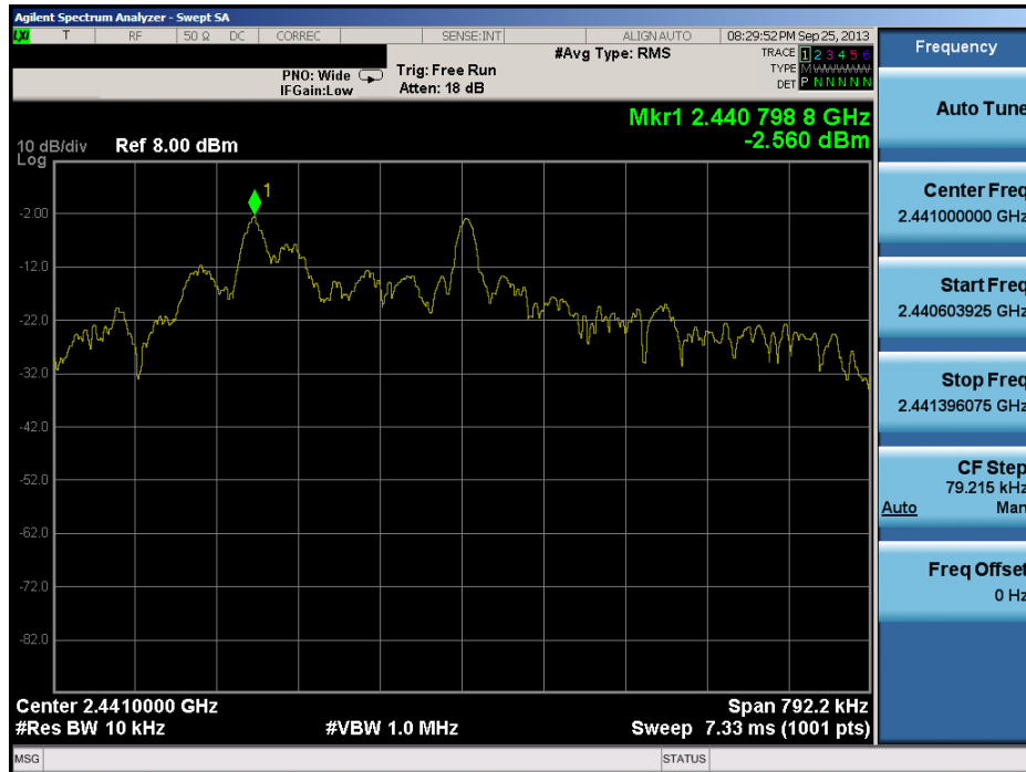
Plot 6-8. Power Spectral Density Plot (2441MHz – Mid Channel)
