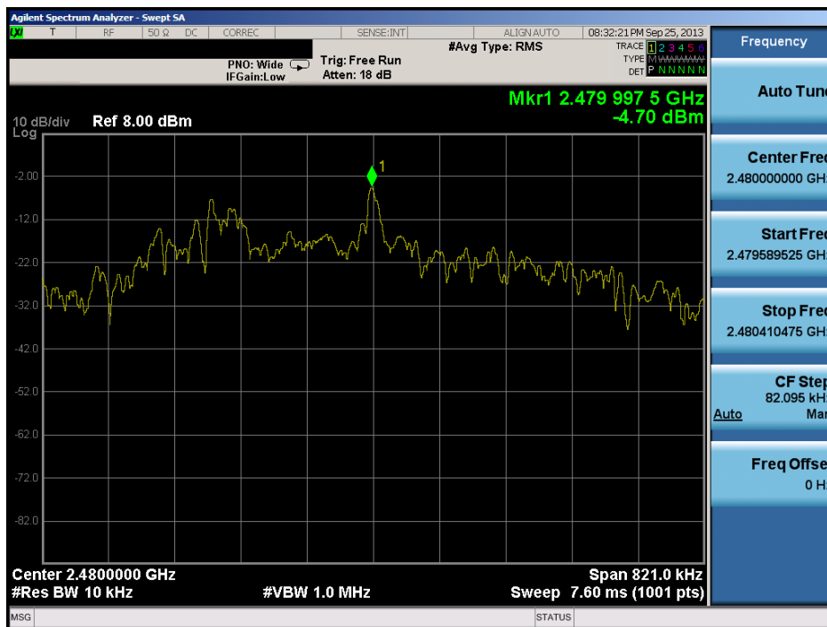
Plot 6-9. Power Spectral Density Plot (2480MHz – High Channel)
