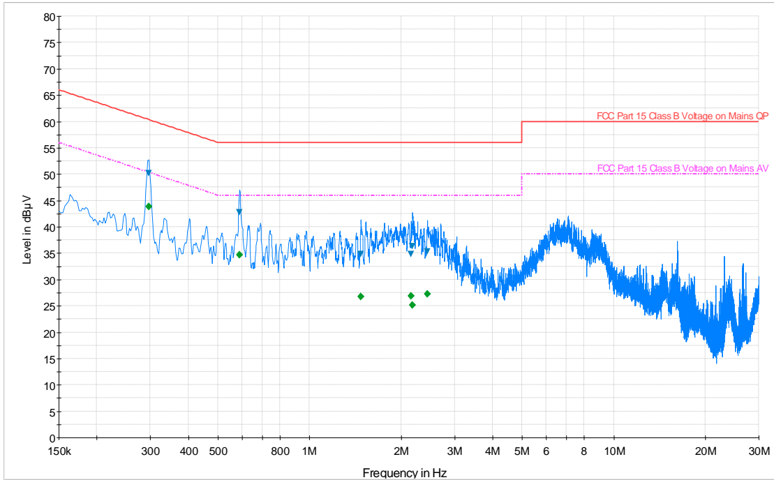
— FCC Part 15 Class B Voltage on Mains CP.LimitLine - - - FCC Part 15 Class B Voltage on Mains AV.LimitLine — Preview Result 1-PK+ ▼ Final Result 1-QPK ◆ Final Result 2-AVG
