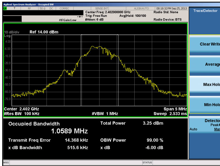
Plot 6-1. 6dB Bandwidth Plot (2402MHz – Low Channel)
