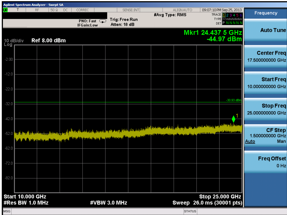
Plot 6-15. Conducted Spurious Plot (2441MHz – Mid Channel)
