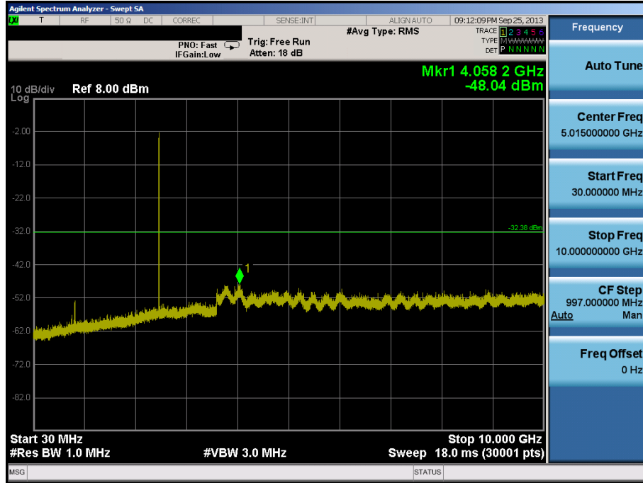
Plot 6-16. Conducted Spurious Plot (2480MHz – High Channel)
