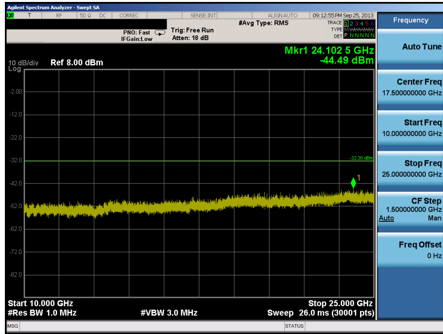
Plot 6-17. Conducted Spurious Plot (2480MHz – High Channel)
