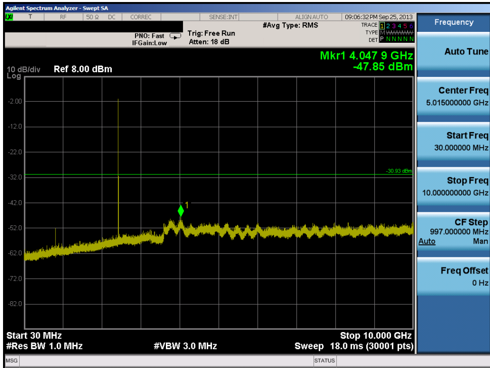
Plot 6-14. Conducted Spurious Plot (2441MHz – Mid Channel)
