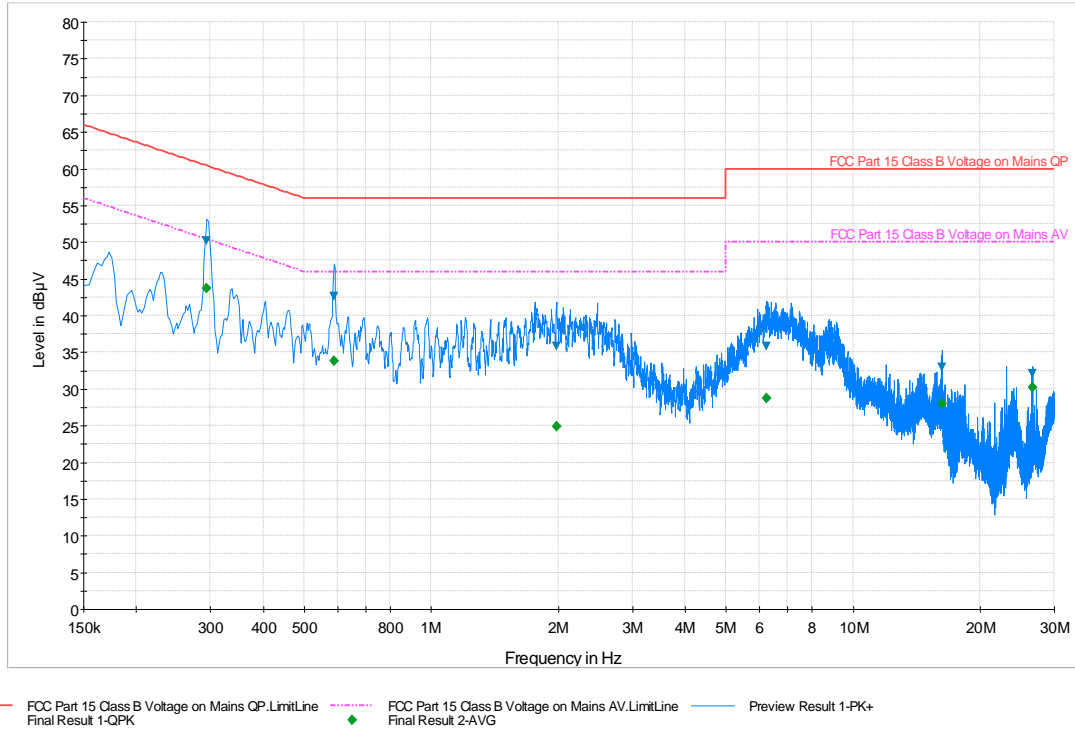
Plot 6-20. Line Conducted Plot with ANT+ (L1)
