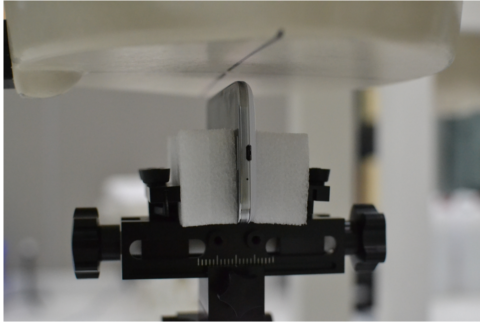
SAR Test Setup Photo 5: Right Edge at 1.0 cm with Wireless Charging Cover
