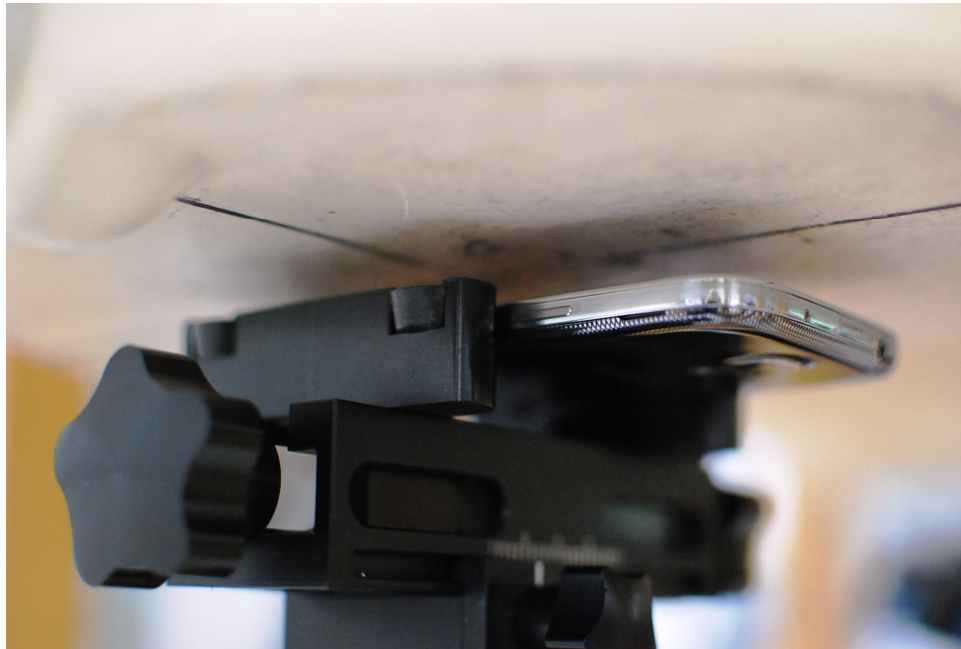
SAR Test Setup Photo 2: Front Side at 1.0 cm with Standard Battery Cover
