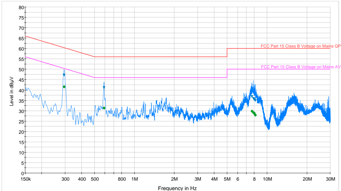
Plot 6-102. Line Conducted Plot with 802.11a UNII Band 1 (N)
