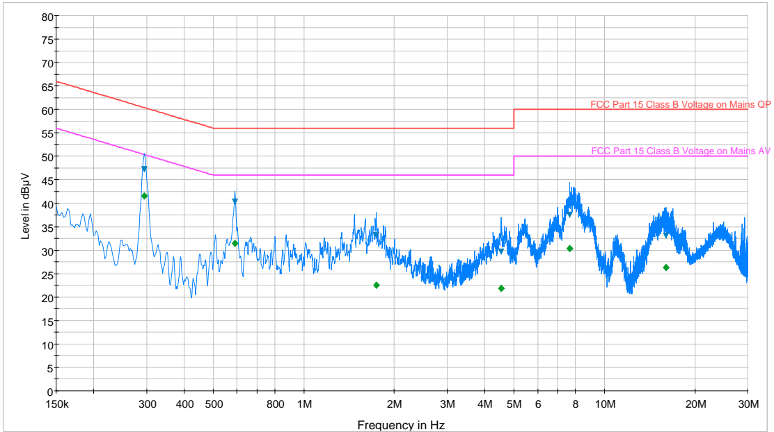
Plot 6-101. Line Conducted Plot with 802.11a UNII Band 1 (L1)
