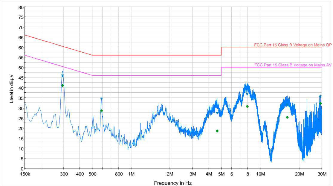
Plot 6-105. Line Conducted Plot with 802.11a UNII Band 3 (L1)
