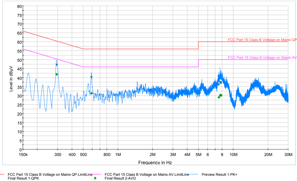
Plot 6-72. Line Conducted Plot with 802.11b (N)
