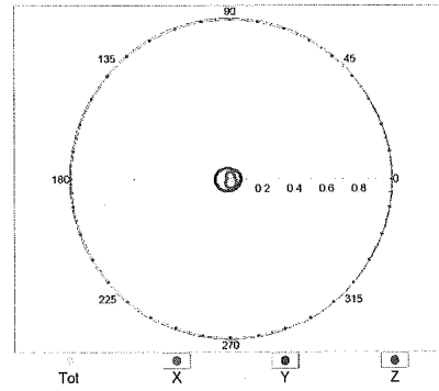
f=2500 MHz,R22,90°
