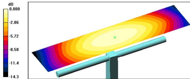
0 dB = 0.465A/m
