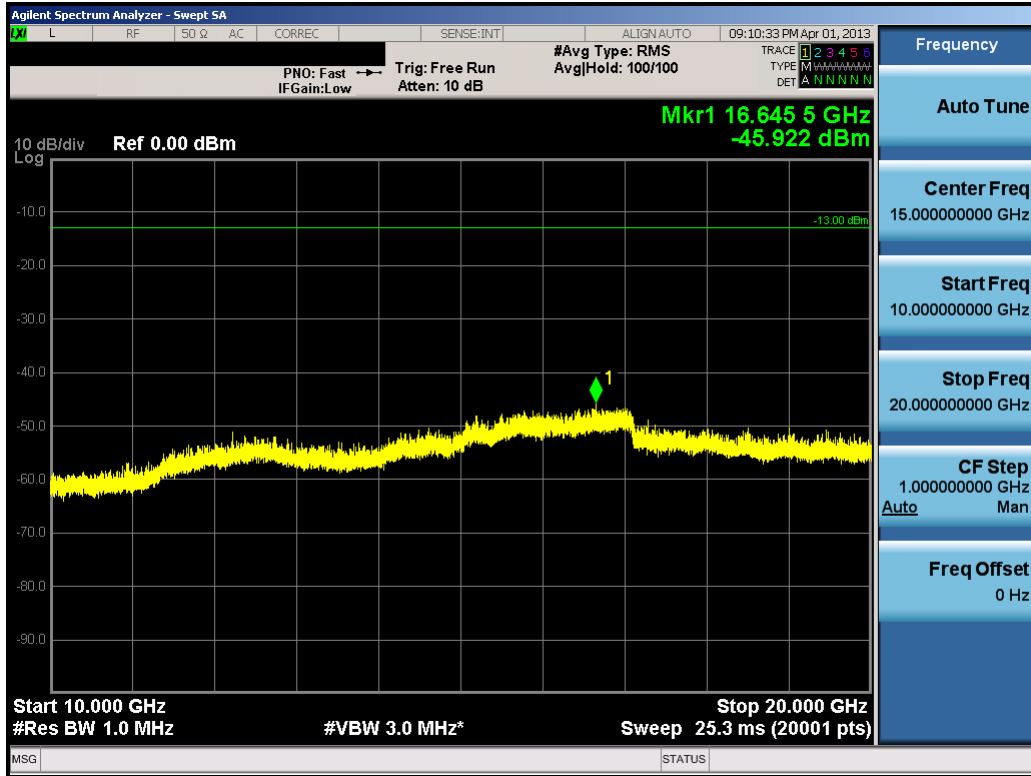
Plot 7-24. Conducted Spurious Plot (10.0MHz QPSK – RB Size 1, RB Offset 0 – High Channel)
