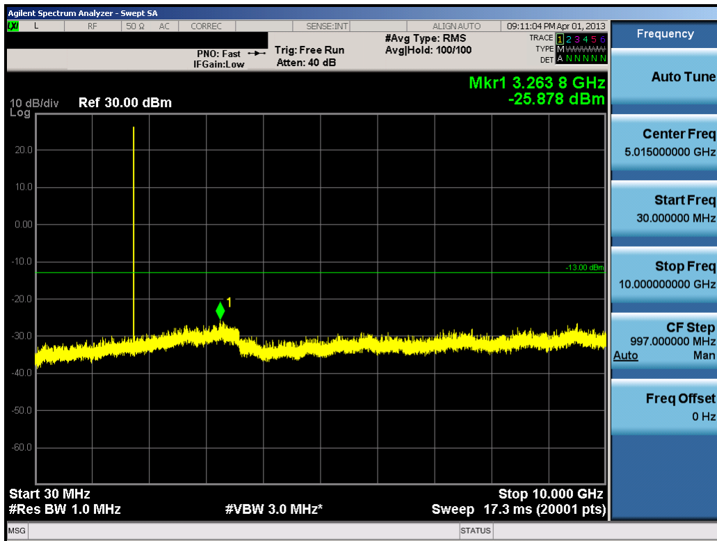
Plot 7-23. Conducted Spurious Plot (10.0MHz QPSK – RB Size 1, RB Offset 0 – High Channel)
