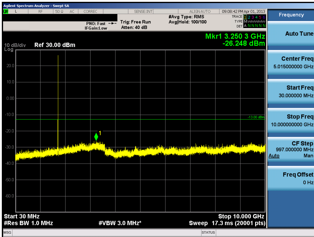
Plot 7-21. Conducted Spurious Plot (10.0MHz QPSK – RB Size 1, RB Offset 0 – Mid Channel)
