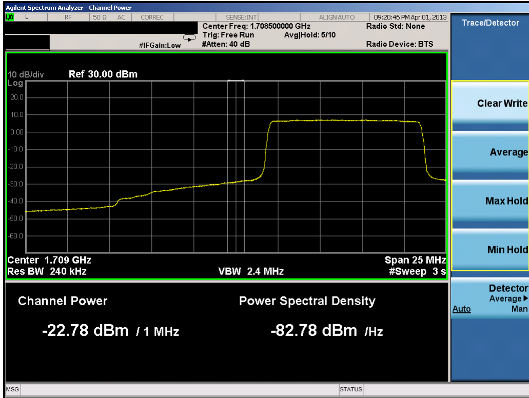
Plot 7-16. Lower Extended Band Edge Plot (10.0MHz QPSK – RB Size 50)
