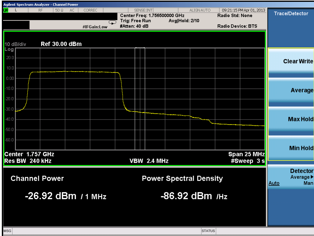
Plot 7-26. Upper Extended Band Edge Plot (10.0MHz QPSK – RB Size 50)
