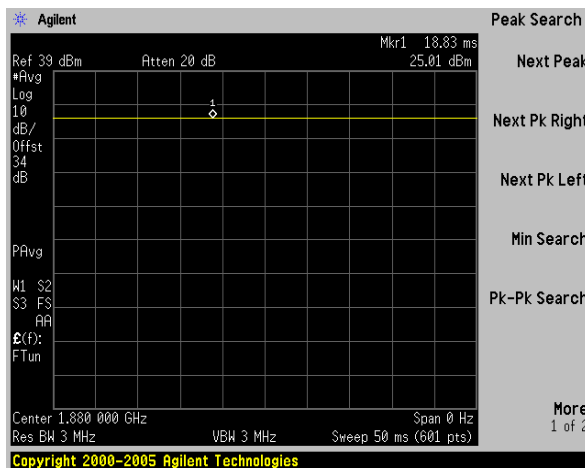
Figure 8.3 CW Signal
