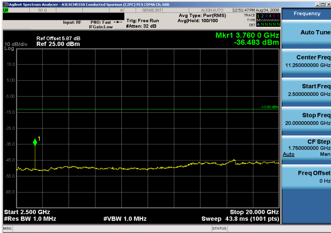
Plot 6-17. Conducted Spurious Plot (PCS CDMA Mode – Ch. 600)
