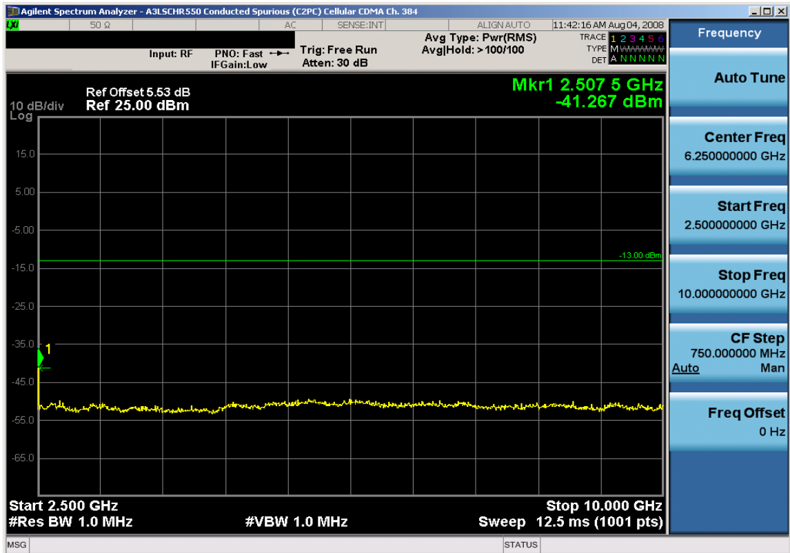
Plot 6-6. Conducted Spurious Plot (Cellular CDMA Mode – Ch. 384)
