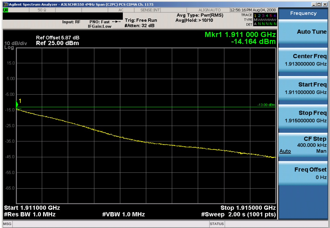
Plot 6-23. 4MHz Span Plot (PCS CDMA Mode – Ch. 1175)
