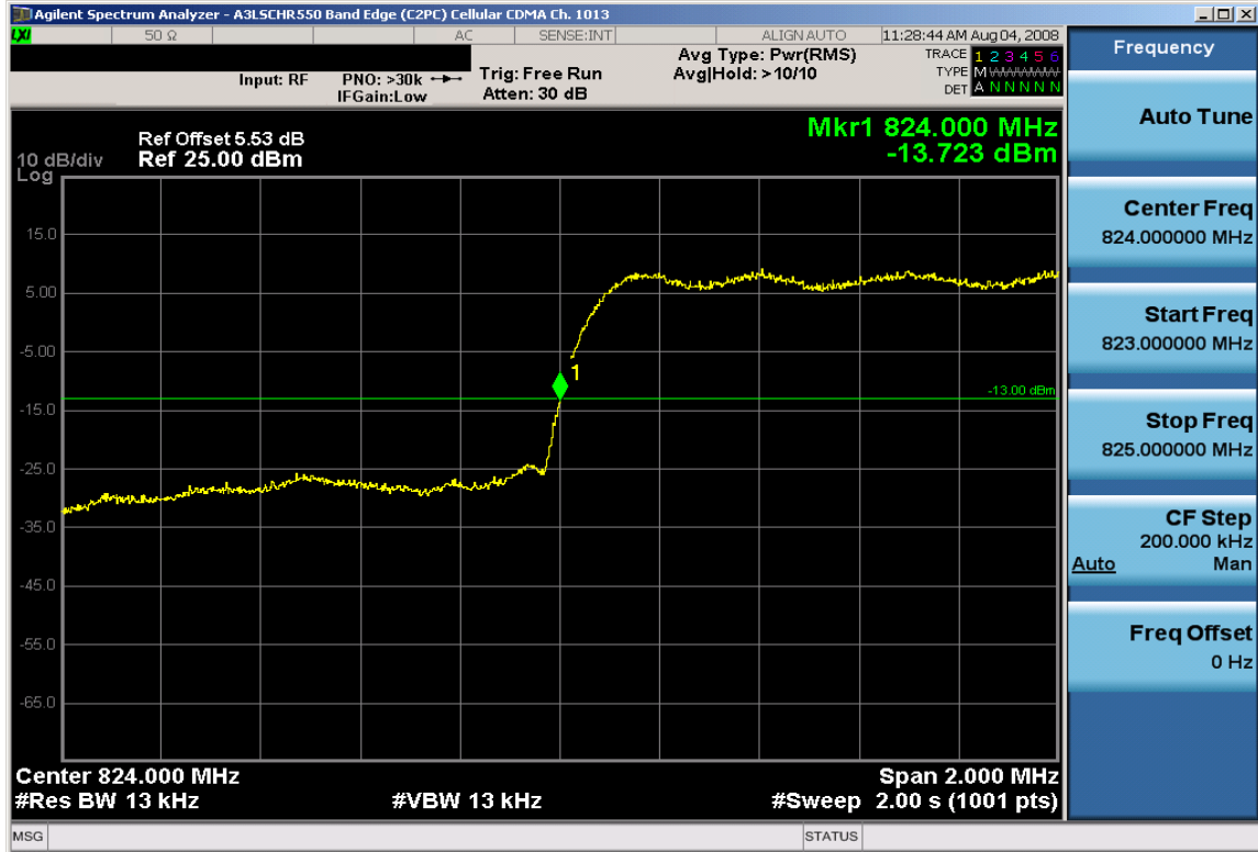
Plot 6-3. Band Edge Plot (Cellular CDMA Mode – Ch. 1013)
