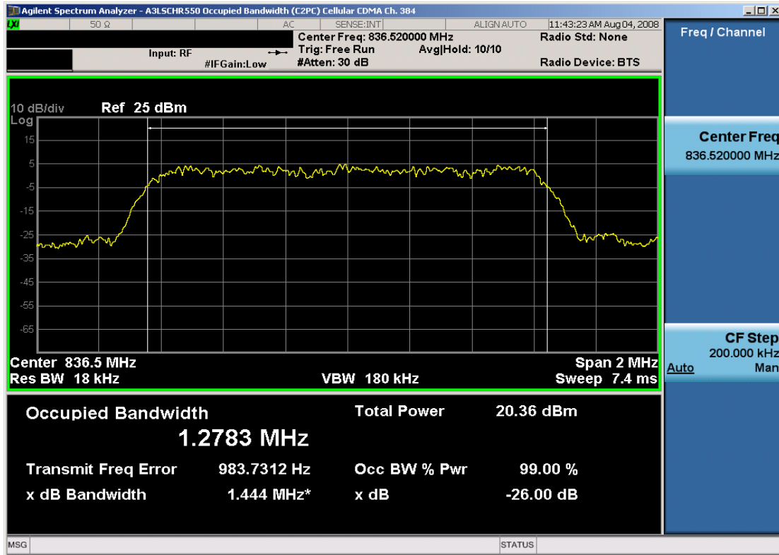
Plot 6-7. Occupied Bandwidth Plot (Cellular CDMA Mode – Ch. 384)
