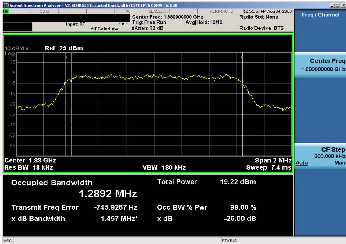
Plot 6-18. Occupied Bandwidth Plot (PCS CDMA Mode – Ch. 600)
