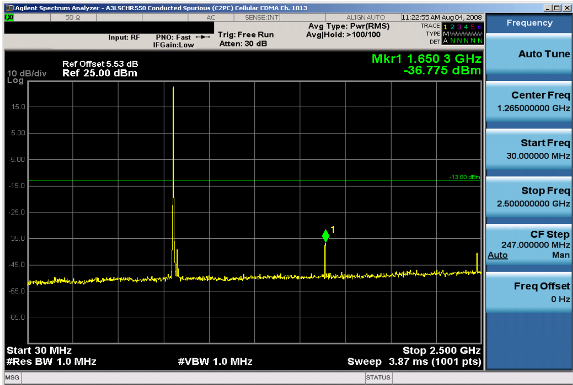
Plot 6-1. Conducted Spurious Plot (Cellular CDMA Mode – Ch. 1013)
