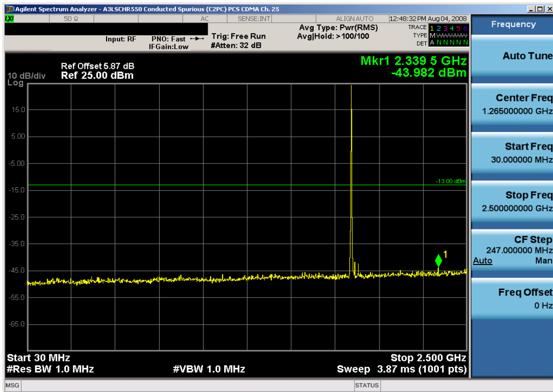
Plot 6-12. Conducted Spurious Plot (PCS CDMA Mode – Ch. 25)
