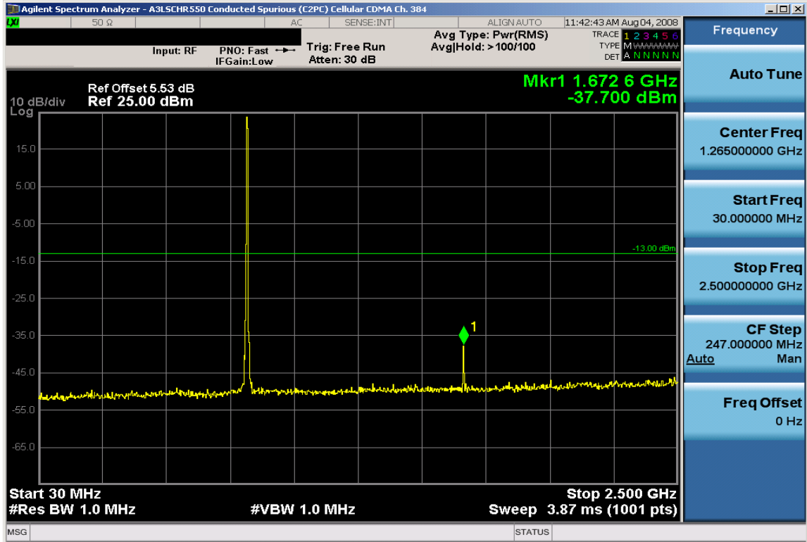
Plot 6-5. Conducted Spurious Plot (Cellular CDMA Mode – Ch. 384)
