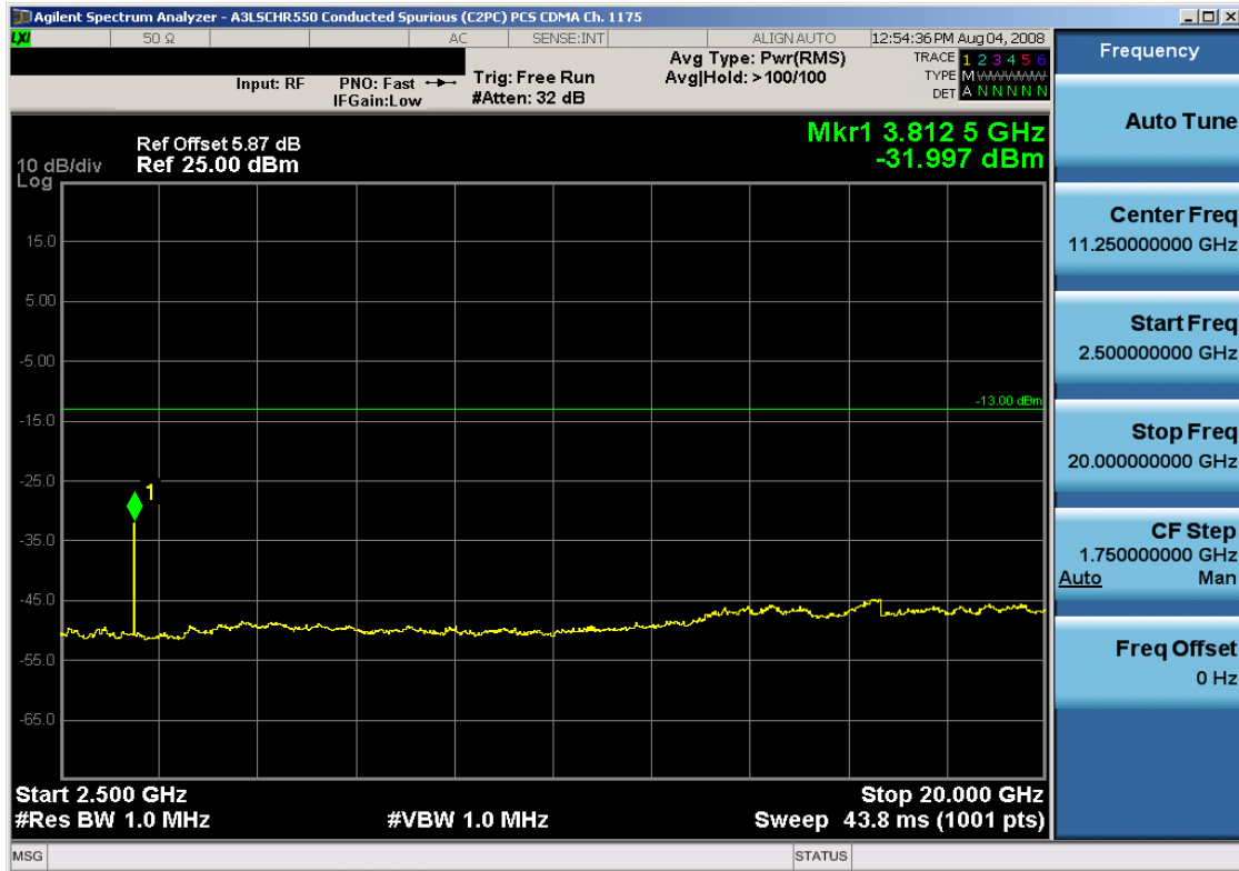
Plot 6-21. Conducted Spurious Plot (PCS CDMA Mode – Ch. 1175)
