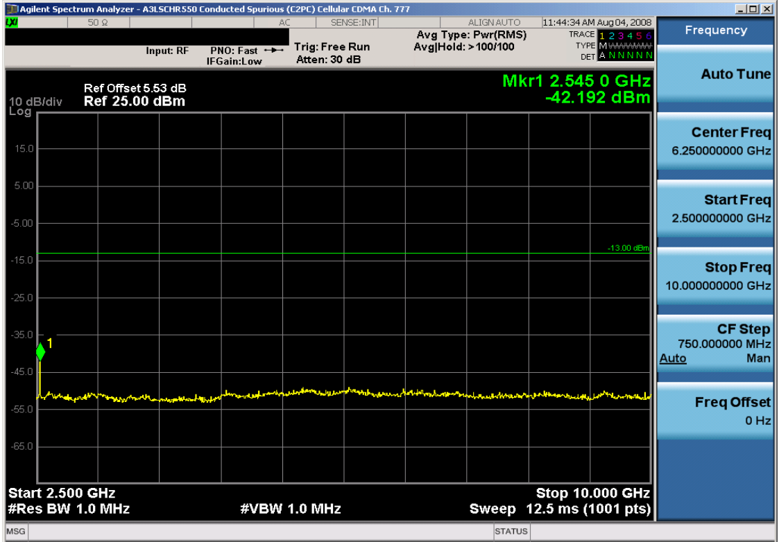
Plot 6-9. Conducted Spurious Plot (Cellular CDMA Mode – Ch. 777)
