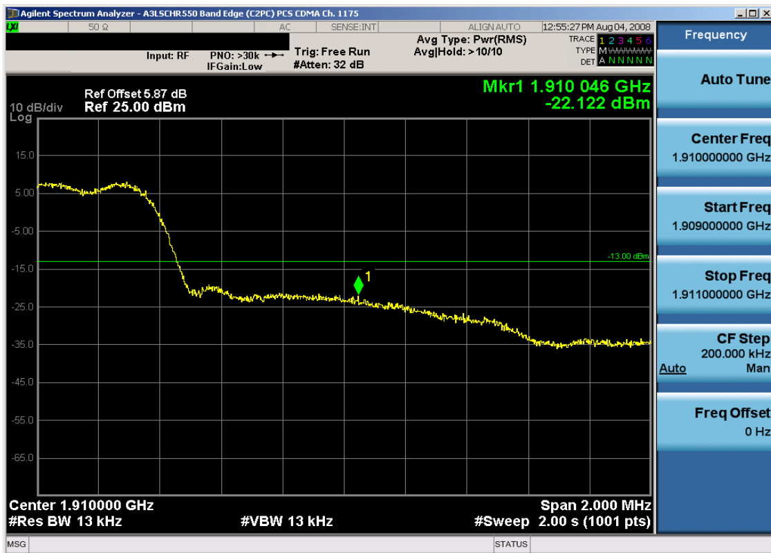
Plot 6-22. Band Edge Plot (PCS CDMA Mode – Ch. 1175)
