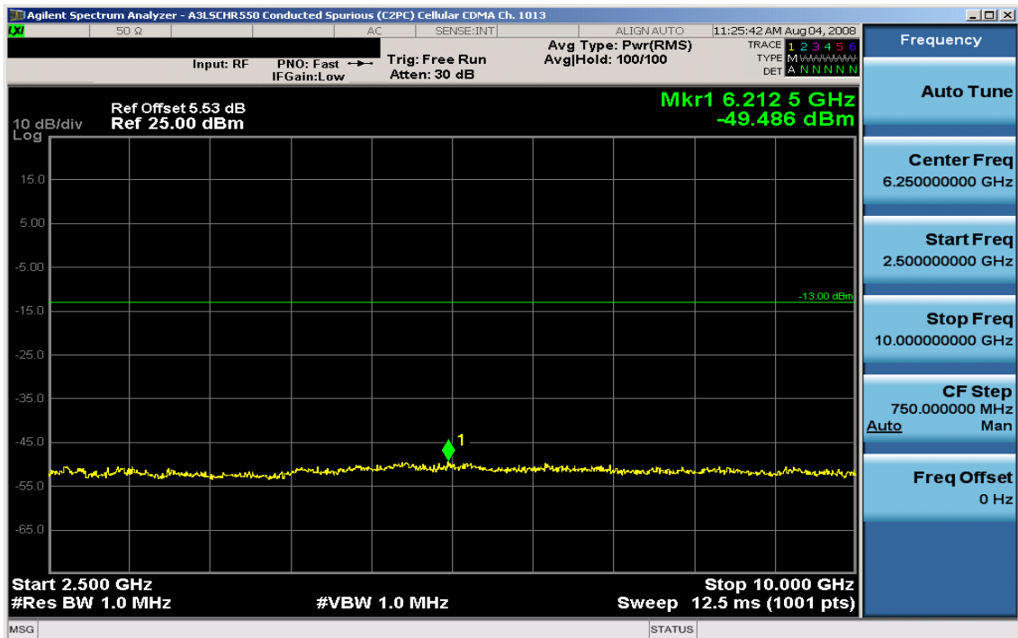
Plot 6-2. Conducted Spurious Plot (Cellular CDMA Mode – Ch. 1013)
