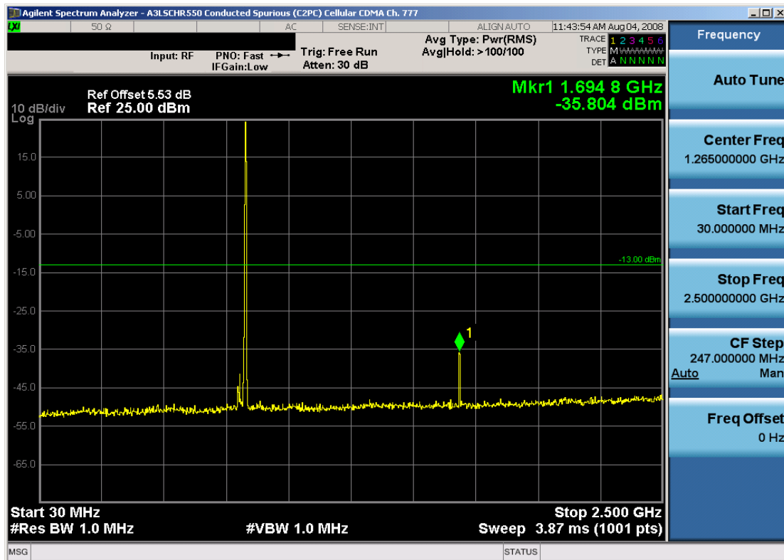
Plot 6-8. Conducted Spurious Plot (Cellular CDMA Mode – Ch. 777)
