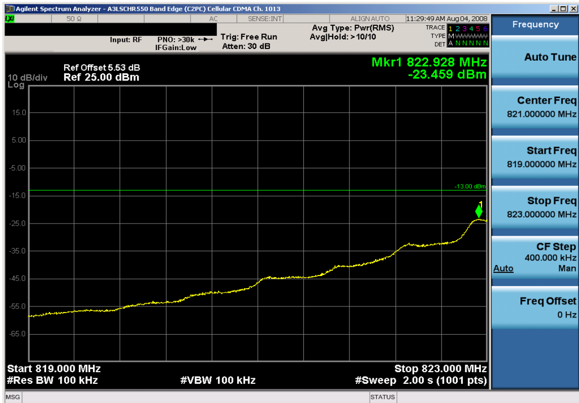
Plot 6-4. 4MHz Span Plot (Cellular CDMA Mode – Ch. 1013)
