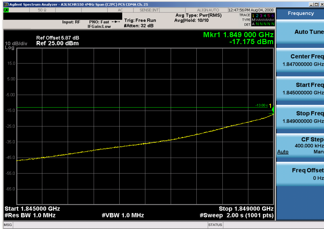
Plot 6-15. 4MHz Span Plot (PCS CDMA Mode – Ch. 25)
