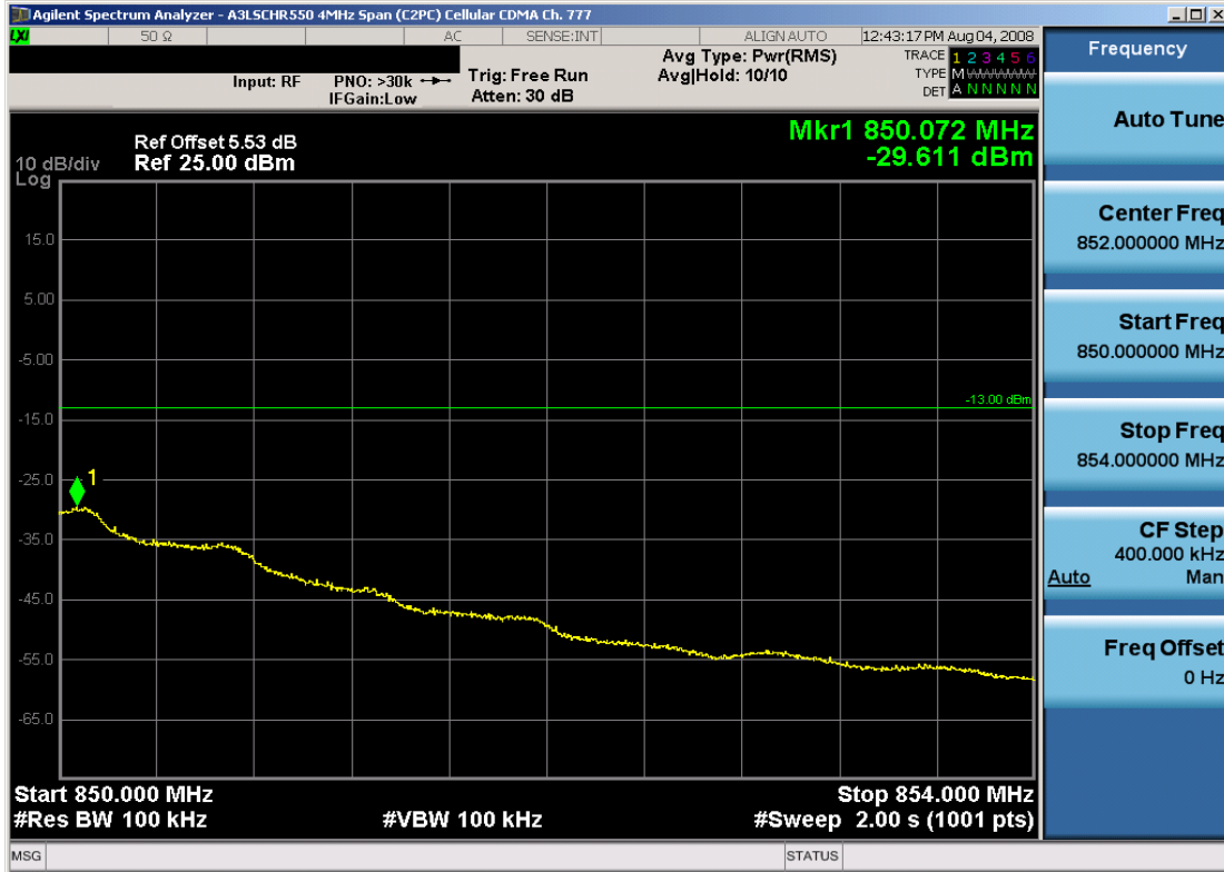
Plot 6-11. 4MHz Span Plot (Cellular CDMA Mode – Ch. 777)
