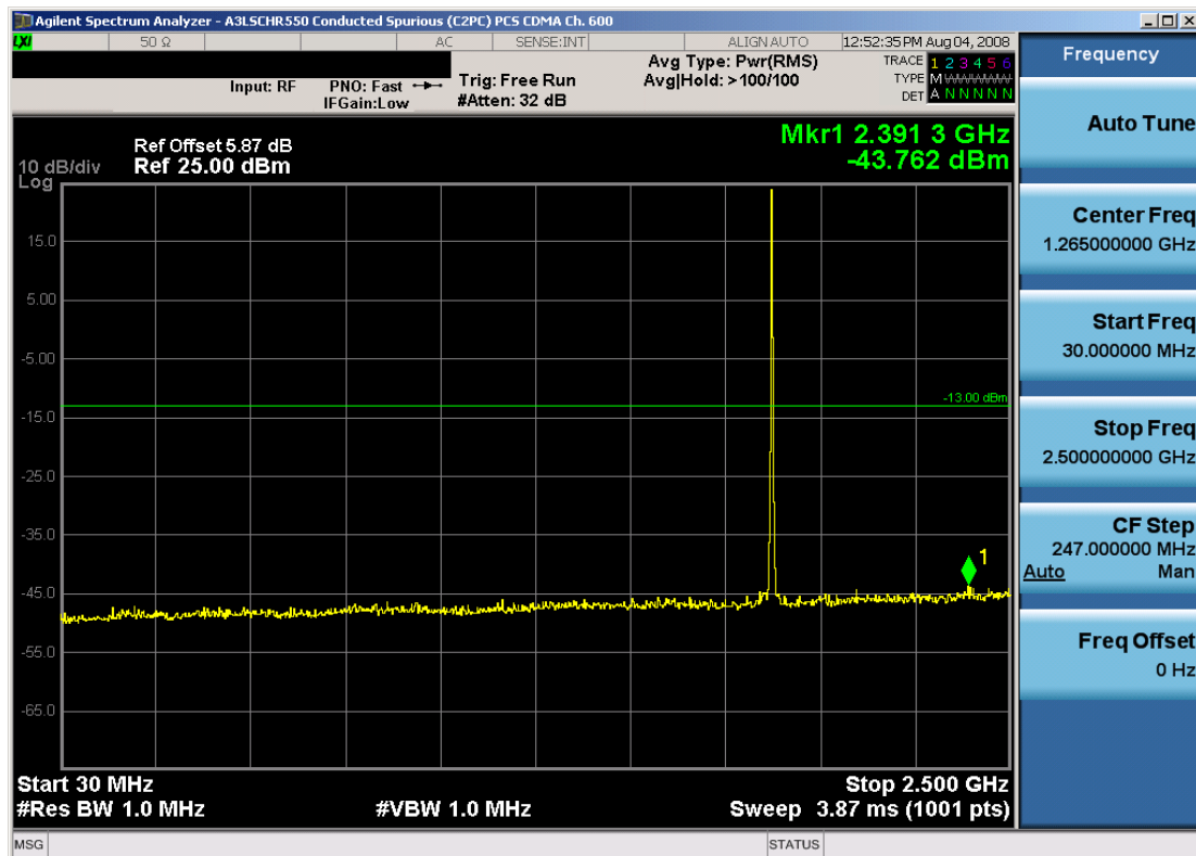
Plot 6-16. Conducted Spurious Plot (PCS CDMA Mode – Ch. 600)
