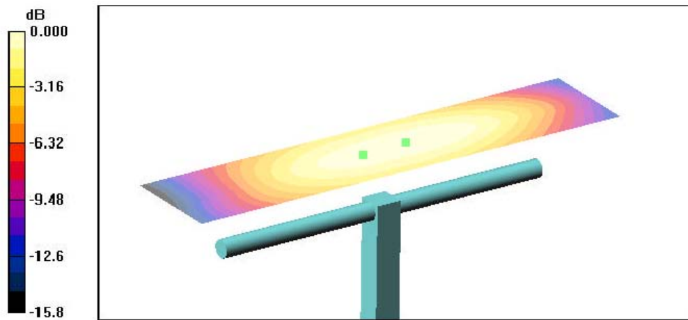
0 dB = 0.433A/m
