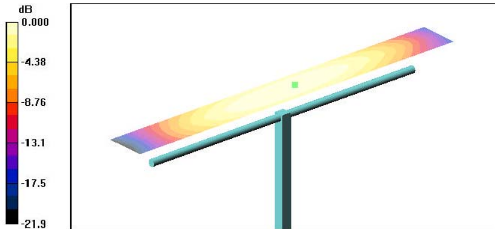
0 dB = 0.437 A/m
