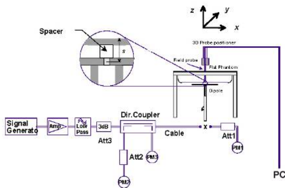
Figure 9-1 System Verification Setup Diagram
