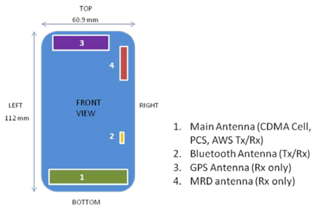
Figure 1-1 DUT Antenna Locations
