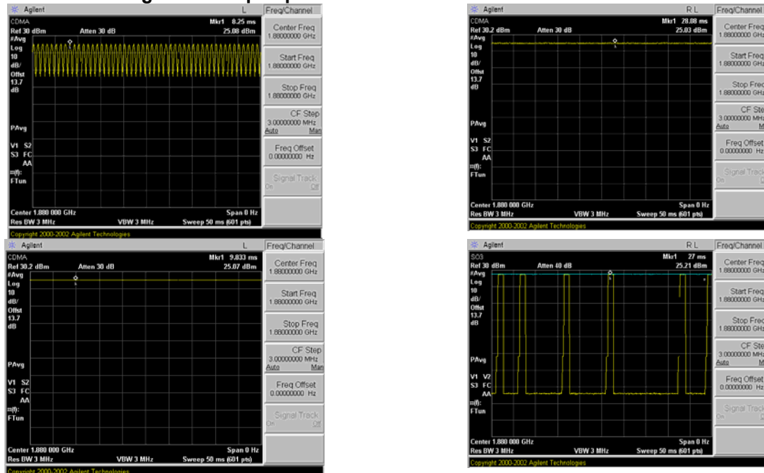
Figure 8-4 Zero-Span Plots
