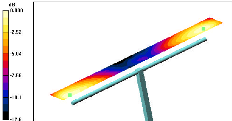
0 dB = 163.5V/m
