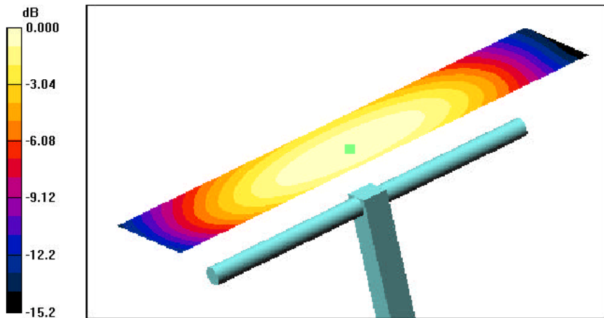
0 dB = 0.446A/m
